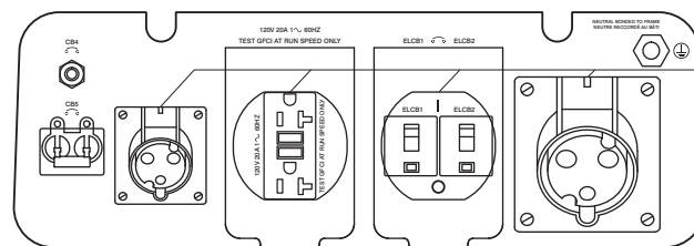
International Model Receptacles
