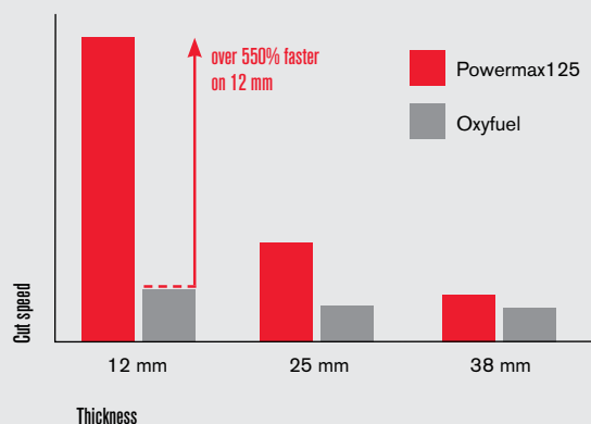
Relative cut performance on mild steel
