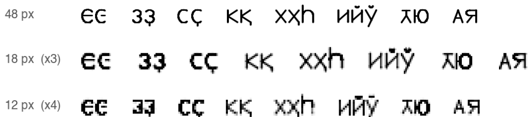
Figure 16: Confusable pairs at reading sizes, FreeType rendering: е/е, з/з, с/с, к/к, х/х, и/й, л/ю, а/я. The 18 and 12 pixel rows are nearest-neighbor magnifications of the actual rasters — what the renderer produced, not what the vector promises.
