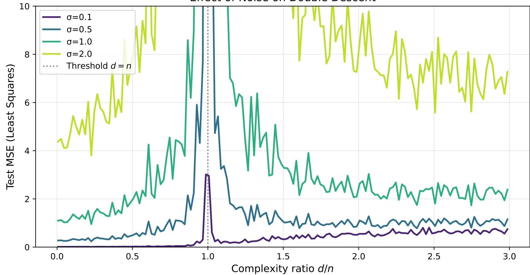
Effect of Noise on Double Descent
