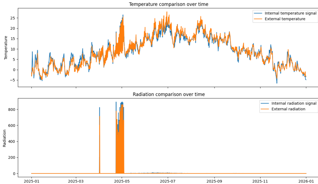
Fig. 6. Comparison of site-level outside-temperature signal, radiation proxy and external weather context
