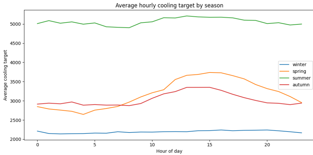
Fig. 8. Average hourly cooling-demand profile by season
