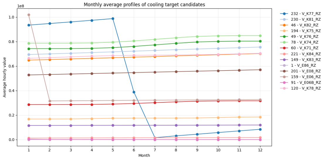
Fig. 4. Monthly average profiles of shortlisted cooling-target candidates
