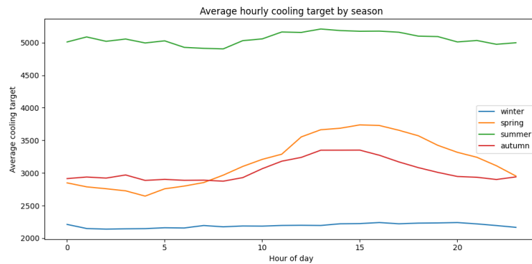
Fig. 8. Average hourly cooling-demand profile by season
