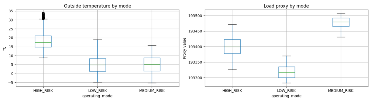
Fig. 14. Operating-mode differences in outside temperature and load proxy
