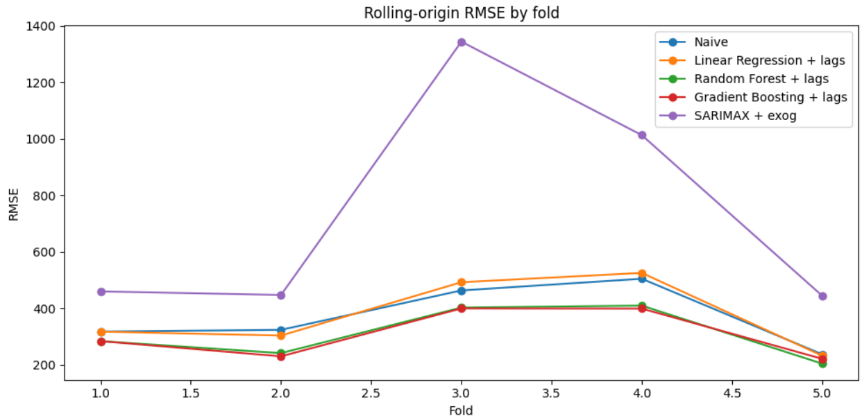
Fig. 12. Rolling-origin RMSE by fold for the main benchmark candidates
