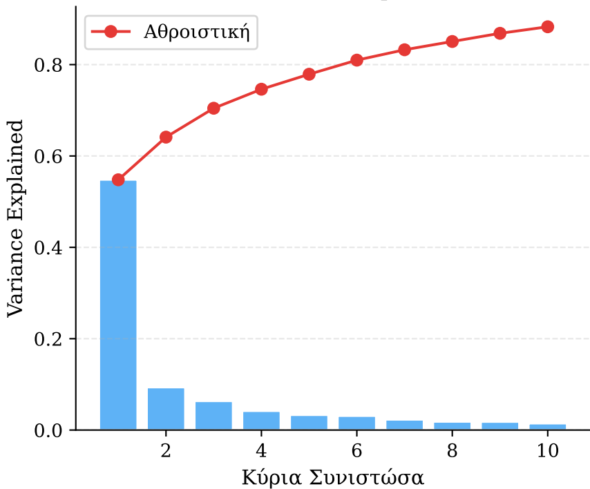
PCA scree (top 10)
