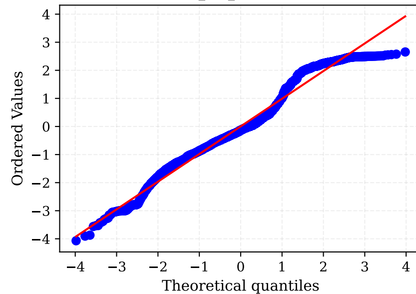
total_acc_z (Q-Q plot)
