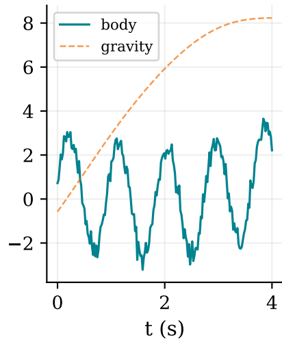
(2) Butterworth (fc=0.3 Hz, n=3)
