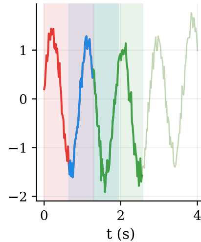
(4) Sliding Window (W=128, 50% overlap)
