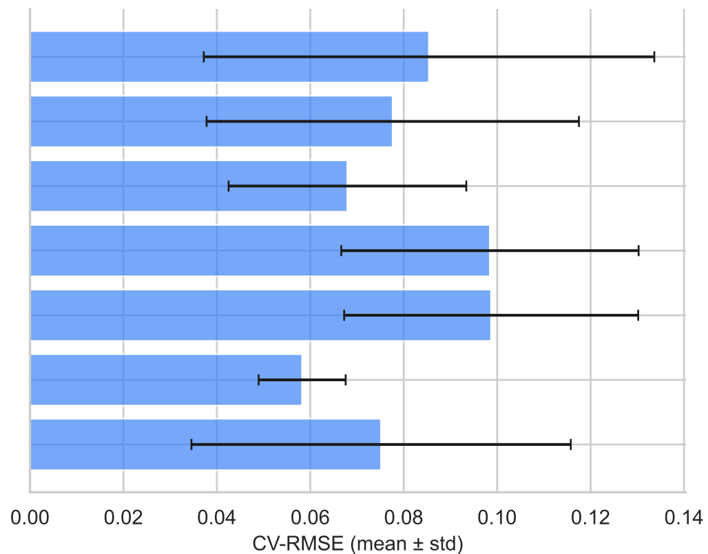
Flood-It! 2
