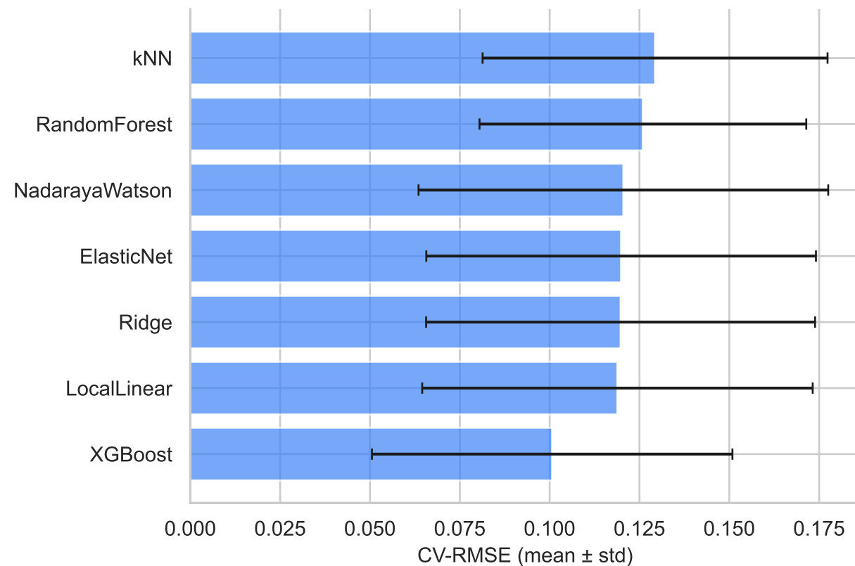
Flood-It!
