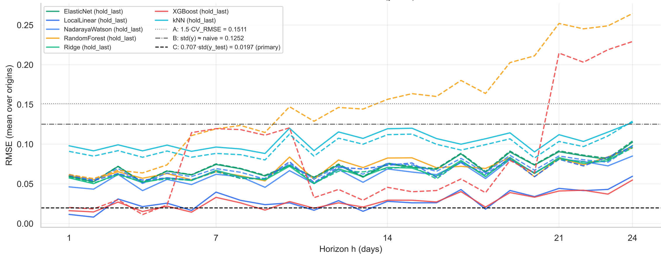
Forecast horizon curve — Flood-It! (ycnex) / stickiness
