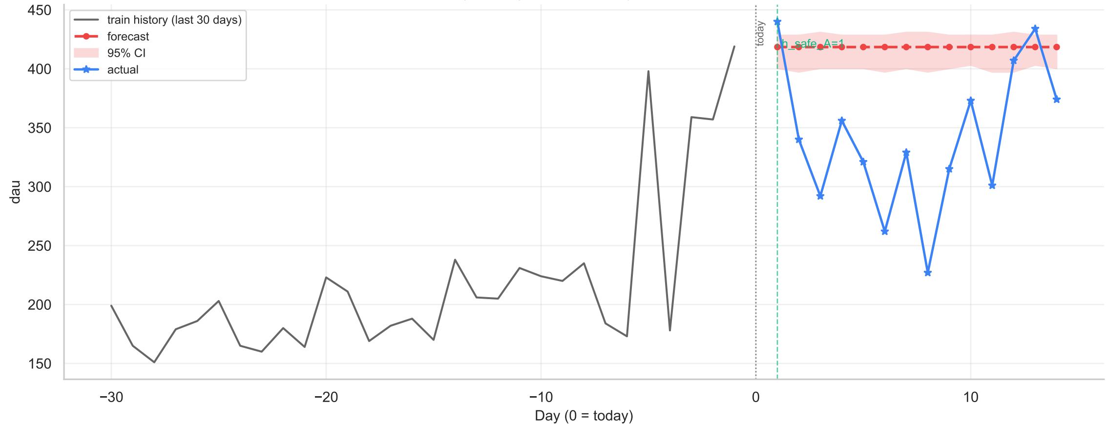
Flood-It! 2 (провал) / dau — 14-day forecast with 95% CI
