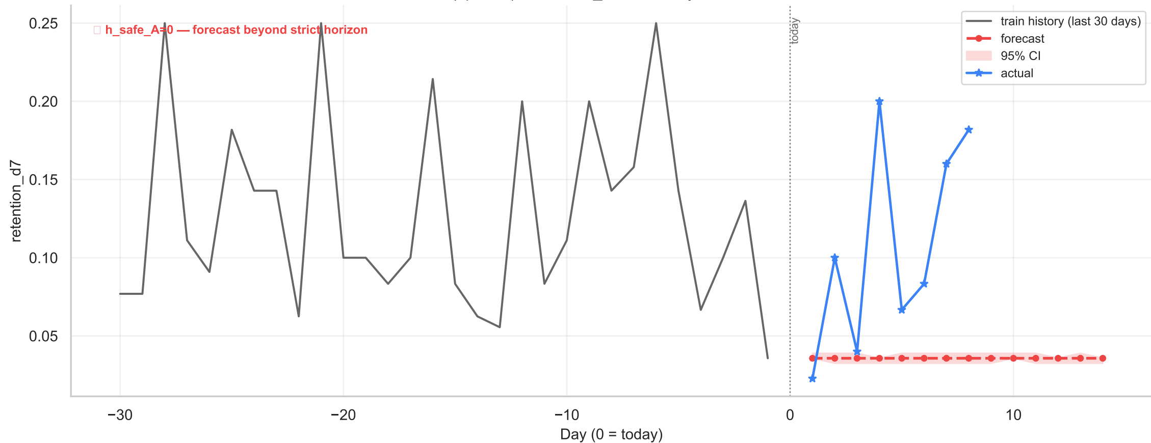
Flood-It! 2 (провал) / retention_d7 — 14-day forecast with 95% CI
