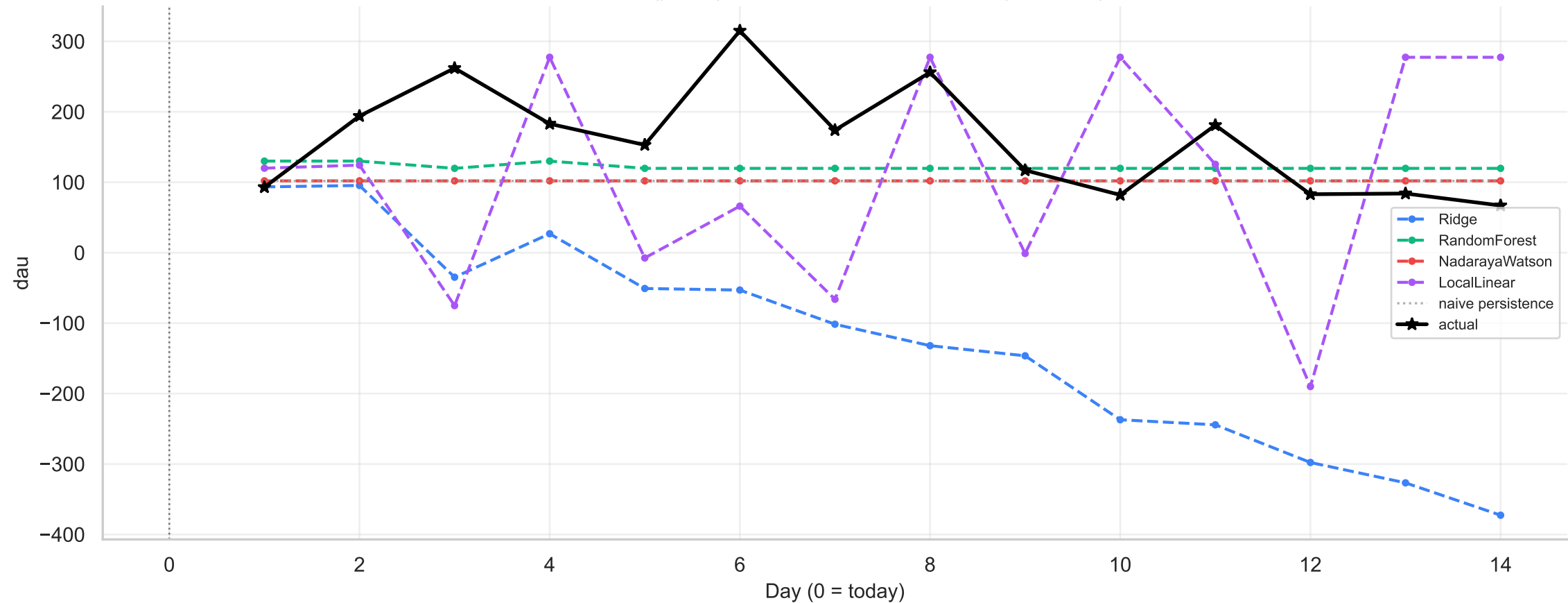
Flood-It! (ycnex) / dau — model comparison (recursive)
