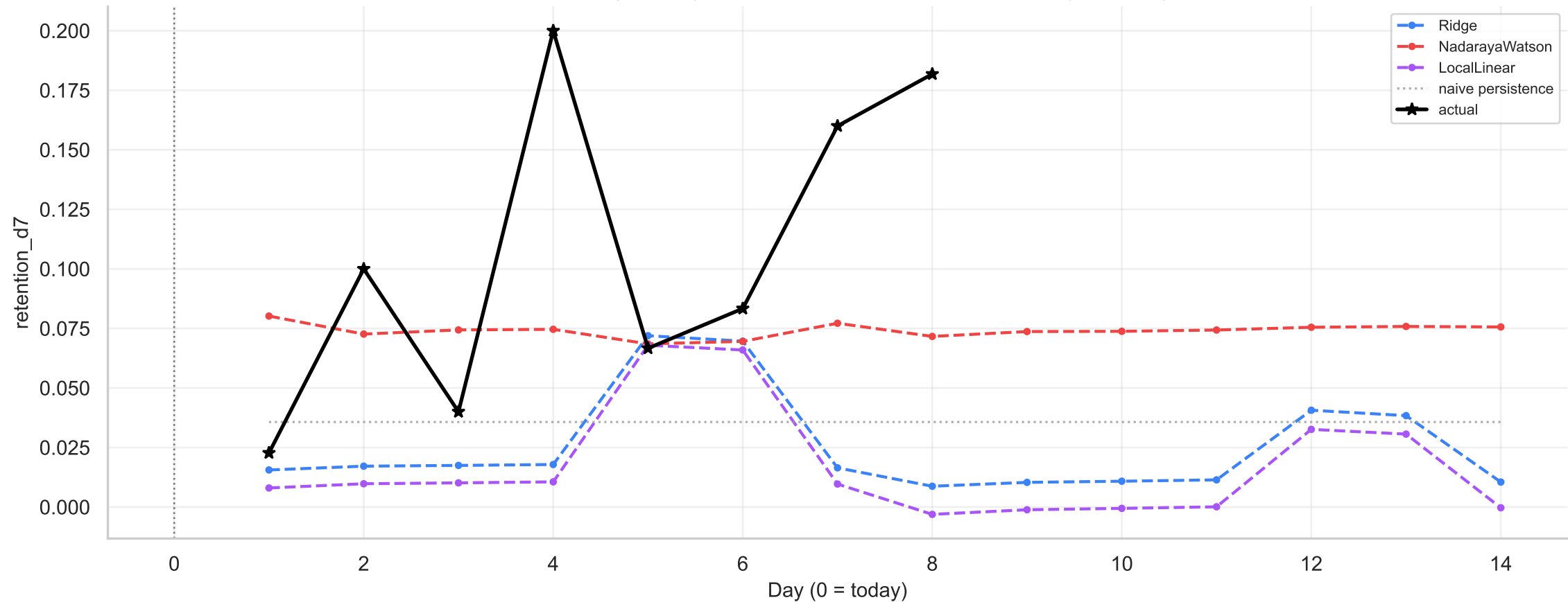
Flood-It! 2 (провал) / retention_d7 — model comparison (recursive)
