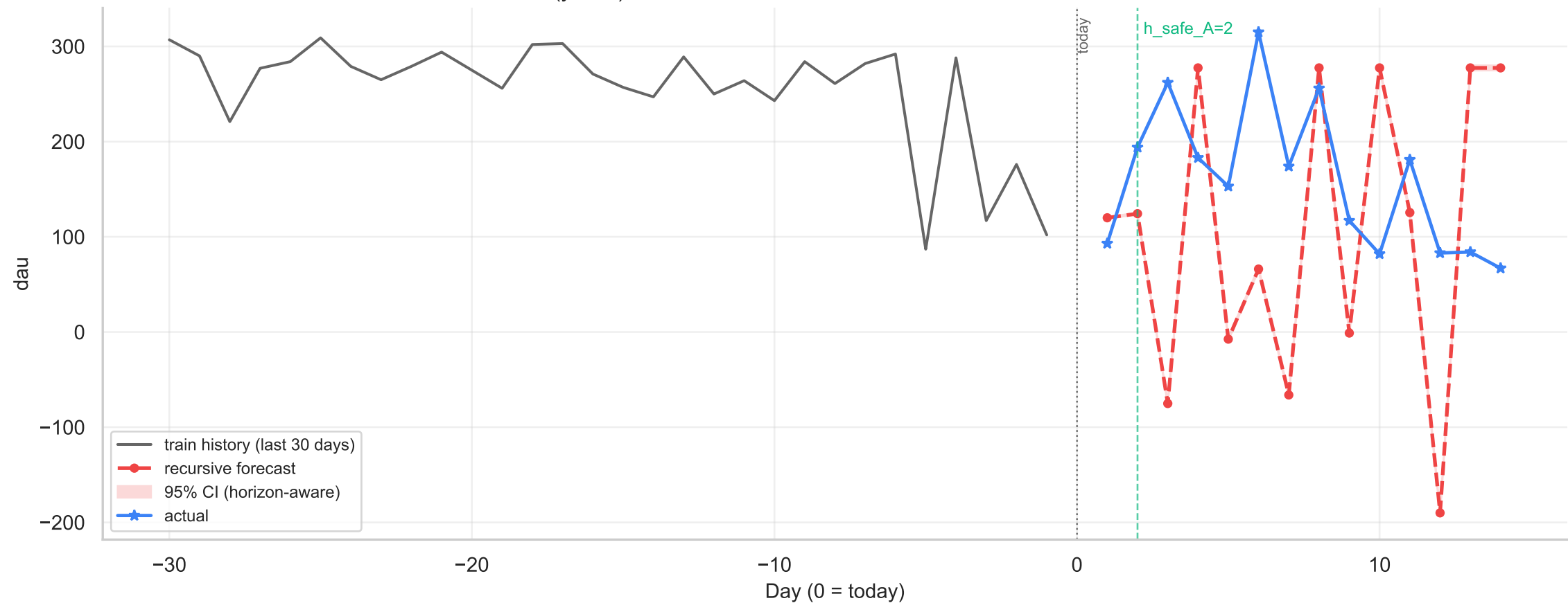
Flood-It! (ycnex) / dau / LocalLinear — recursive forecast h=14 with 95% CI
