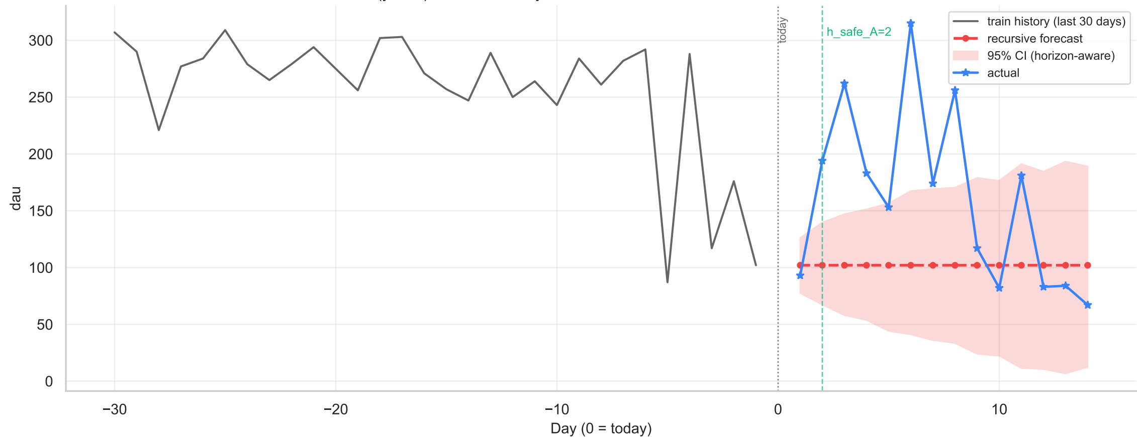
Flood-It! (ycnex) / dau / NadarayaWatson — recursive forecast h=14 with 95% CI
