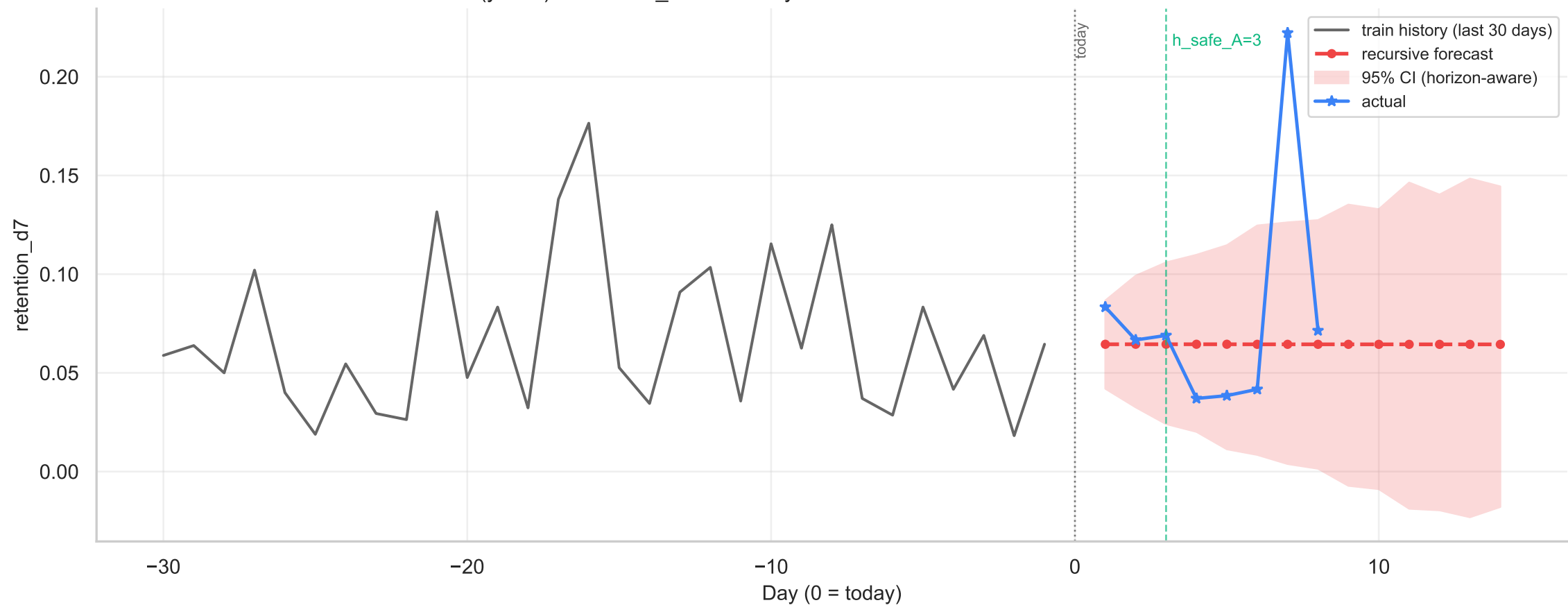
Flood-It! (ycnex) / retention_d7 / NadarayaWatson — recursive forecast h=14 with 95% CI
