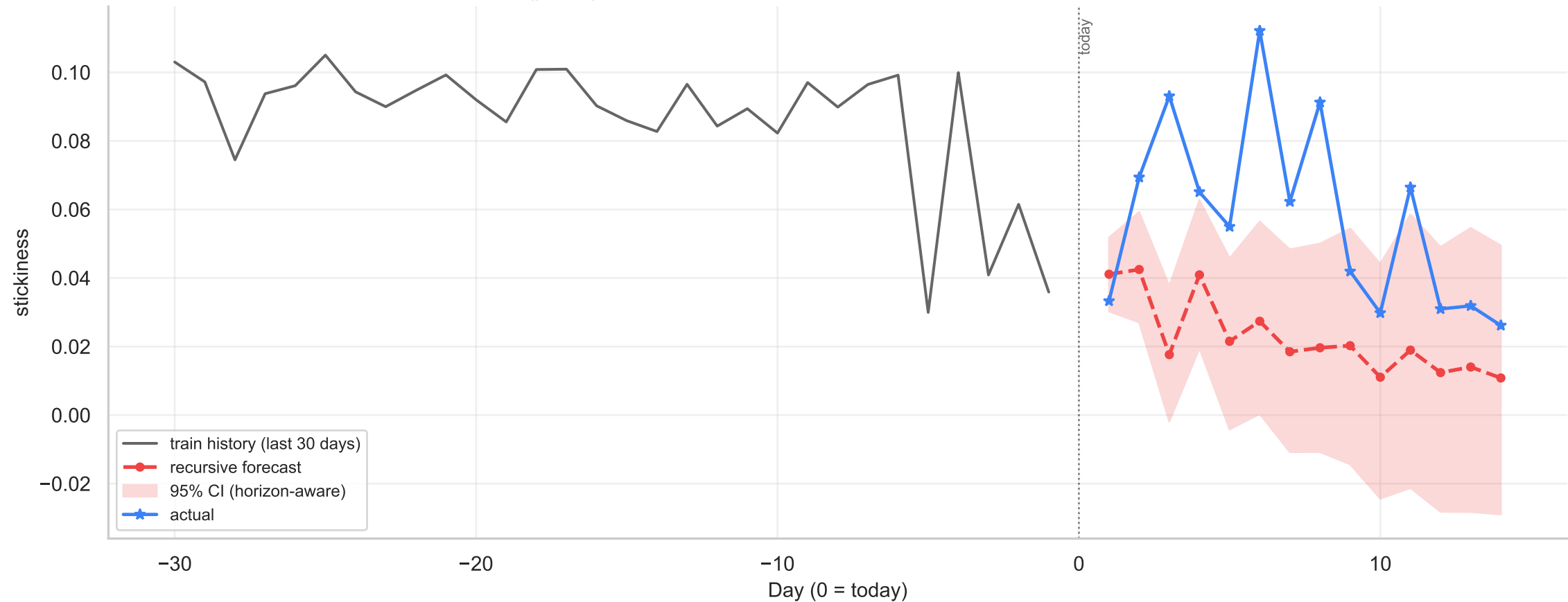
Flood-It! (ycnex) / stickiness / LocalLinear — recursive forecast h=14 with 95% CI
