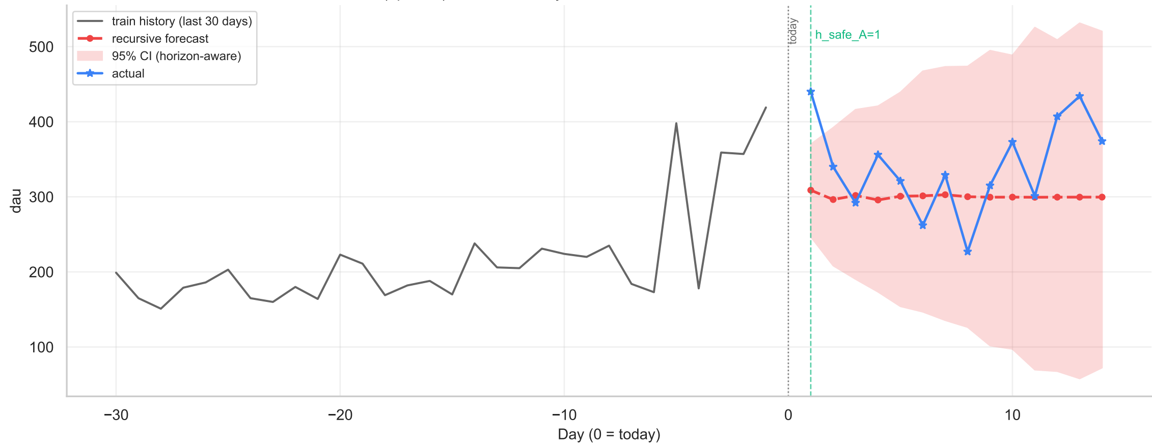
Flood-It! 2 (провал) / dau / NadarayaWatson — recursive forecast h=14 with 95% CI
