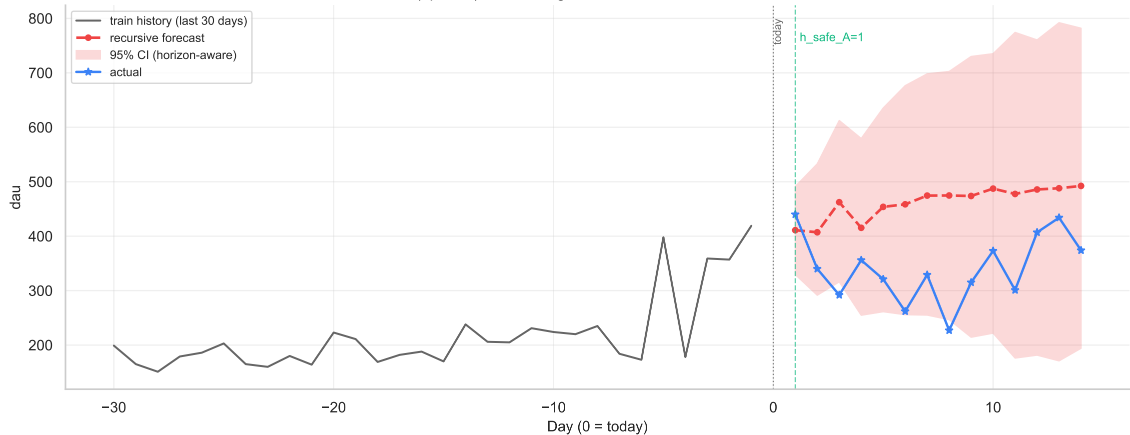
Flood-It! 2 (провал) / dau / Ridge — recursive forecast h=14 with 95% CI
