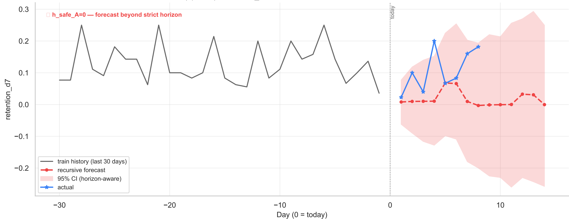
Flood-It! 2 (провал) / retention_d7 / LocalLinear — recursive forecast h=14 with 95% CI
