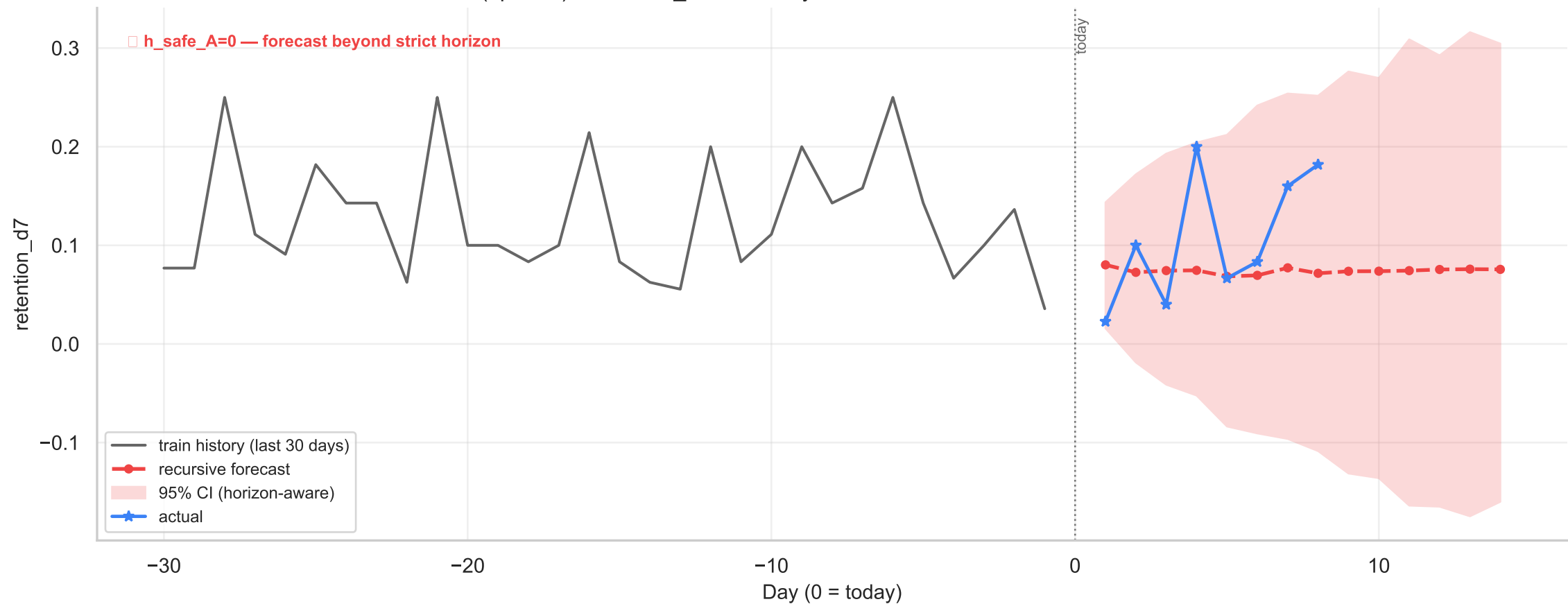
Flood-It! 2 (провал) / retention_d7 / NadarayaWatson — recursive forecast h=14 with 95% CI
