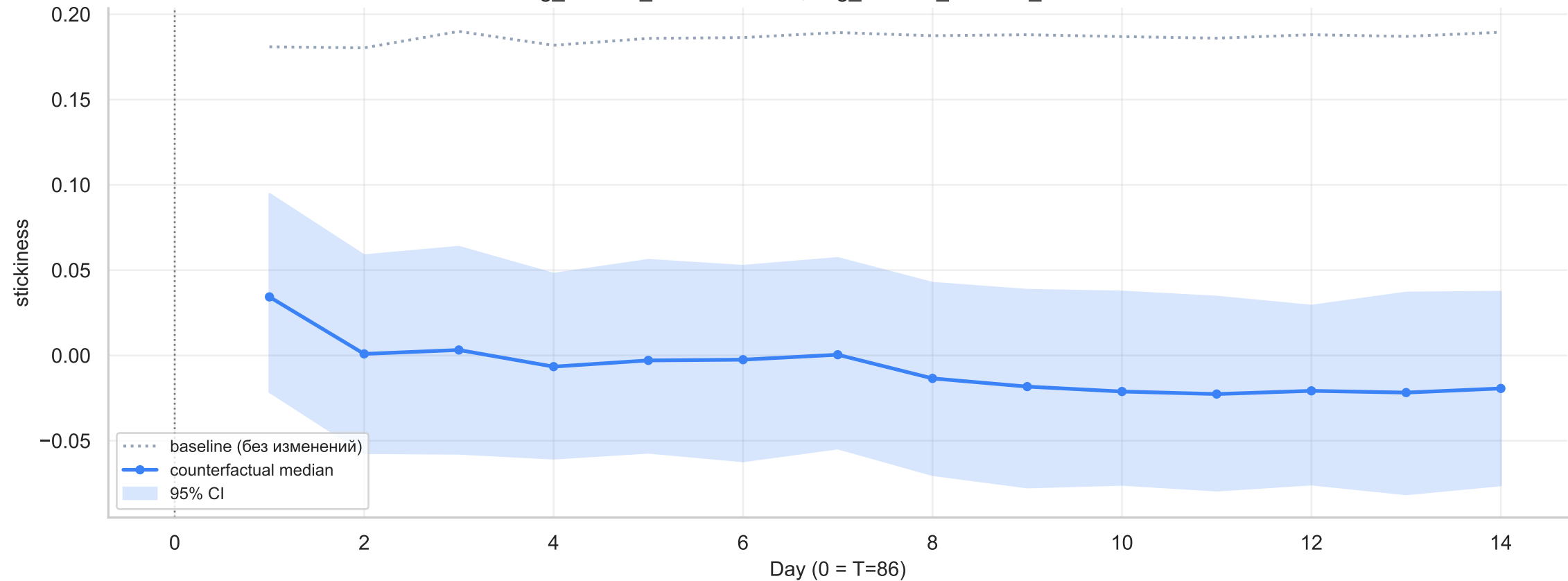
Flood-It! 2 (провал) / stickiness / combined_improvement avg_session_duration=1.270, avg_session_duration_ma7=0.91...
