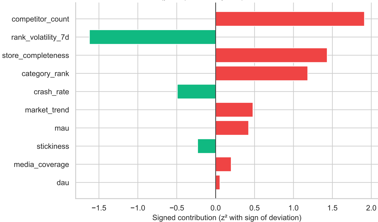
Flood-It! (ycnex) / M3 / day 55: per-feature contribution
