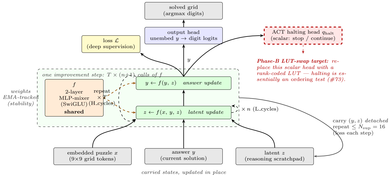
Tiny Recursive Model (TRM) — attention-free MLP-mixer Sudoku variant. A single shared 2-layer net f is applied T \times (n+1) times per improvement step (stock T=3, n=6 ; our fast config T=2, n=3 ), deep-supervised for up to N_{\text{sup}}=16 steps. \sim 5M params.
