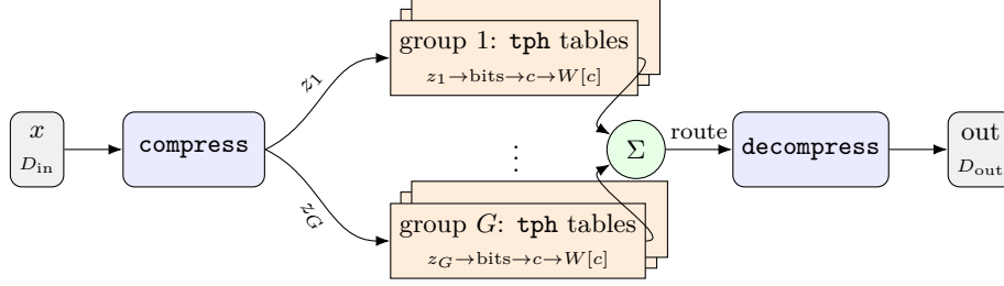
Figure 2: The ProjectionLUT data path. The input projection compress ( D_{\text{in}} \rightarrow h_{\text{in}}d_{\text{in}} ) splits x into per-group spaces z_g ; in each group the probes hash z_g to a cell per table and the tph reads are summed; the group outputs are routed and the output projection decompress ( h_{\text{out}}d_{\text{out}} \rightarrow D_{\text{out}} ) expands the result. D_{\text{in}} and D_{\text{out}} are independent and may differ. The box in the middle is the cartridge; the wrapper treats it as opaque.
