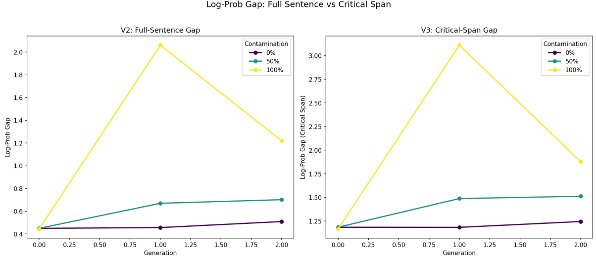
Figure 7: Comparison of full-sentence and critical-span gap variants. The critical-span gap (right) is uniformly larger and shows clearer separation between contamination levels, confirming that novel construction tokens are the primary locus of degradation.
