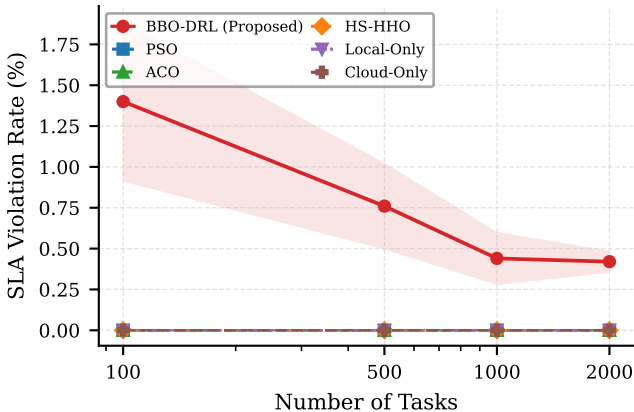
SLA Violation Rate vs. Task Scale
