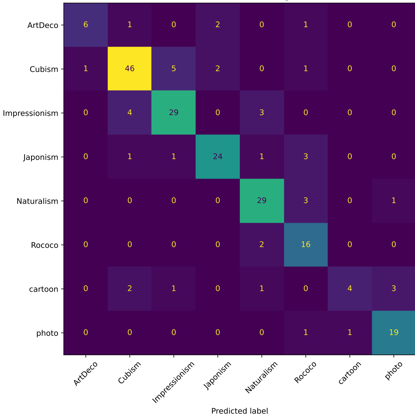
Confusion Matrix (Clustering + GB)
