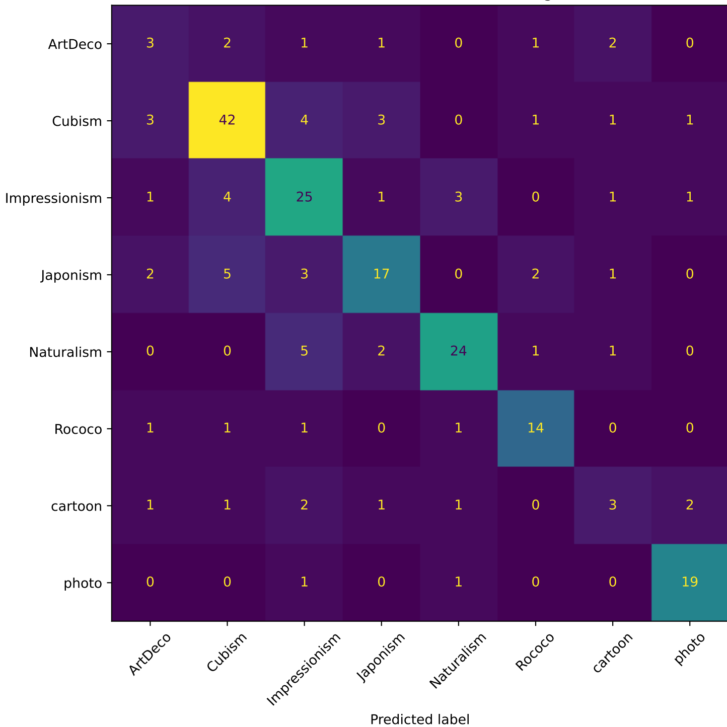
Confusion Matrix (Metric Learning)
