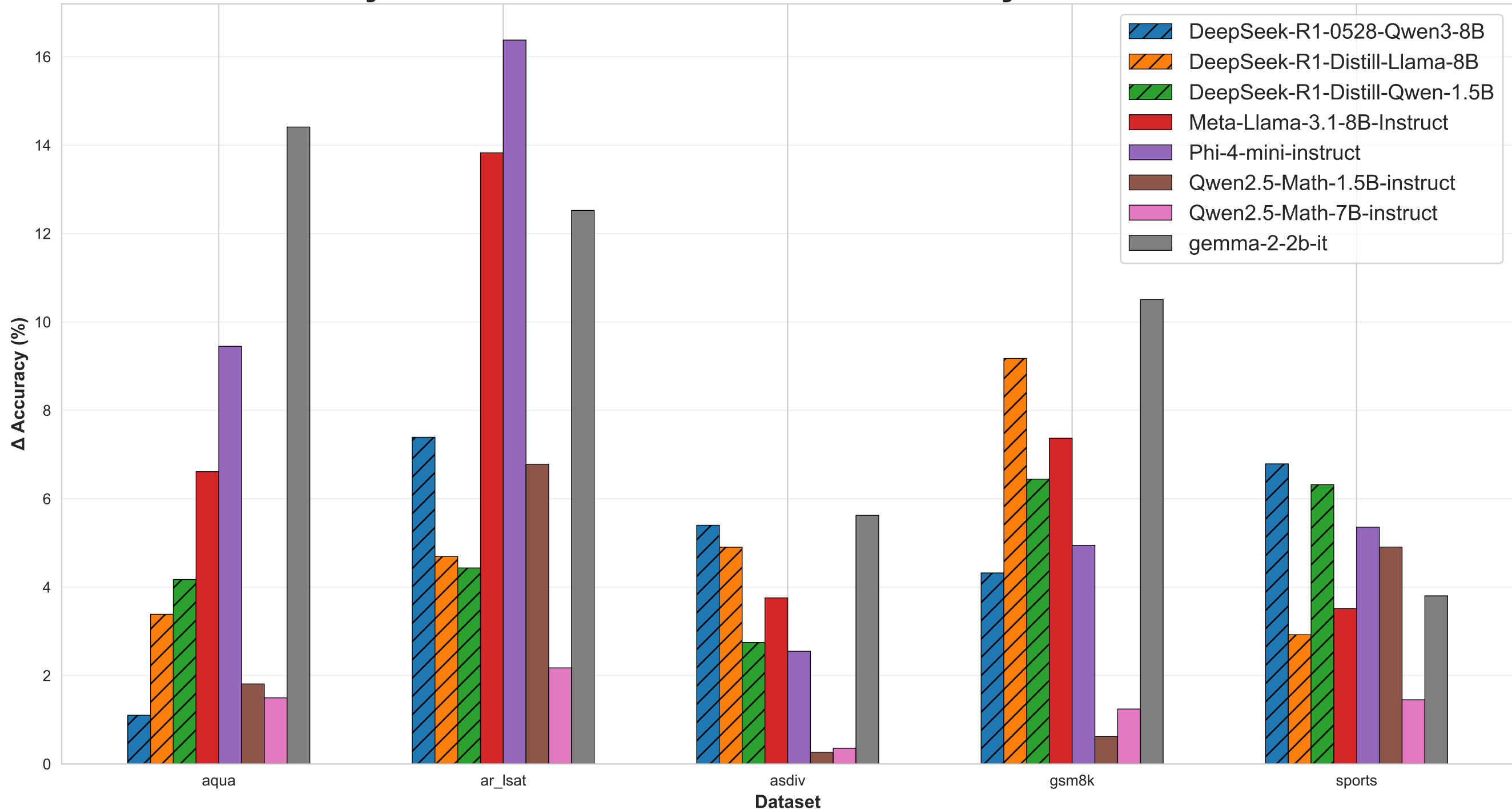
Accuracy Gain After Hint-Based Correction by Model and Dataset
