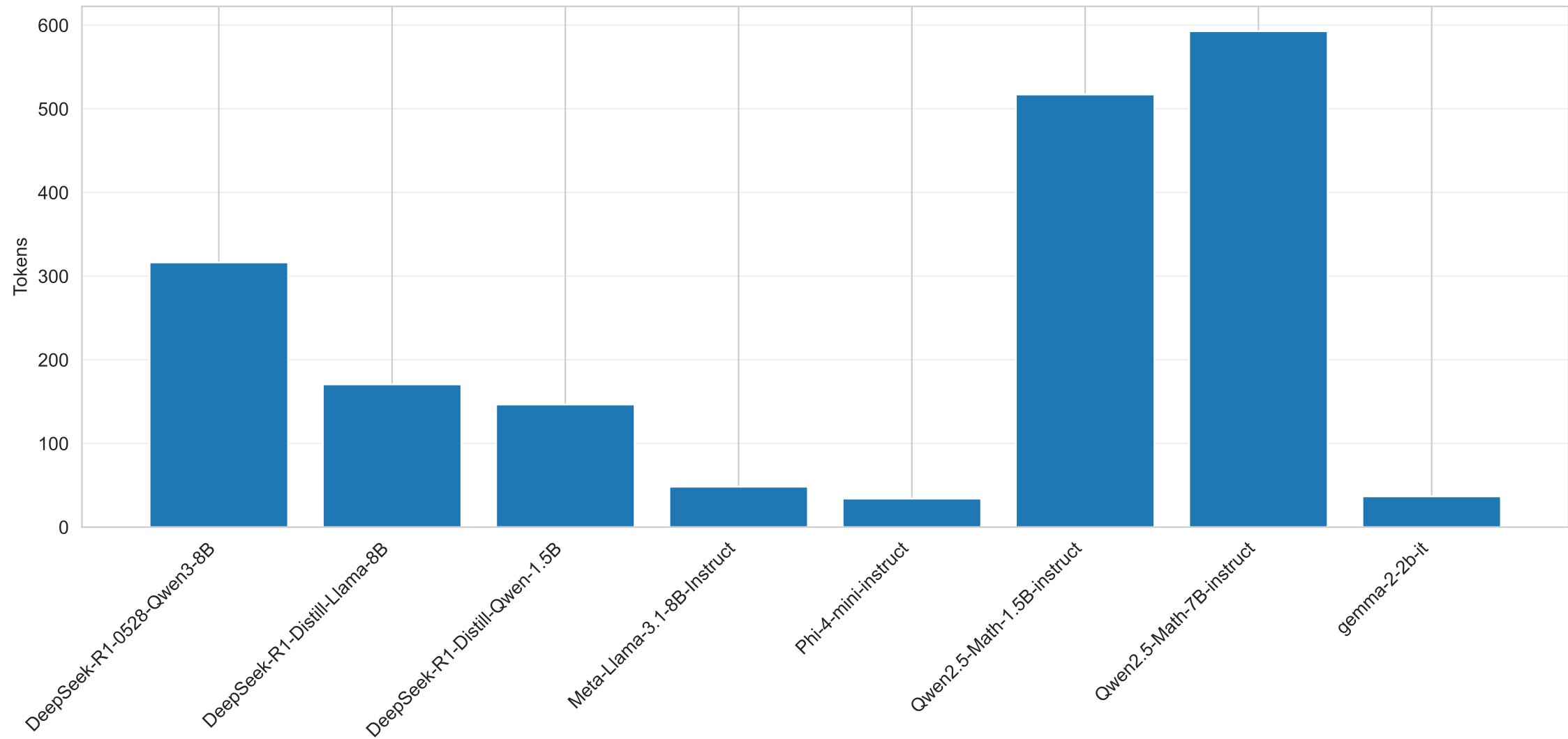
Average hint tokens by model
