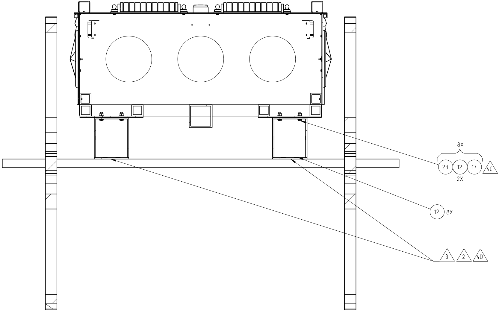
SECTION B-B SEE SHEET 3D2
