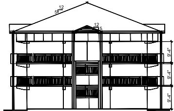
BLDG. BB270 - EAST/WEST ELEVATION - EXISTING CONDITIONS NTS
