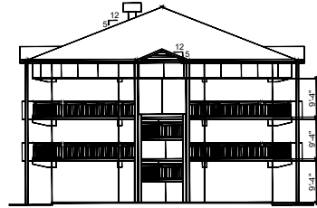
BLDG. BB265 - NORTH/SOUTH ELEVATION - EXISTING CONDITIONS NTS
