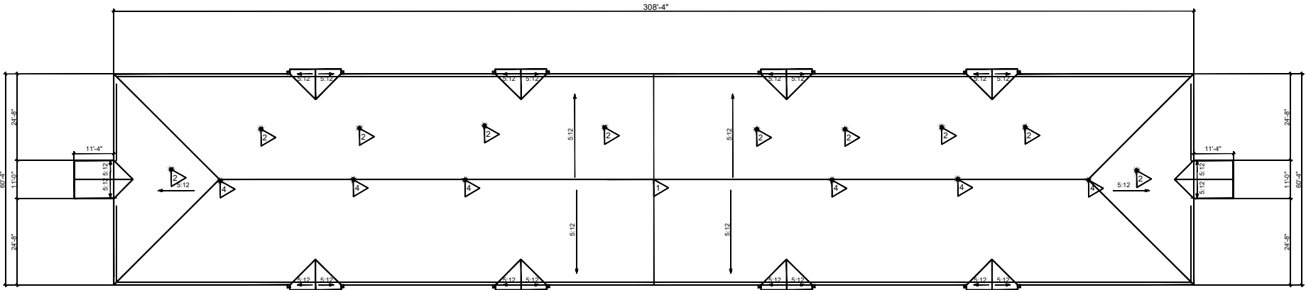
BLDG. BB265 - ROOF PLAN - EXISTING CONDITIONS NTS
