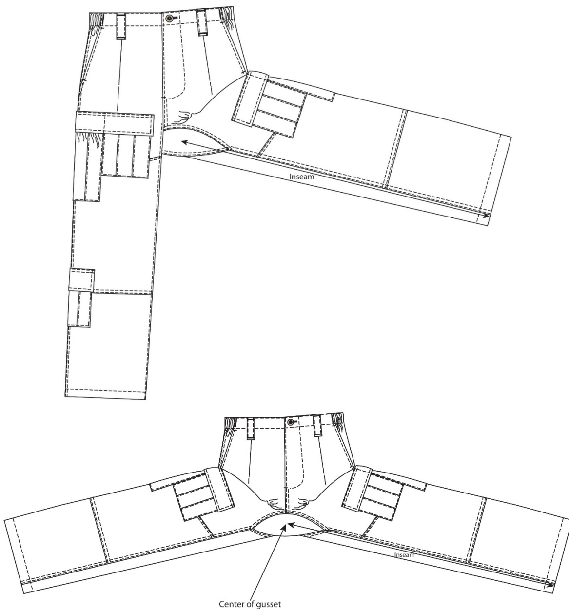
Figure 13. Trouser Inseam Finished Dimension.
