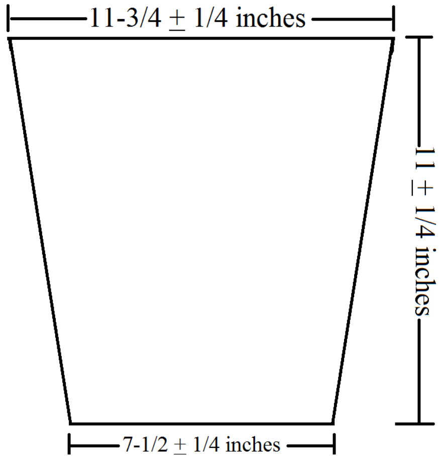
FIGURE 5. Test Specimen, percent Bite Protection Test.
