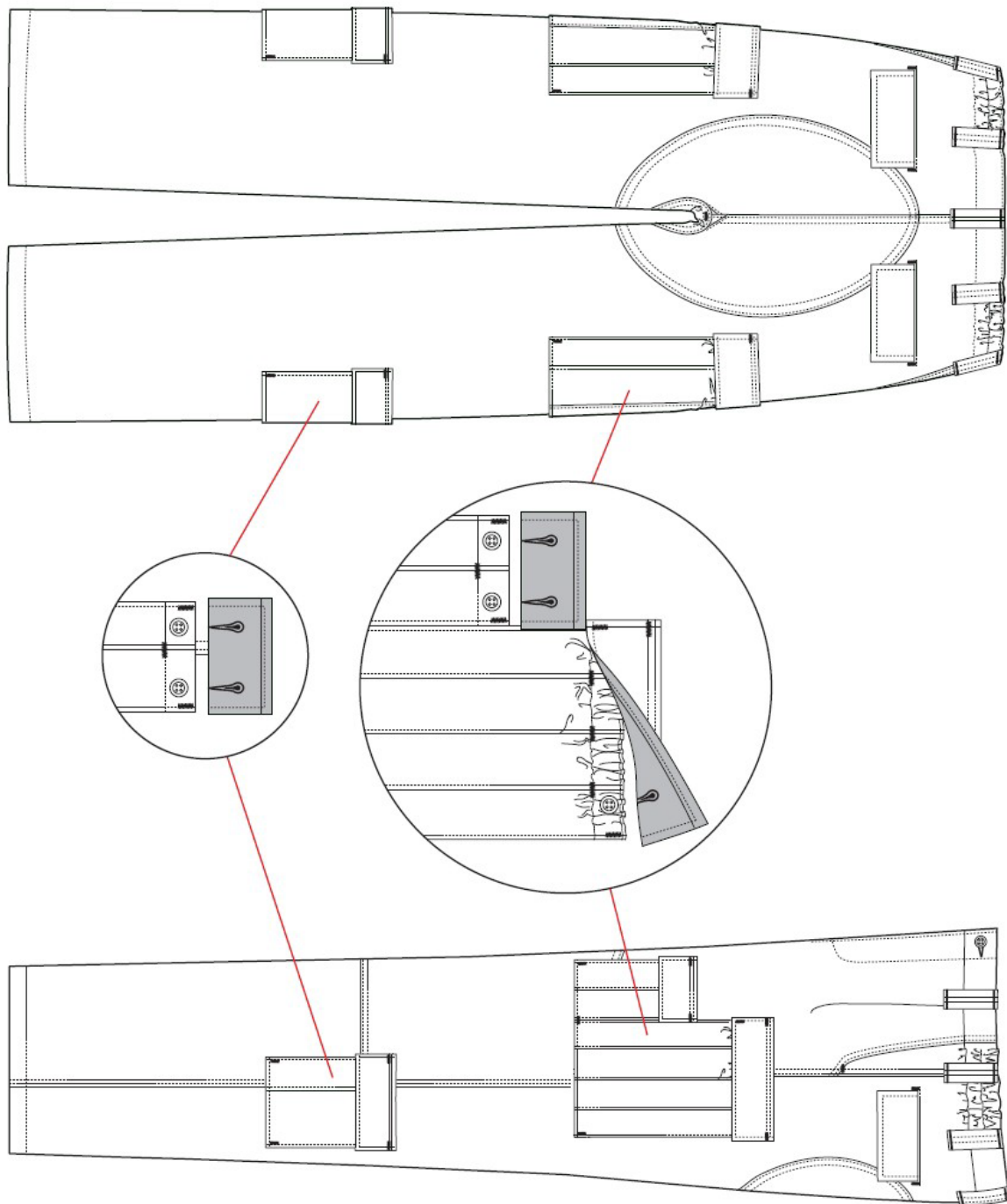
FIGURE 4. Trousers, Back and Side view with pocket detail.
