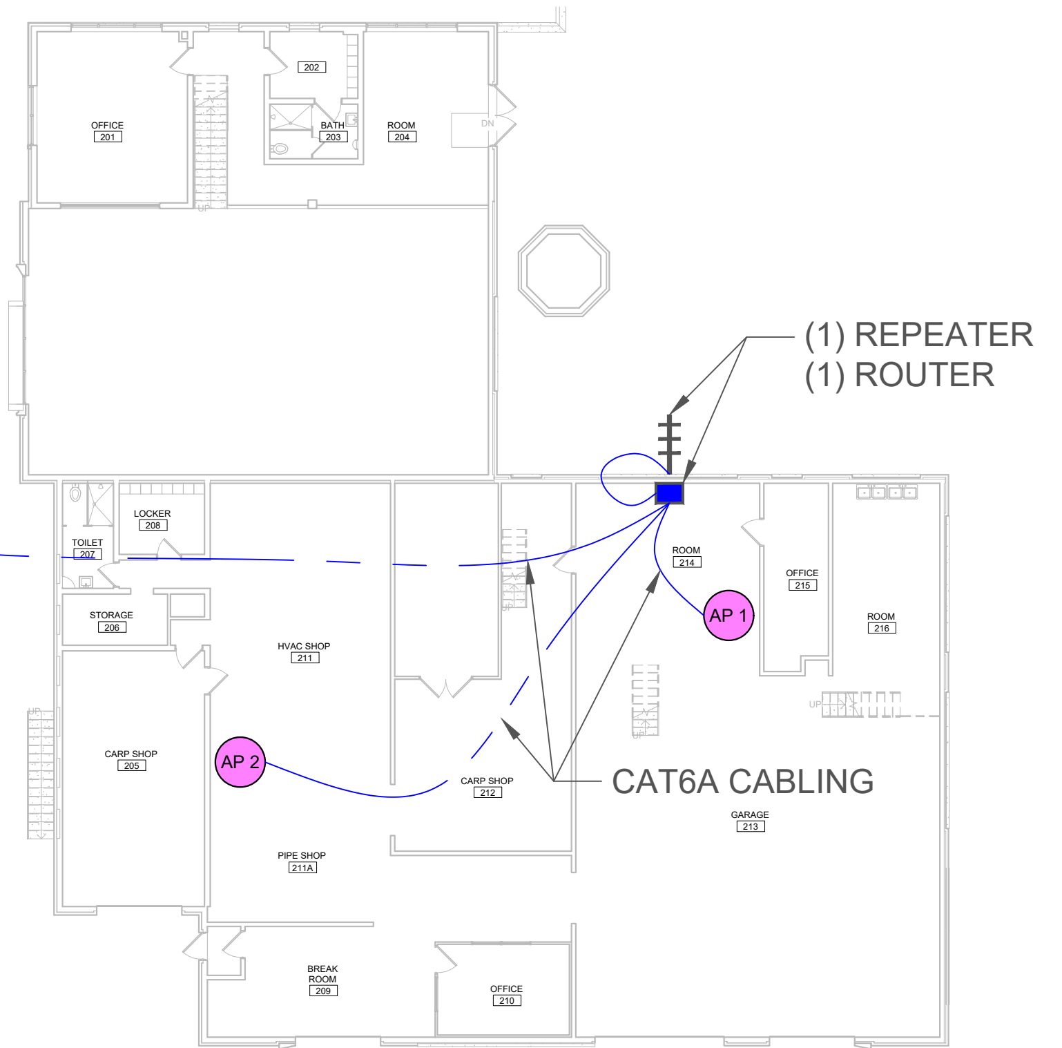
BLDG 2 SECOND FLOOR PLAN
