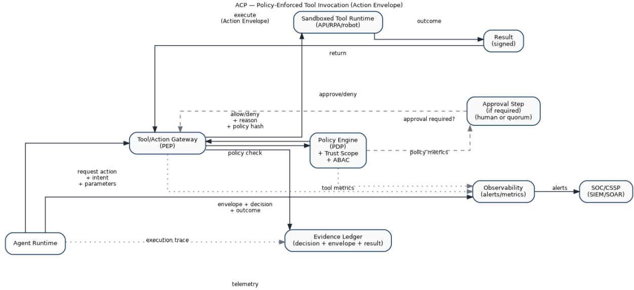
Figure 2: Action Loop
