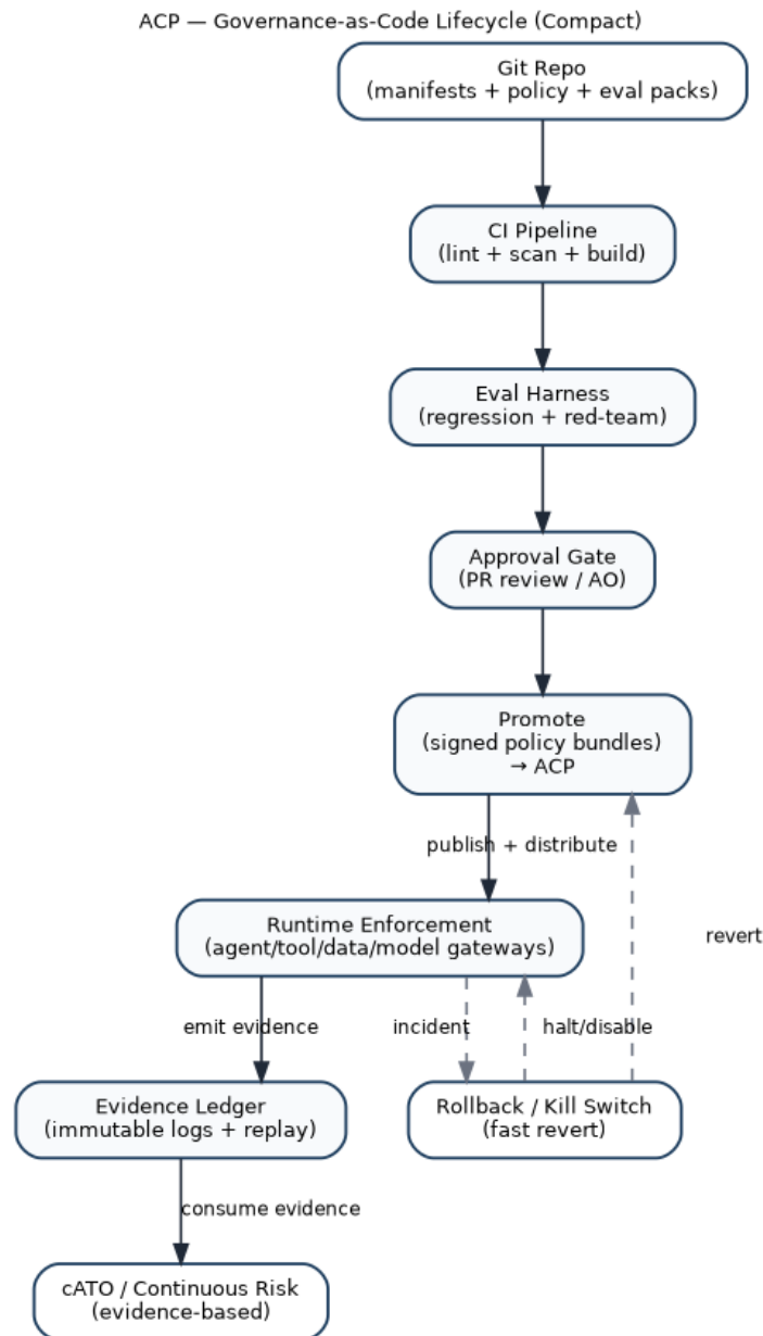
Figure 3: Governance Lifecycle
