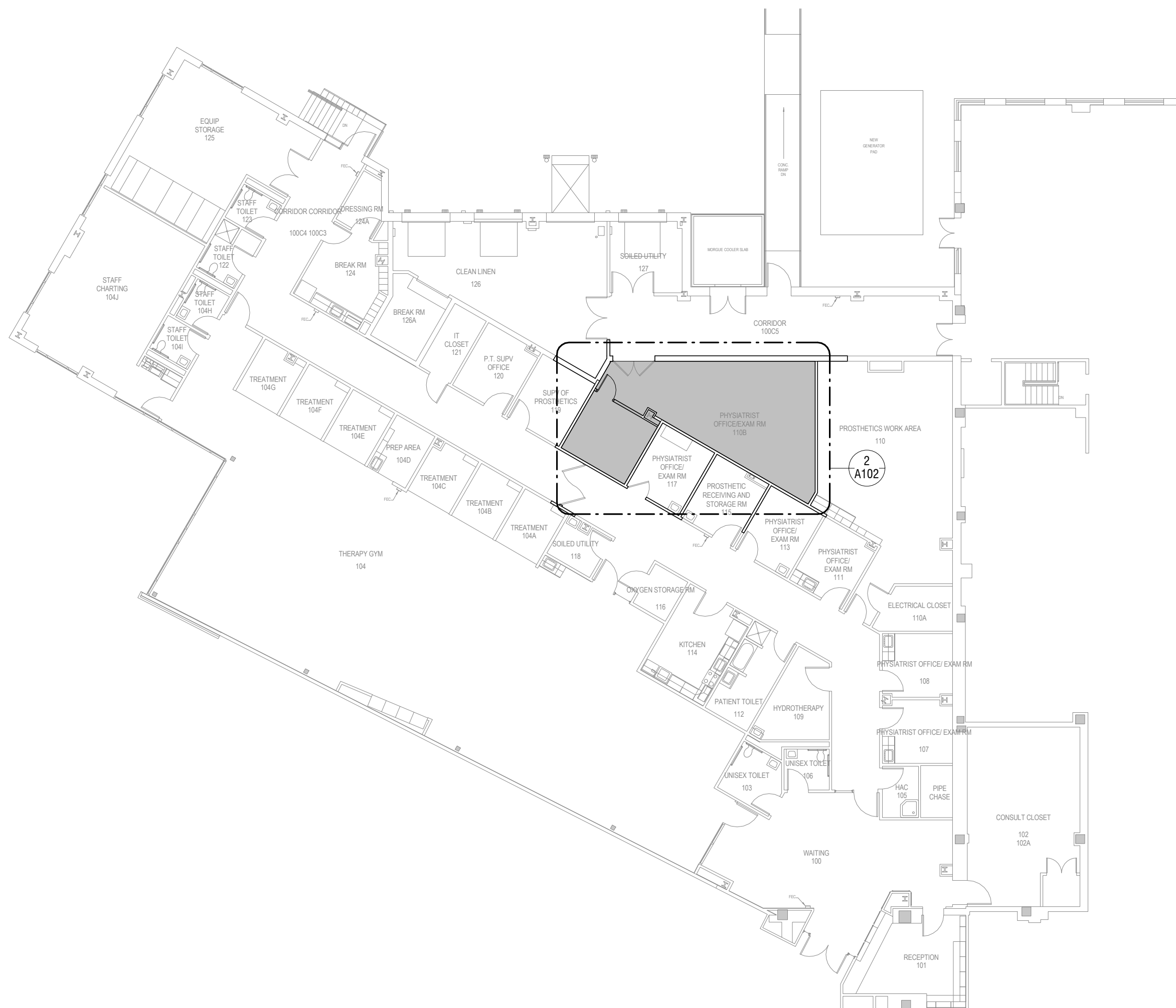
BUILDING 102 - FIRST FLOOR ARCHITECTURAL OVERALL PLAN 1/16" = 1'-0"
