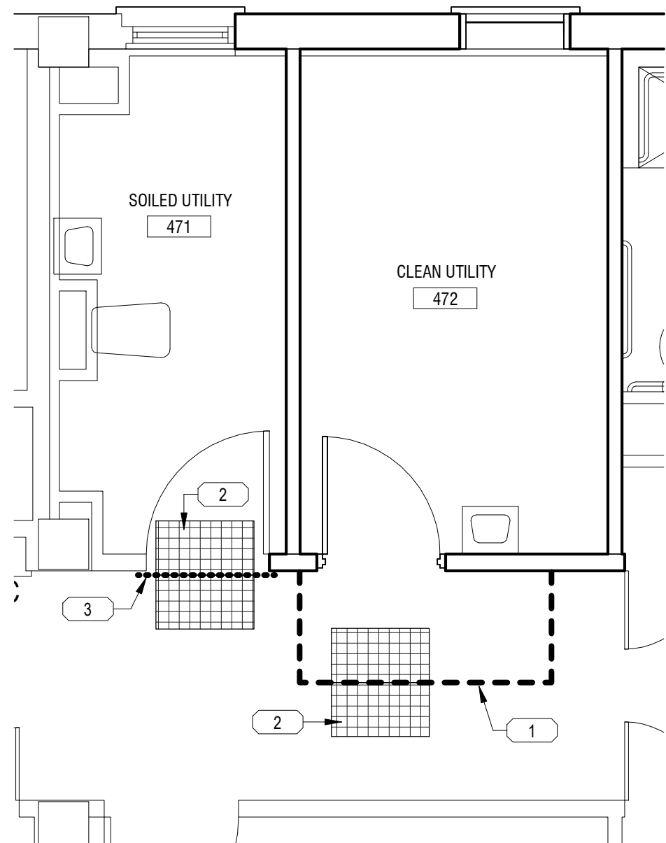
5 Bldg 01-04 FOURTH FLOOR - 472 - ICRA 1/4" = 1'-0"
