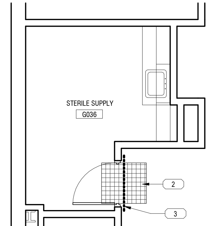
3 Bldg 01-00 BASEMENT FLOOR - G036 - ICRA 1/4" = 1'-0"
