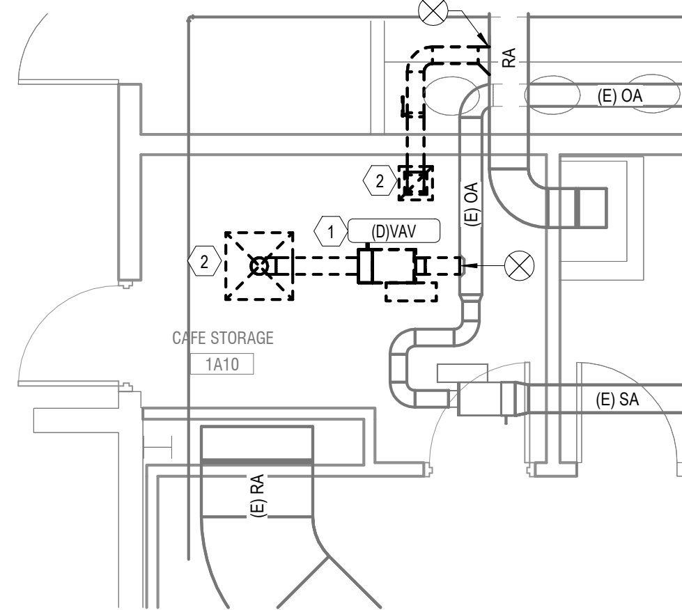
Bldg 37-01-FIRST FLOOR HVAC DEMOLITION PLAN -ROOM 1A10
