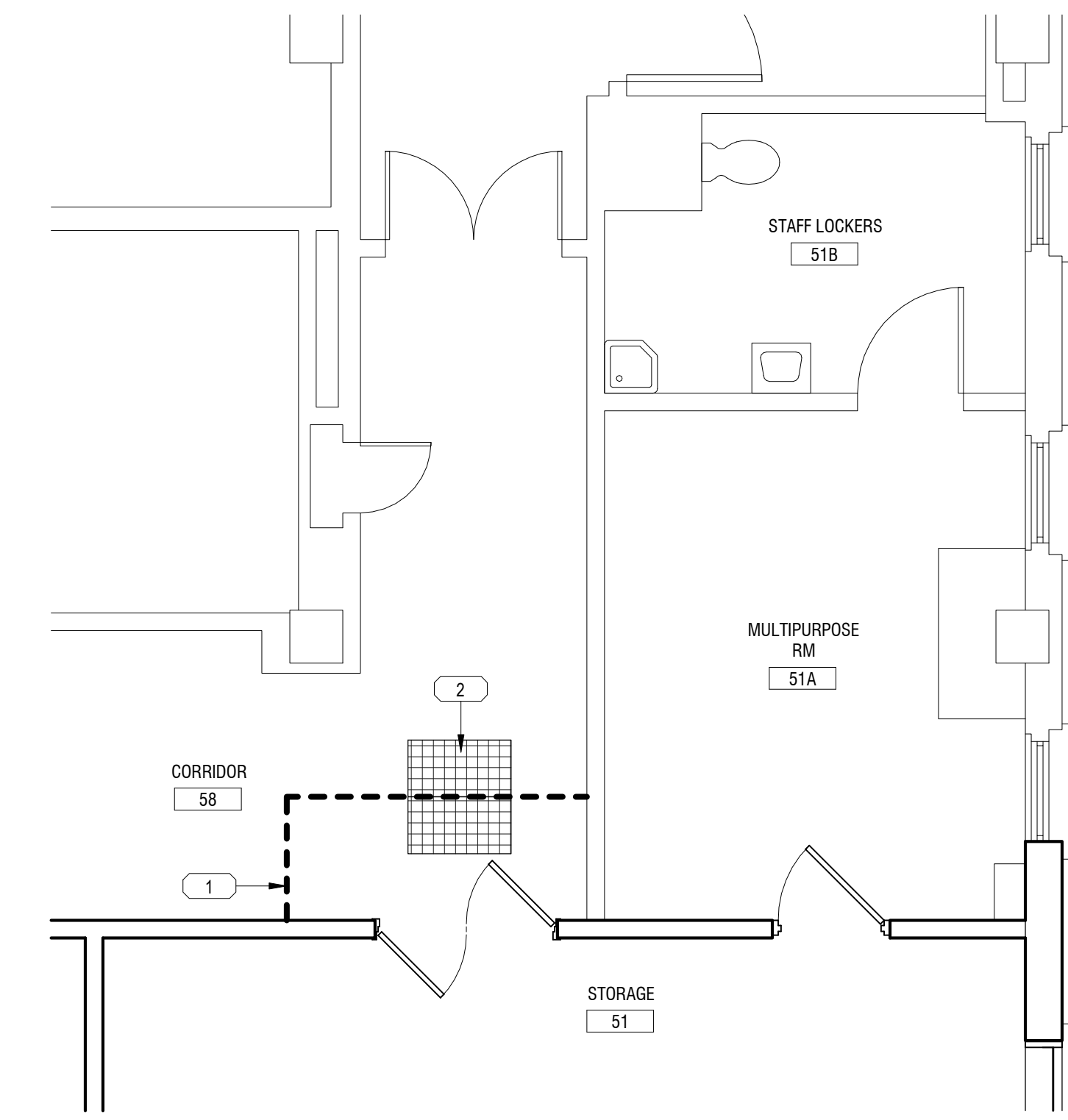
1 Bldg 01-00 BASEMENT FLOOR - RM 51 - ICRA 1/4" = 1'-0"
