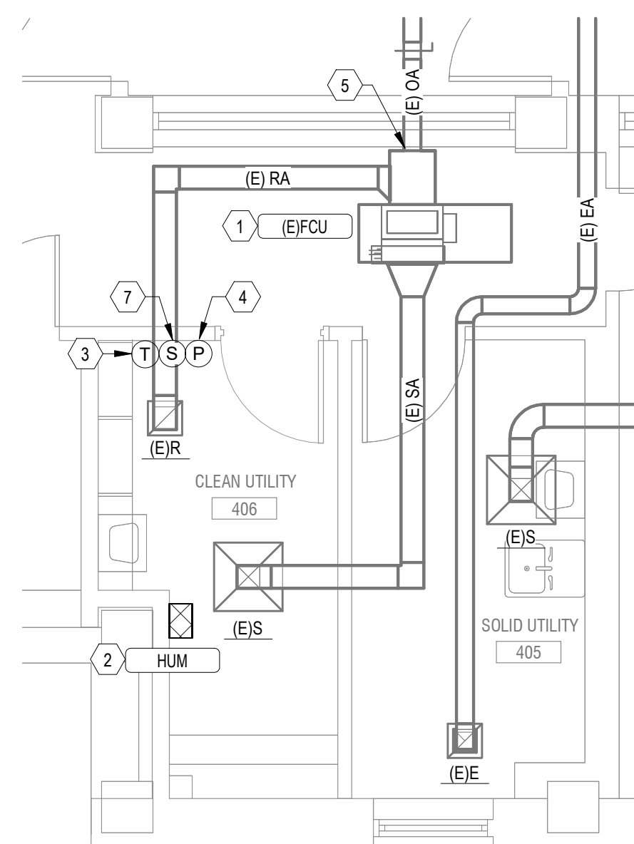
Bldg 01-04 FOURTH FLOOR HVAC PLAN - ROOM 406
