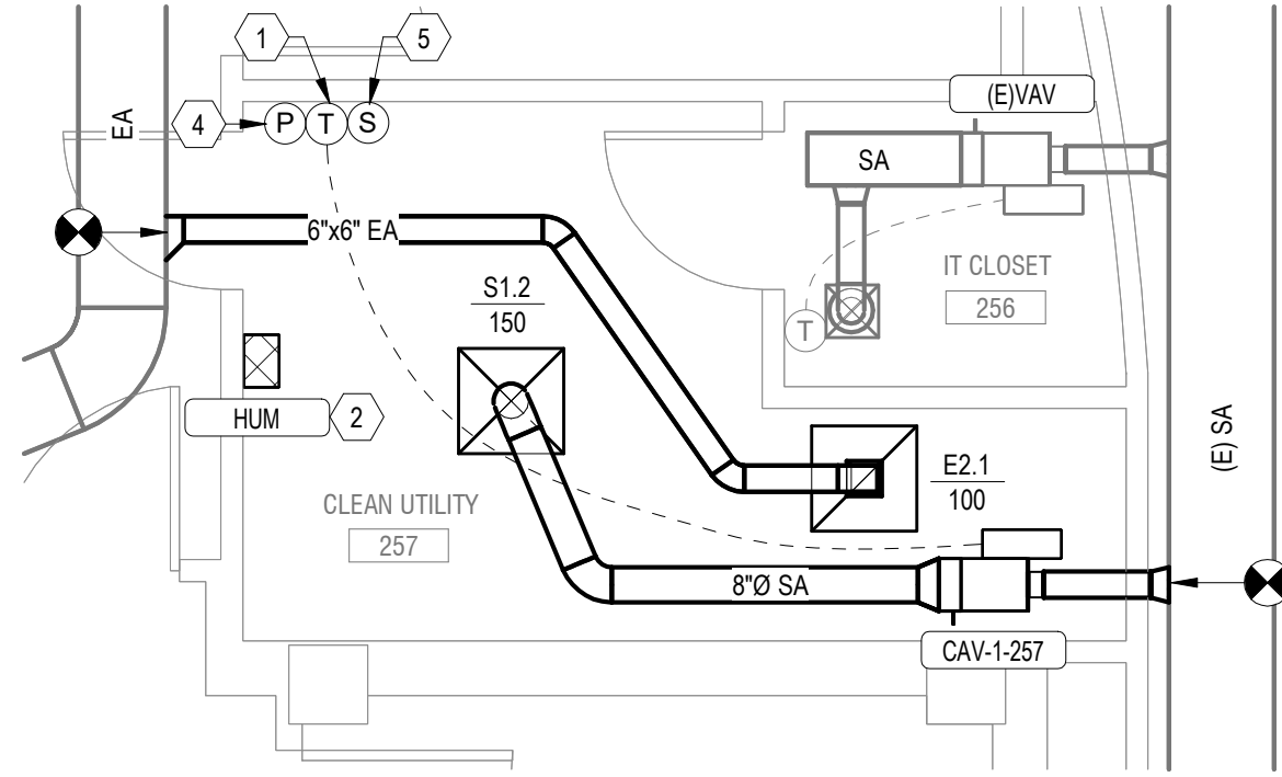
Bldg 01-02 SECOND FLOOR HVAC PLAN - ROOM 257
