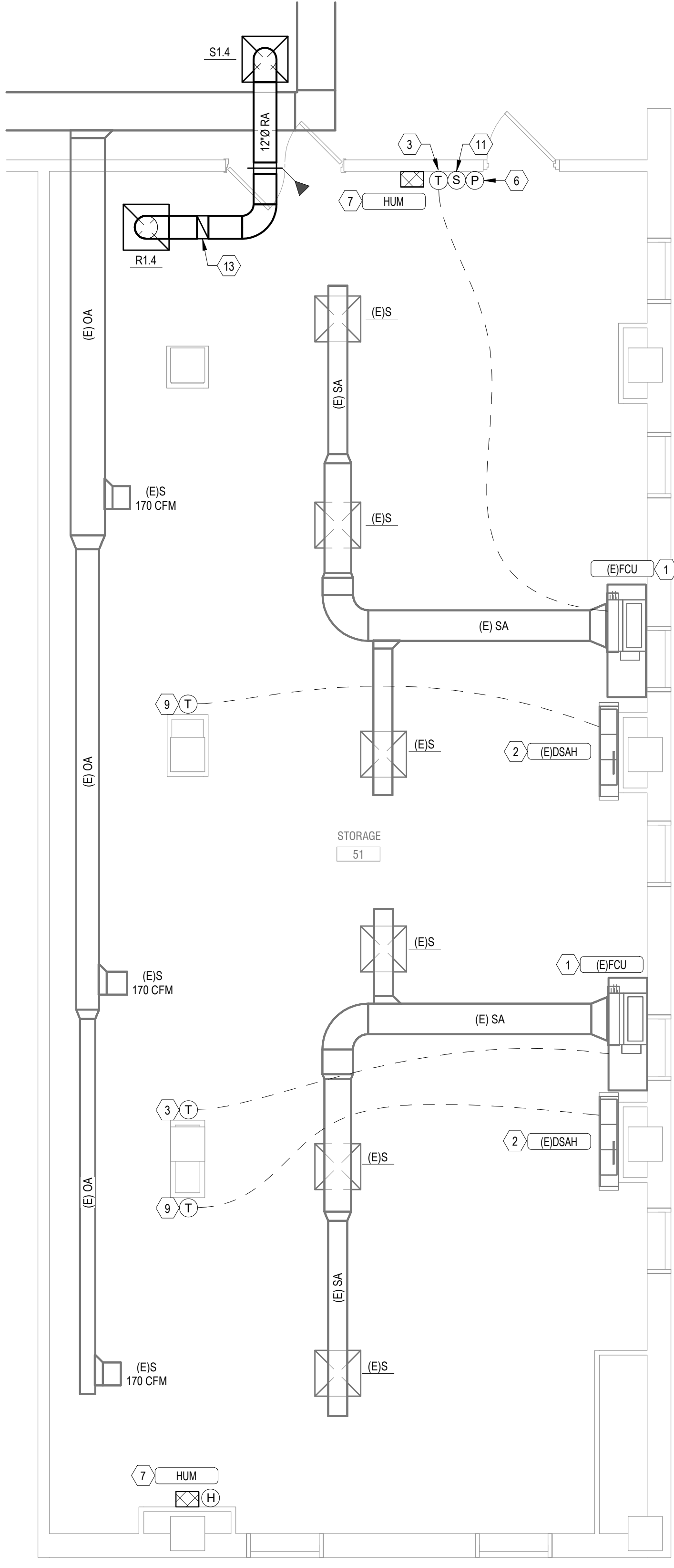
Bldg 01-00 BASEMENT FLOOR HVAC PLAN - ROOM 51
