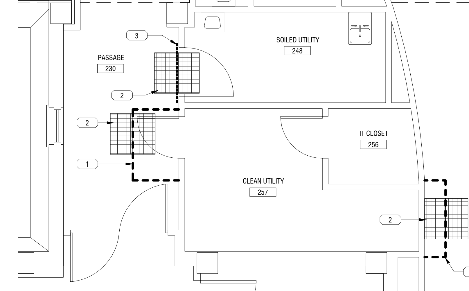
7 Bldg 01-02 SECOND FLOOR - 257-ICRA 1/4" = 1'-0"
