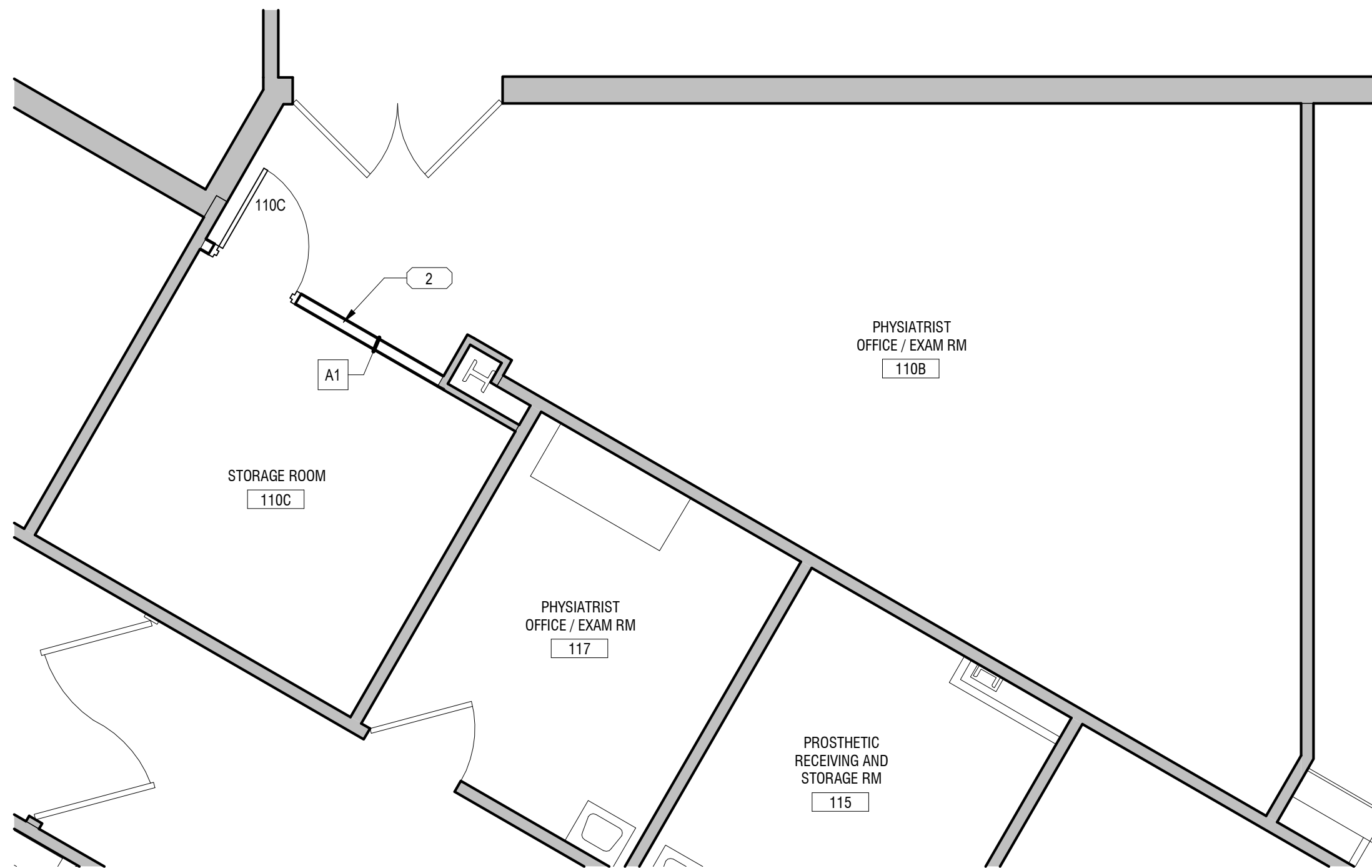
BUILDING 102 - FIRST FLOOR ENLARGED PLAN 1/4" = 1'-0"
