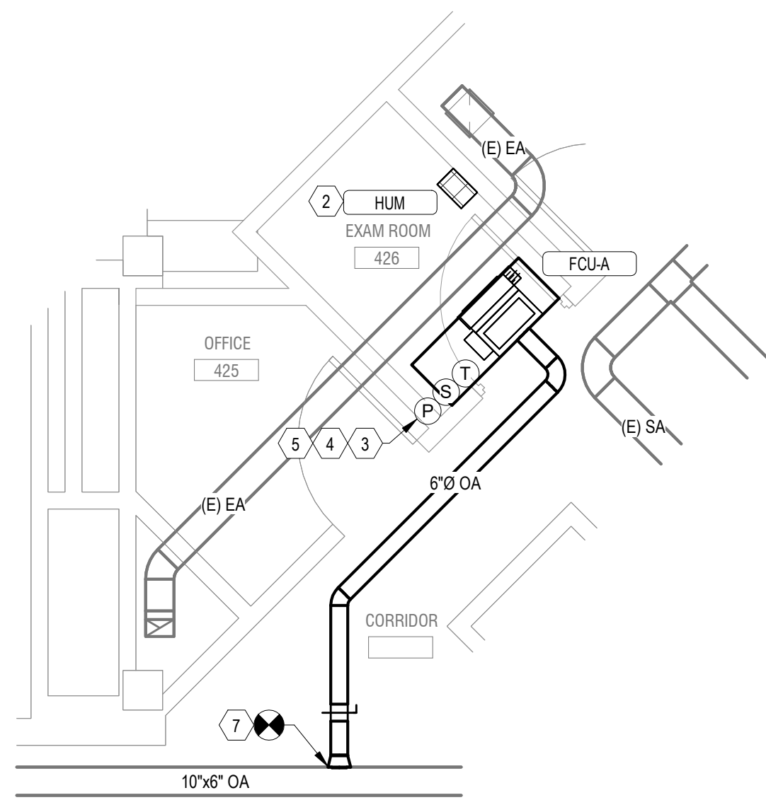
BID DEDUCT 1 - Bldg 17-04 FOURTH FLOOR HVAC PLAN - ROOM 426 1/4" = 1'-0"
