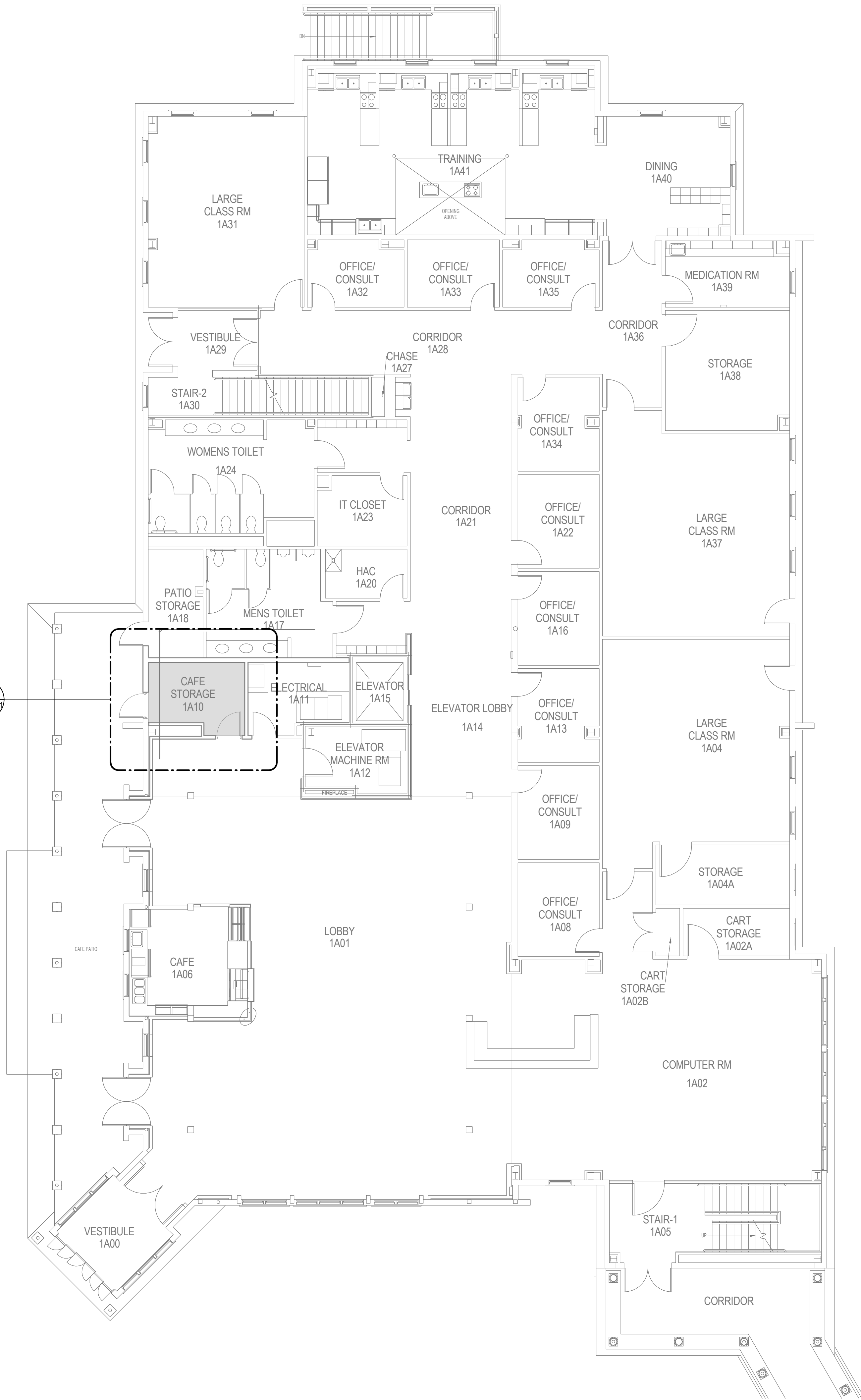
1 Bldg 37-01-FIRST FLOOR HVAC DEMOLITION PLAN 1/8" = 1'-0"
