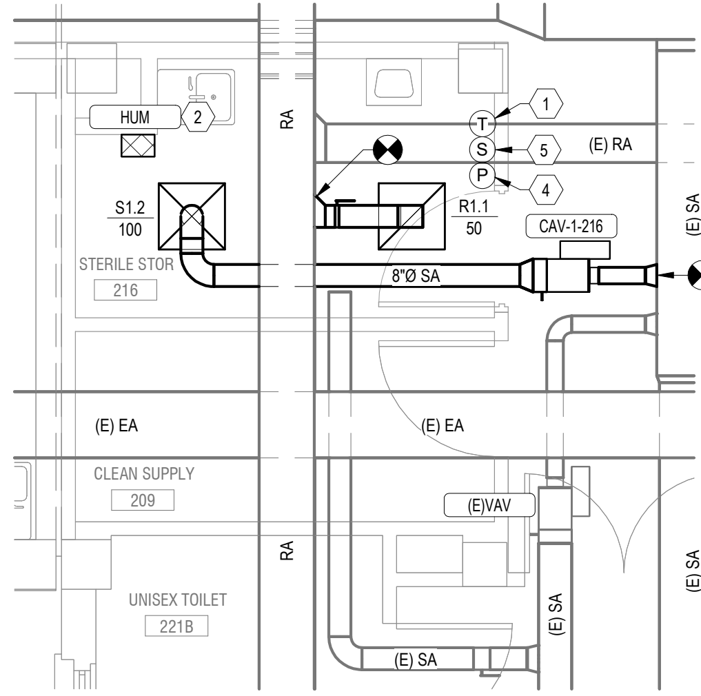
Bldg 01-02 SECOND FLOOR HVAC PLAN - ROOM 216
