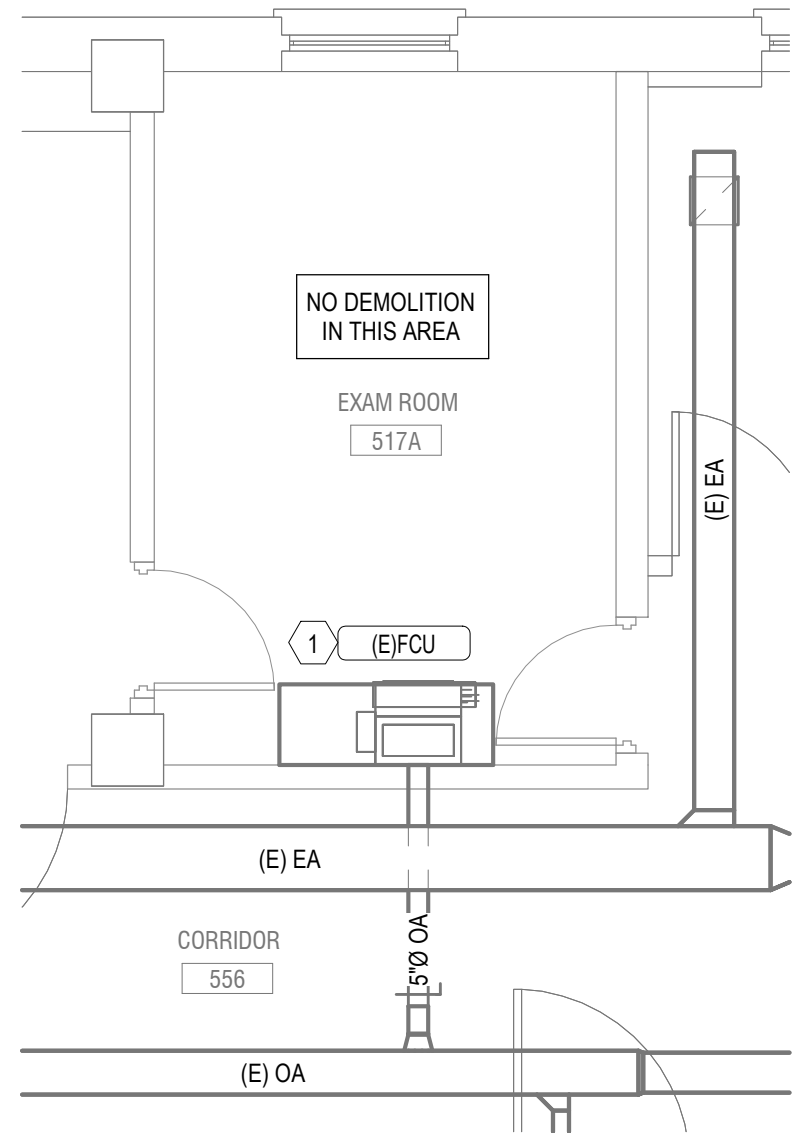
Bldg 18-05 FIFTH FLOOR HVAC DEMOLITION PLAN - ROOM 517A
