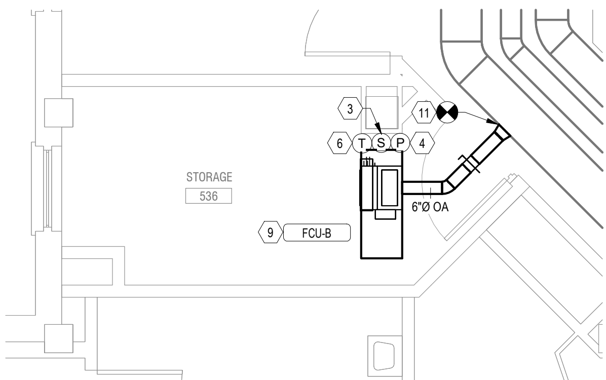
BID DEDUCT 1 - Bldg 17-05 FIFTH FLOOR HVAC PLAN - ROOM 536 1/4" = 1'-0"
