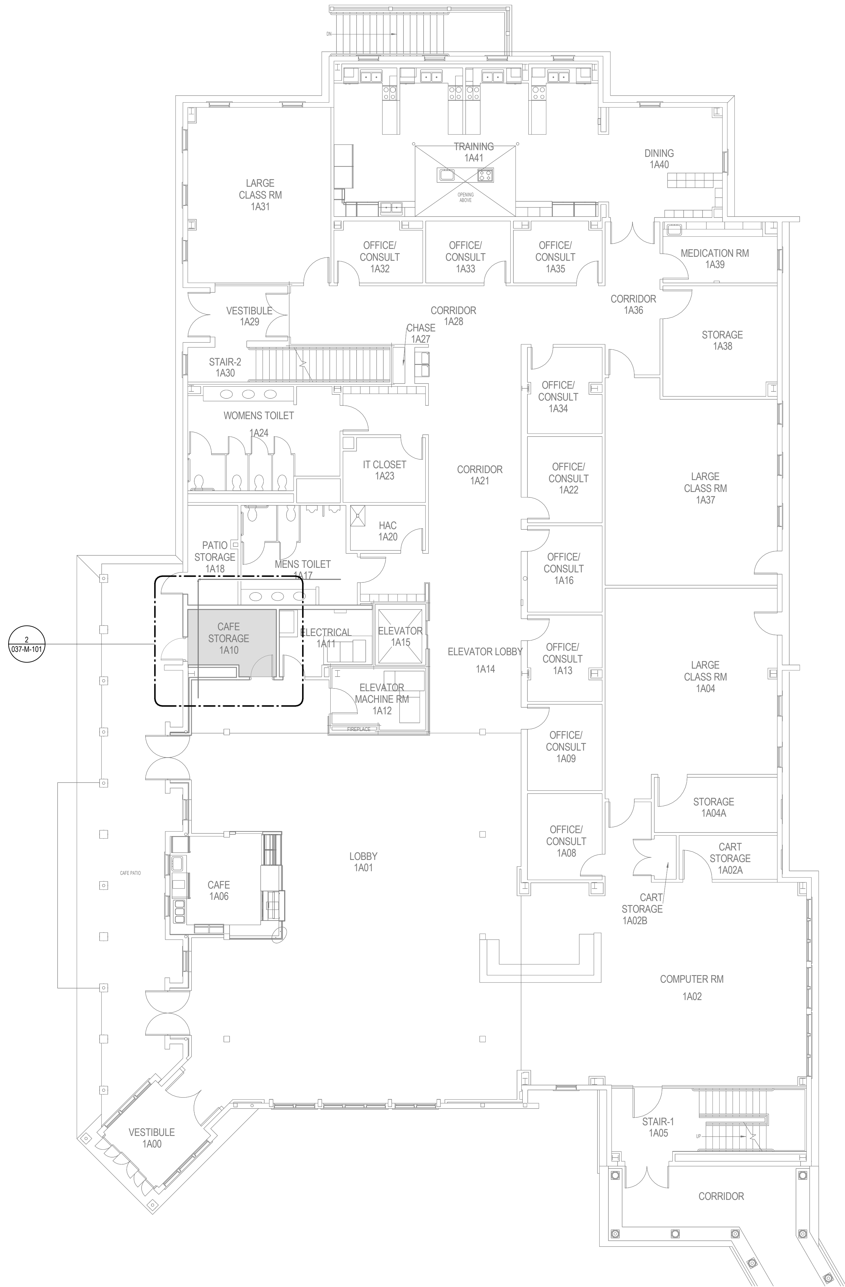
1 Bldg 37-01-FIRST FLOOR HVAC PLAN
