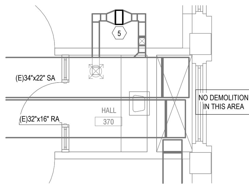
4 Bldg 01-03 THIRD FLOOR HVAC DEMOLITION PLAN - ROOM 370 1/4" = 1'-0"
