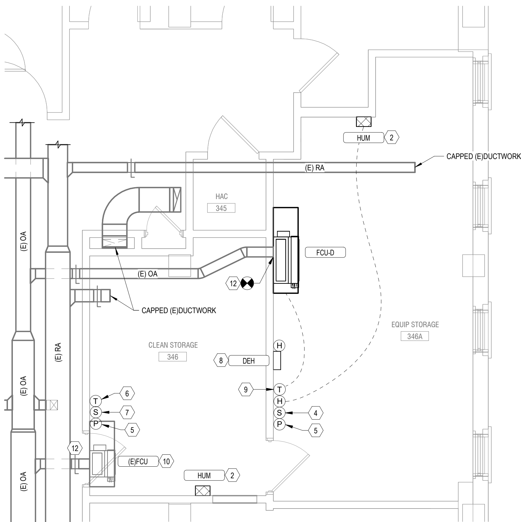
3 Bldg 01-03 THIRD FLOOR HVAC PLAN - ROOM 346 & 346A 1/4" = 1'-0"
