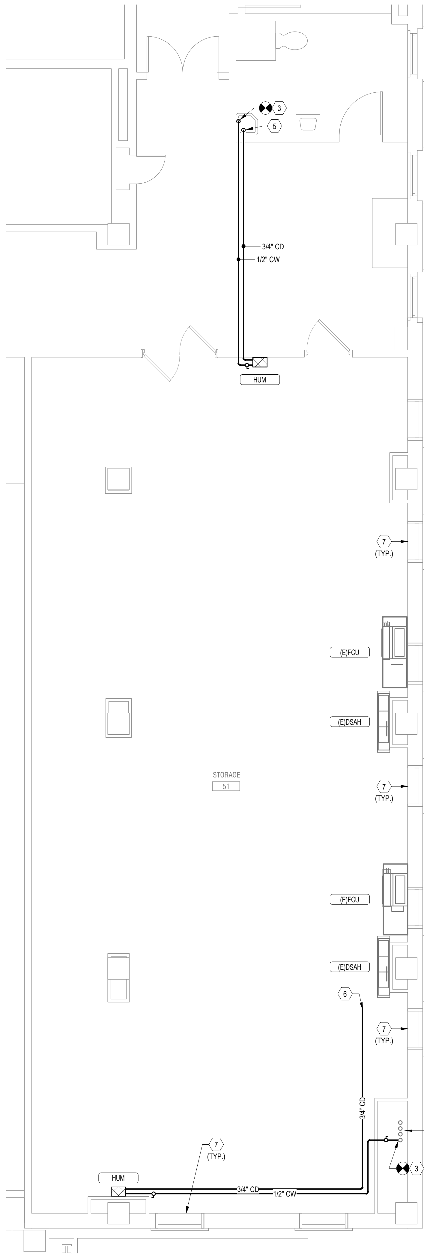
4 Bldg 01-00 BASEMENT FLOOR PIPING PLAN - ROOM 51 1/4\"/>
