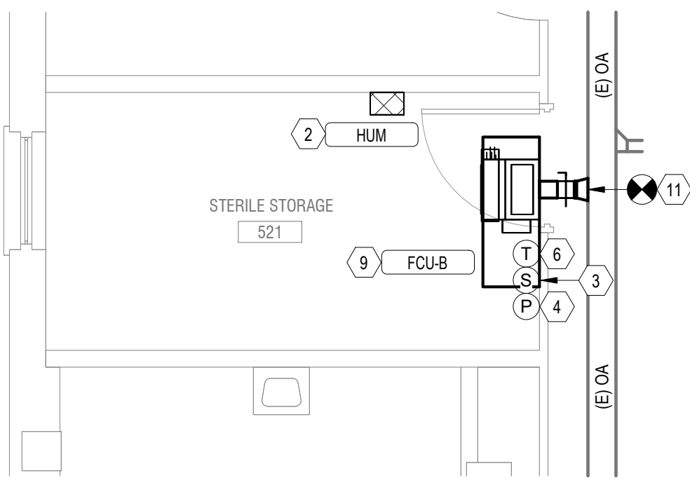
BID DEDUCT 1 - Bldg 17-05 FIFTH FLOOR HVAC PLAN - ROOM 521 1/4" = 1'-0"
