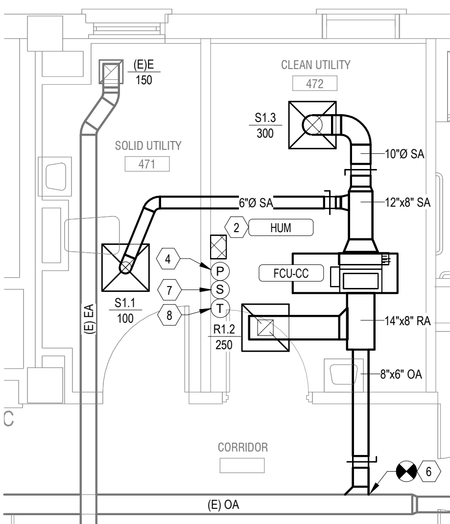
Bldg 01-04 FOURTH FLOOR HVAC PLAN - ROOM 472
