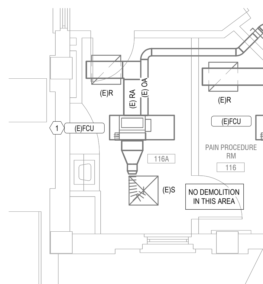
Bldg 01-01 FIRST FLOOR HVAC DEMOLITION PLAN - ROOM 116A
