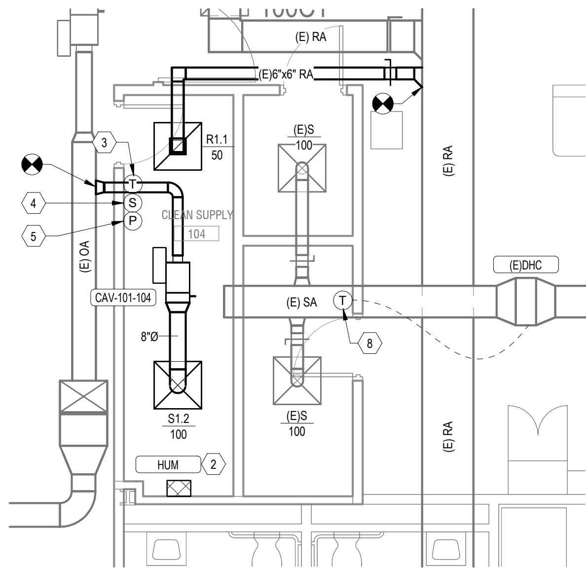
Bldg 101-01-FIRST FLOOR HVAC PLAN - ROOM 104
