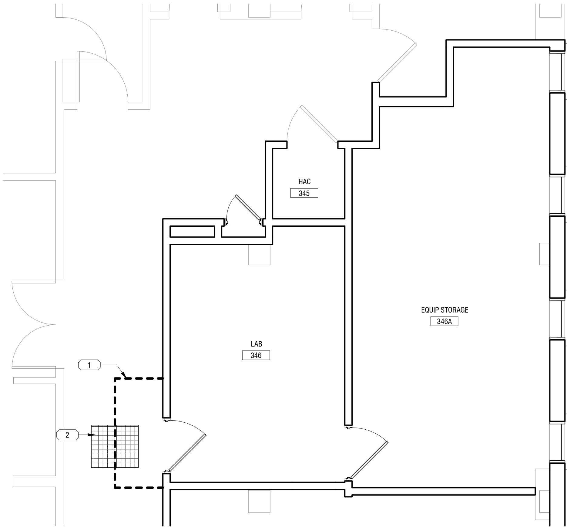
1 Bldg 01-03 THIRD FLOOR - 346 & 346A - ICRA 1/4" = 1'-0"
