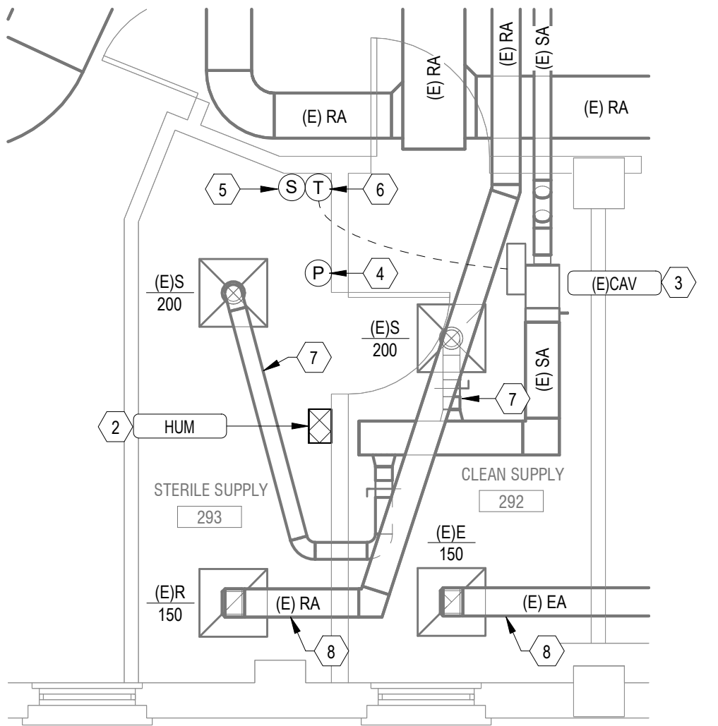
Bldg 01-02 SECOND FLOOR HVAC PLAN - ROOM 293
