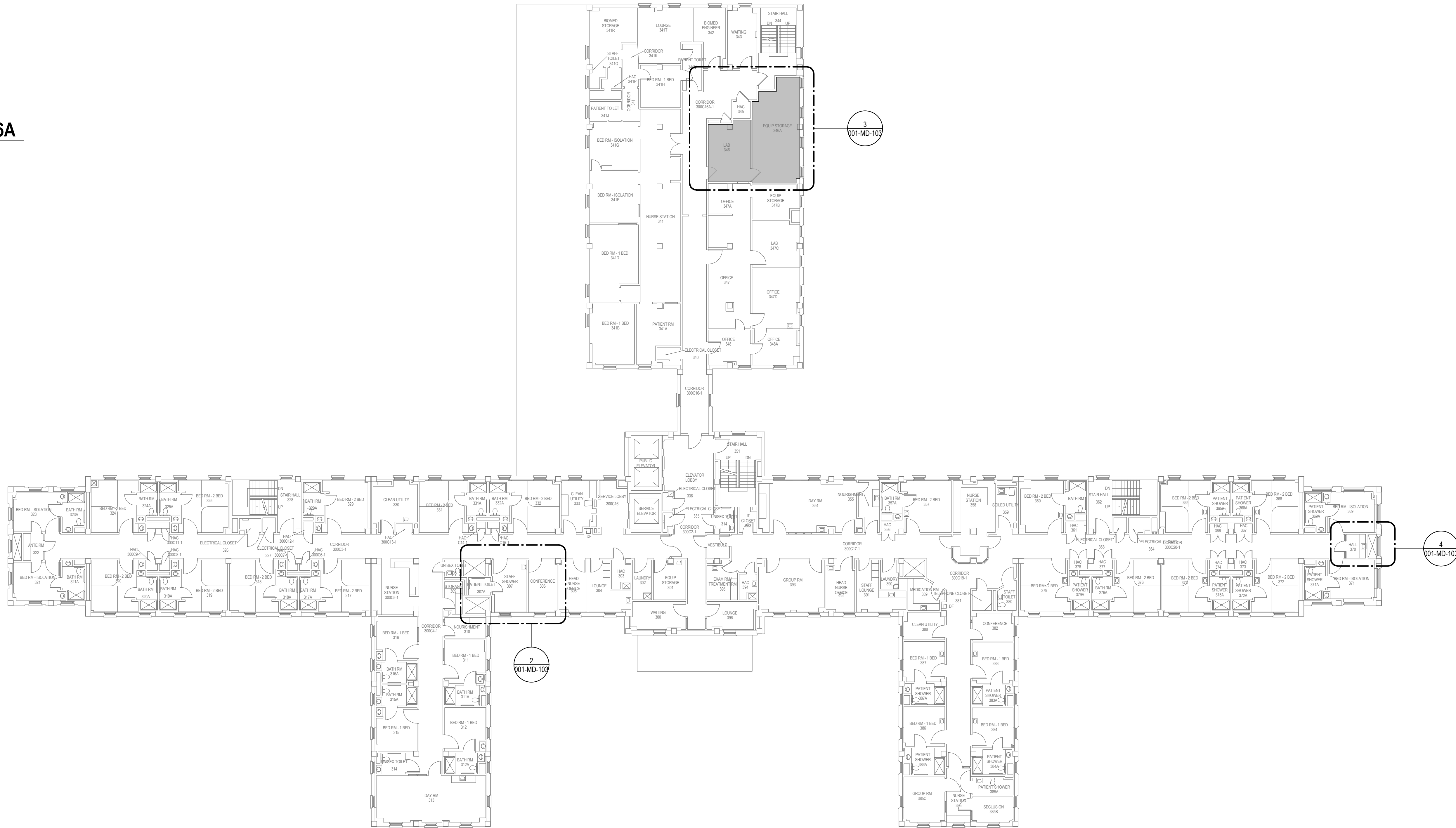
1 Bldg 01-03 THIRD FLOOR HVAC DEMOLITION PLAN 1/16" = 1'-0"
