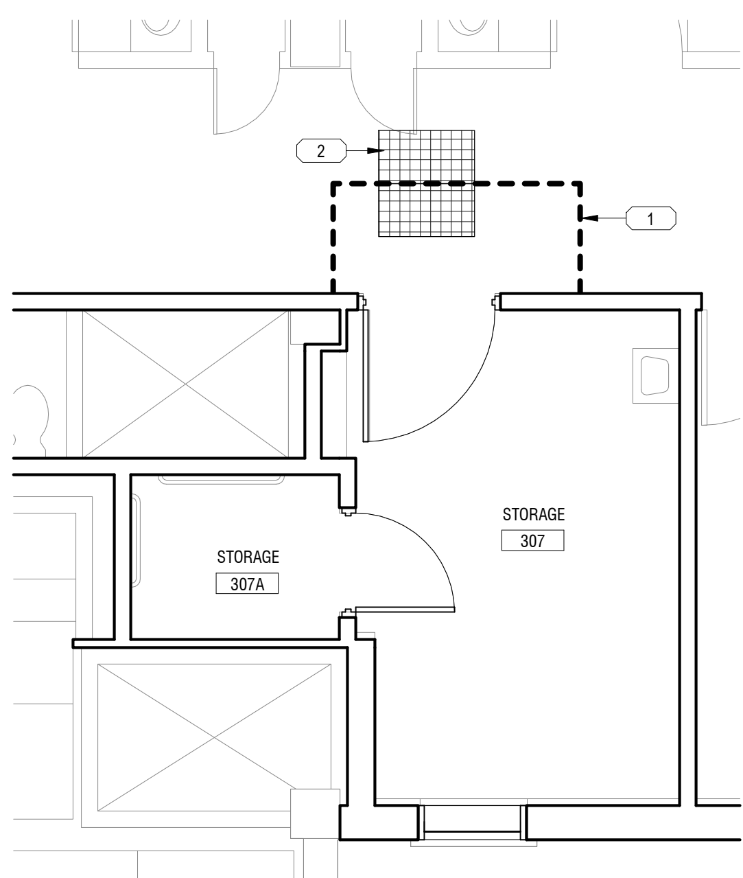
2 Bldg 01-03 THIRD FLOOR - 307 - ICRA 1/4" = 1'-0"
