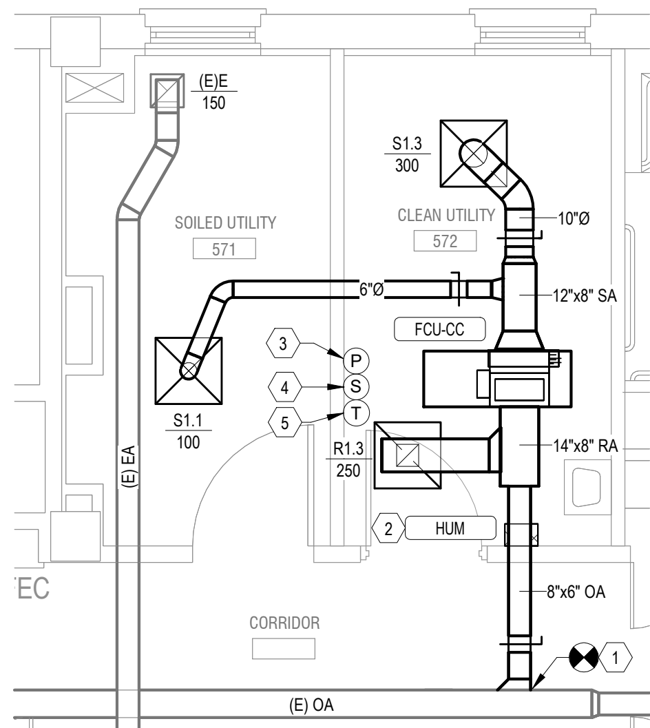
Bldg 01-05 FIFTH FLOOR HVAC PLAN - ROOM 572
