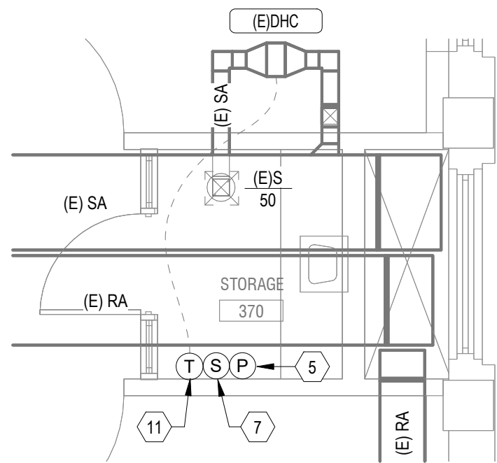
4 Bldg 01-03 THIRD FLOOR HVAC PLAN - ROOM 370 1/4" = 1'-0"
