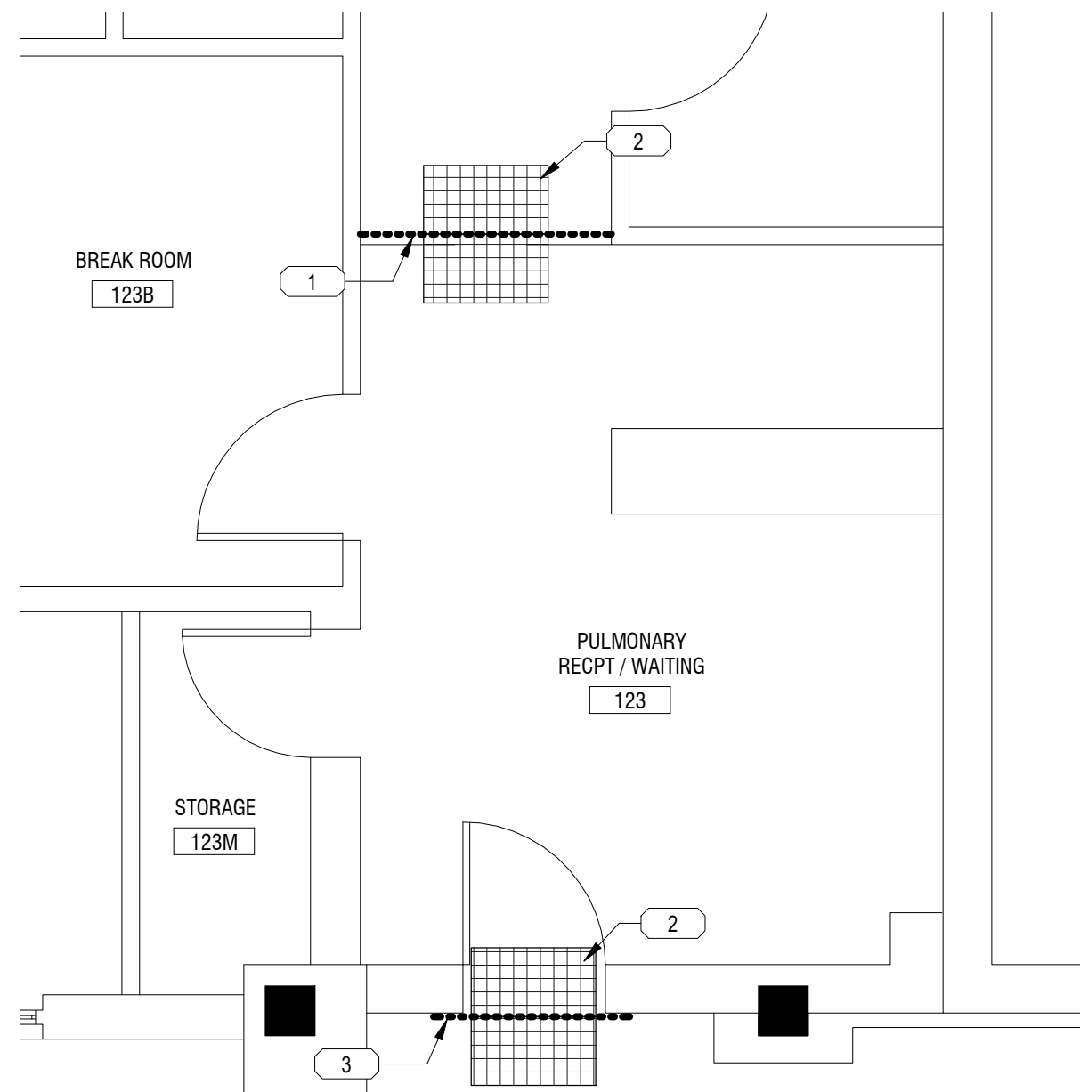
8 Bldg 17-01-FIRST FLOOR - 123M - ICRA 1/4" = 1'-0"
