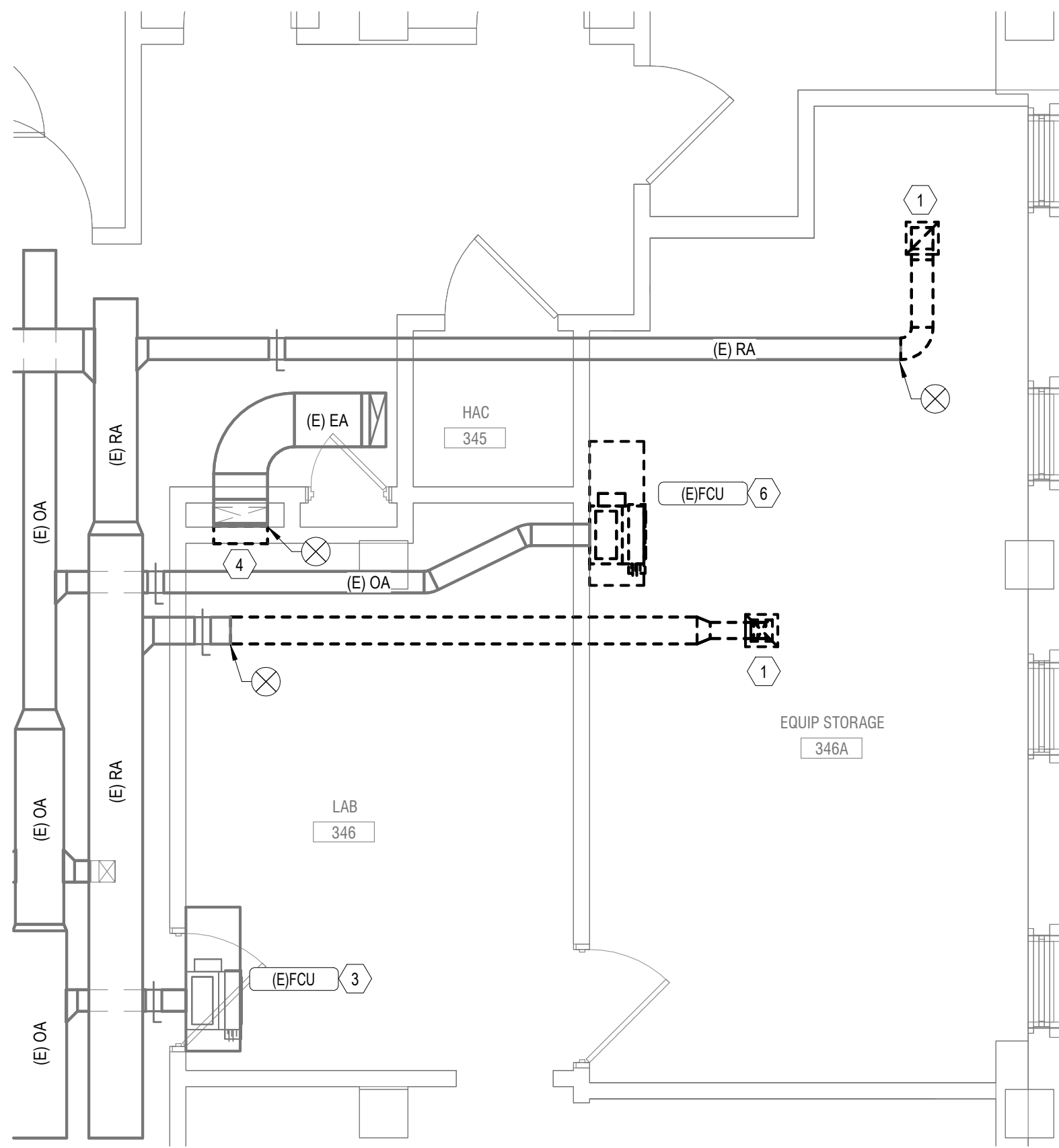
3 Bldg 01-03 THIRD FLOOR HVAC DEMOLITION PLAN - ROOM 346 & 346A 1/4" = 1'-0"
