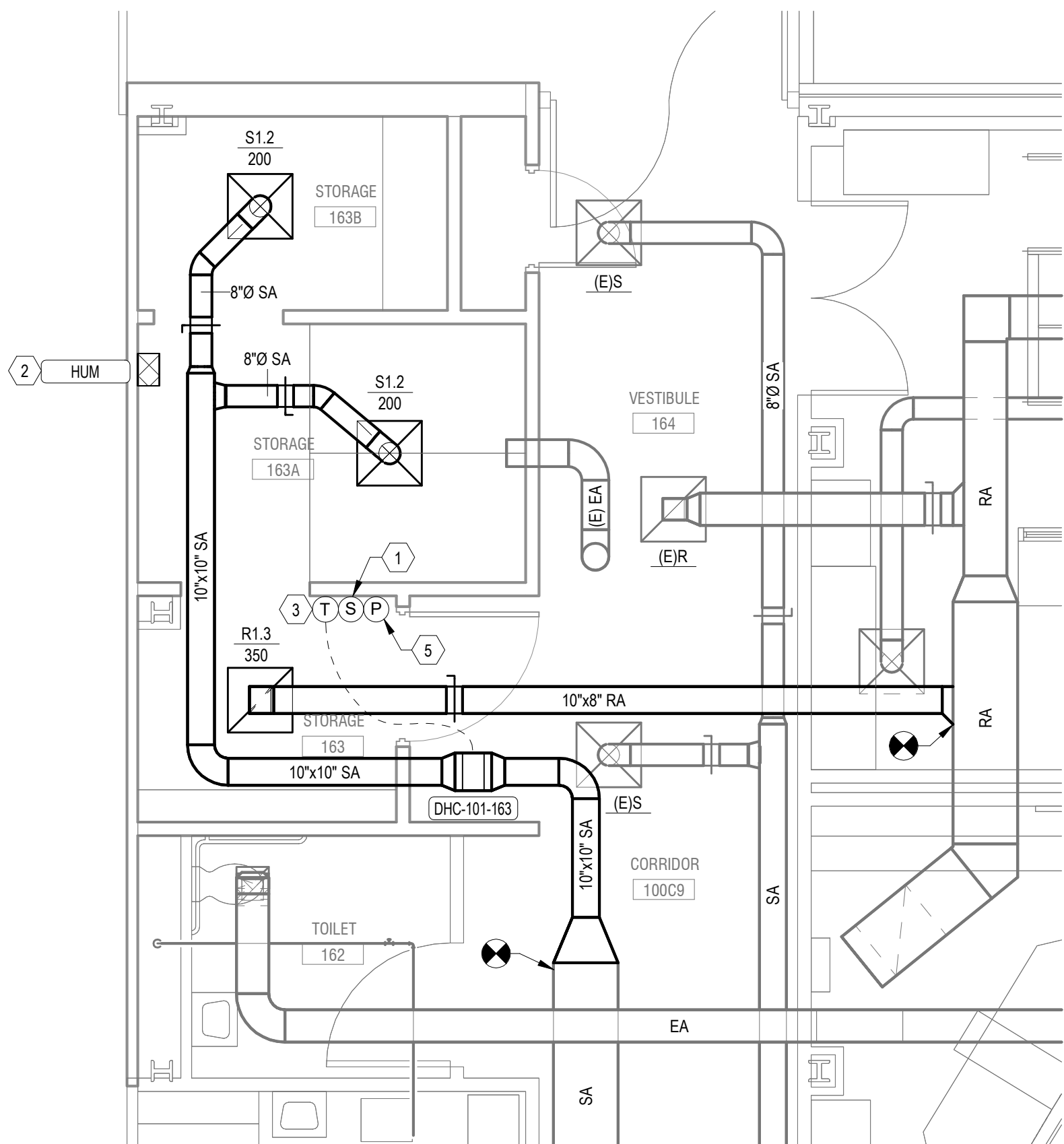
Bldg 101-01-FIRST FLOOR HVAC PLAN - ROOM 163, 163A, 163B
