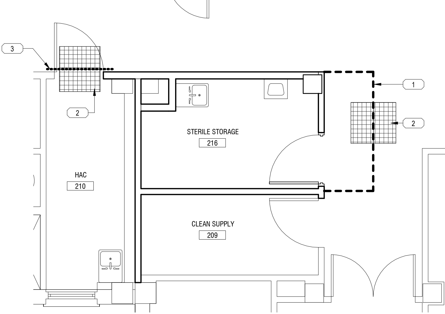
6 Bldg 01-02 SECOND FLOOR - 216 - ICRA 1/4" = 1'-0"
