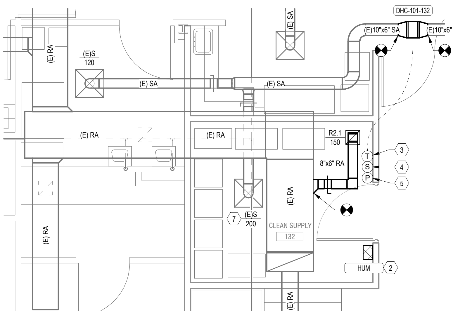
Bldg 101-01-FIRST FLOOR HVAC PLAN - ROOM 132
