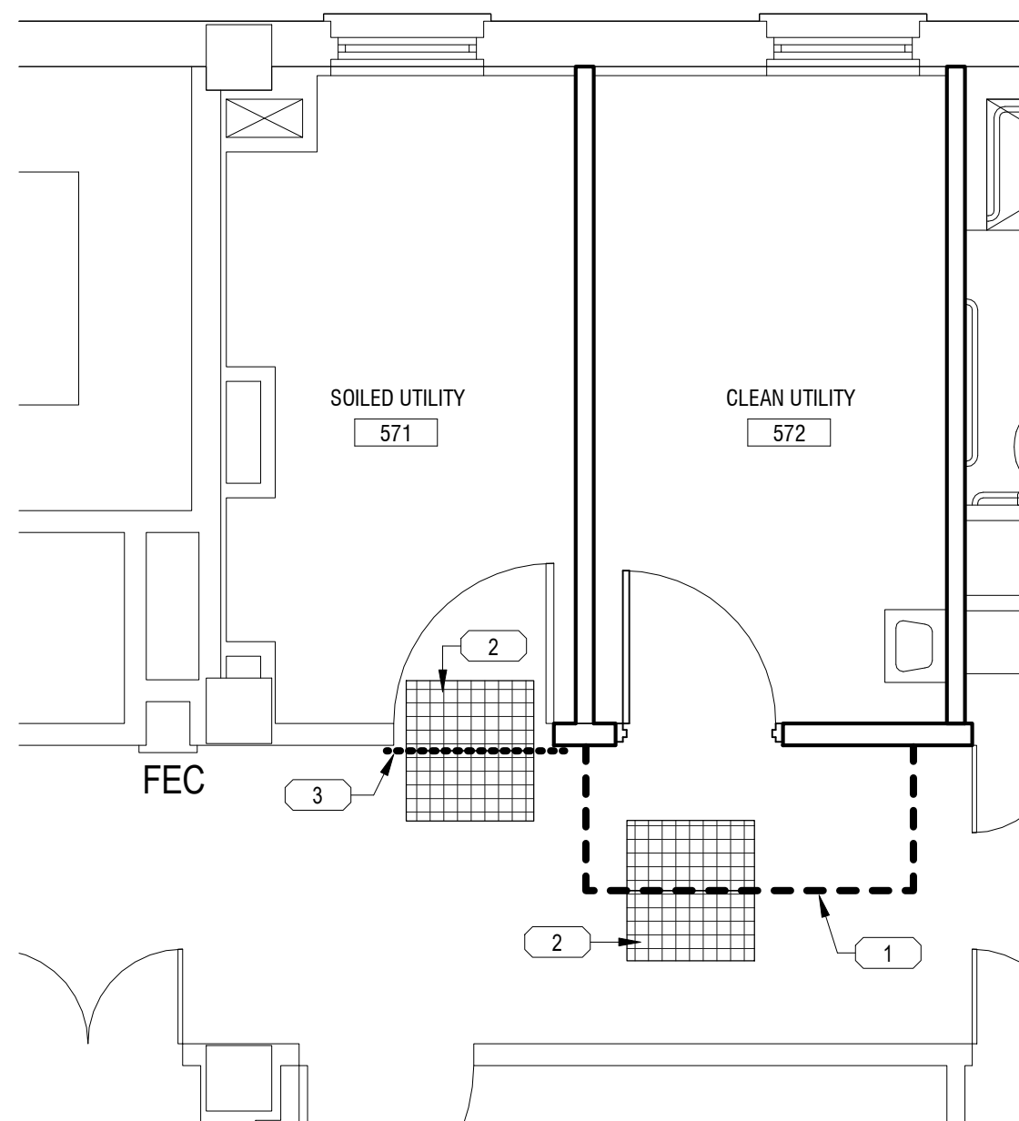
6 Bldg 01-05 FIFTH FLOOR - 572 - ICRA 1/4" = 1'-0"
