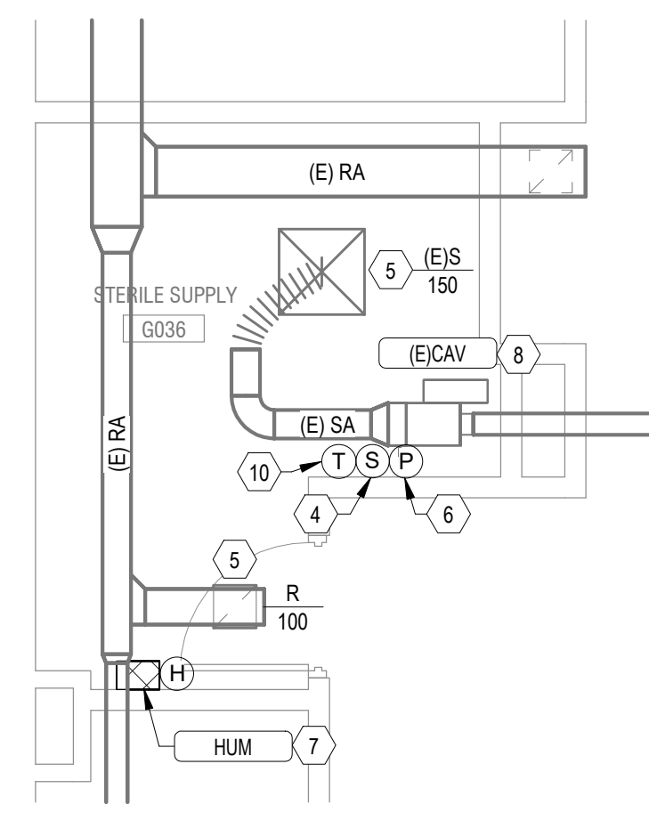
Bldg 01-00 BASEMENT FLOOR HVAC PLAN - ROOM G036
