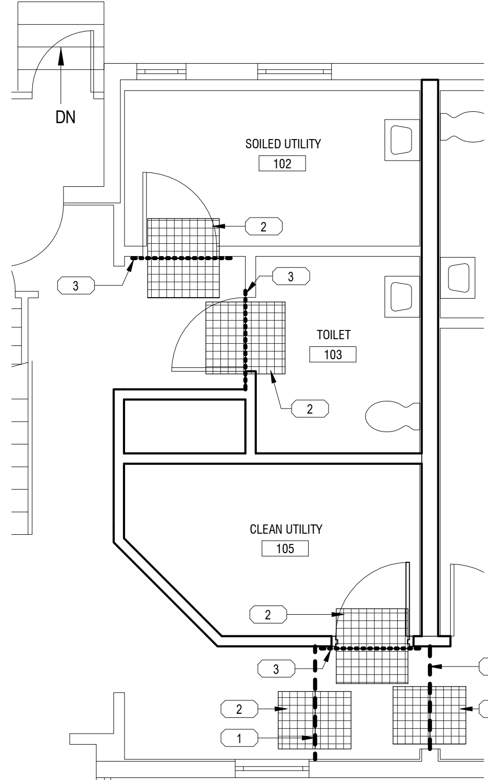
7 Bldg 04-01 FIRST FLOOR - 105 - ICRA 1/4" = 1'-0"
