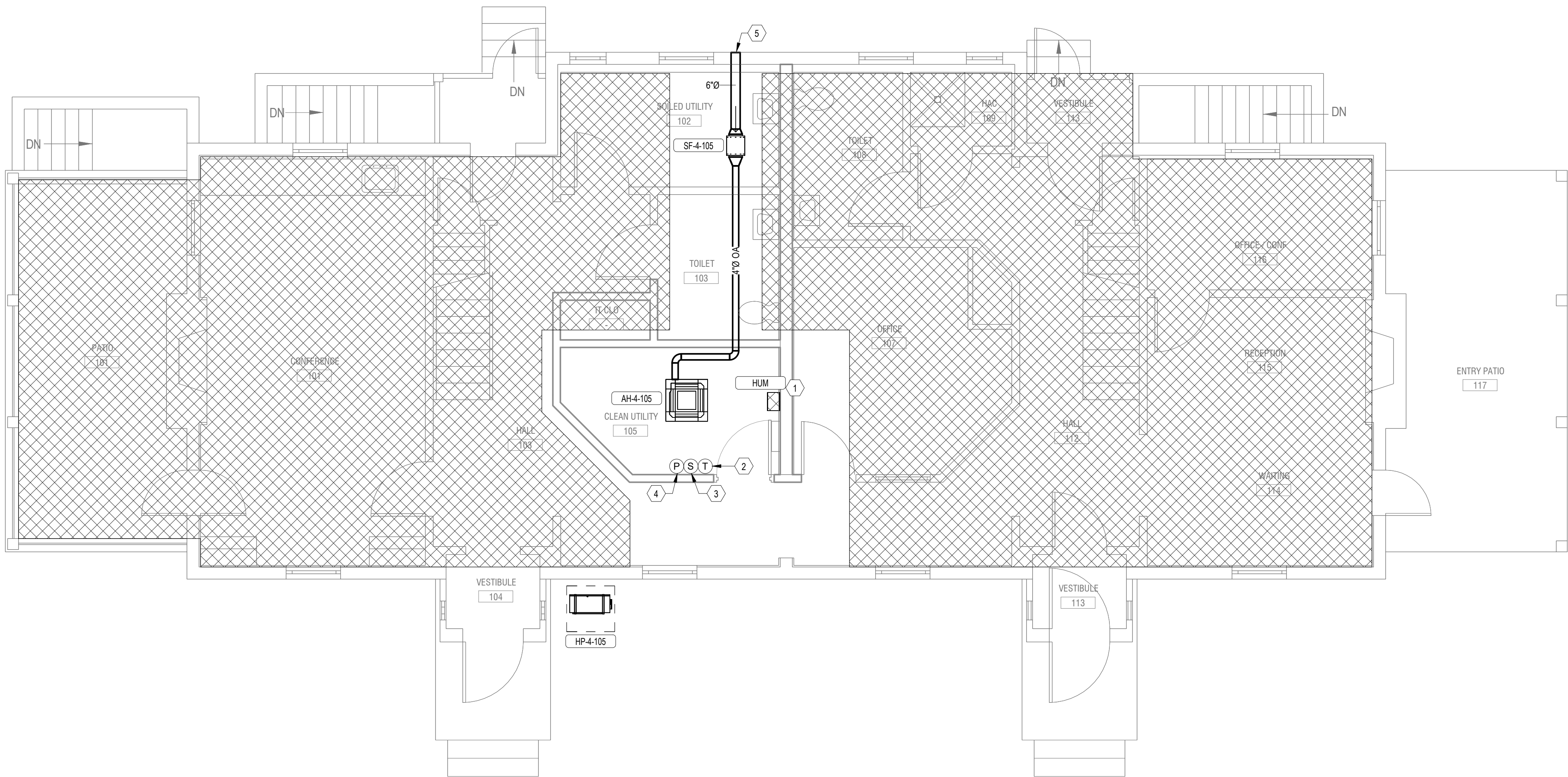
1 Bldg 04-01 FIRST FLOOR HVAC PLAN - ROOM 105 1/4" = 1'-0"
