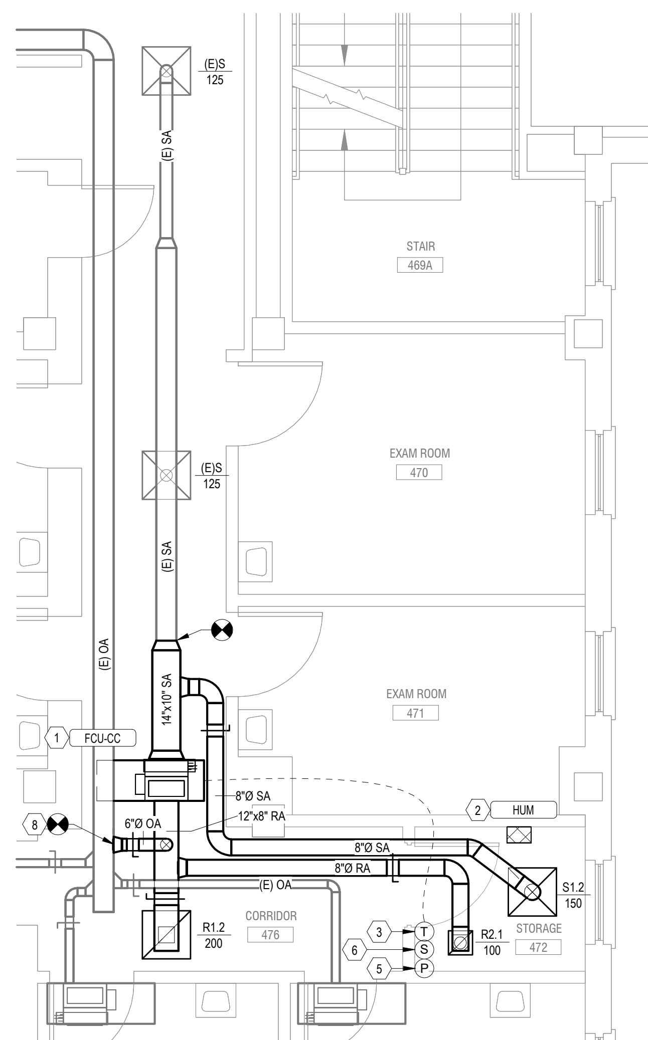
BID DEDUCT 1 - Bldg 17-04 FOURTH FLOOR HVAC PLAN - ROOM 472 1/4" = 1'-0"
