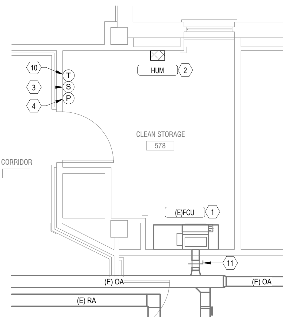
BID DEDUCT 1 - Bldg 17-05 FIFTH FLOOR HVAC PLAN - ROOM 578 1/4" = 1'-0"
