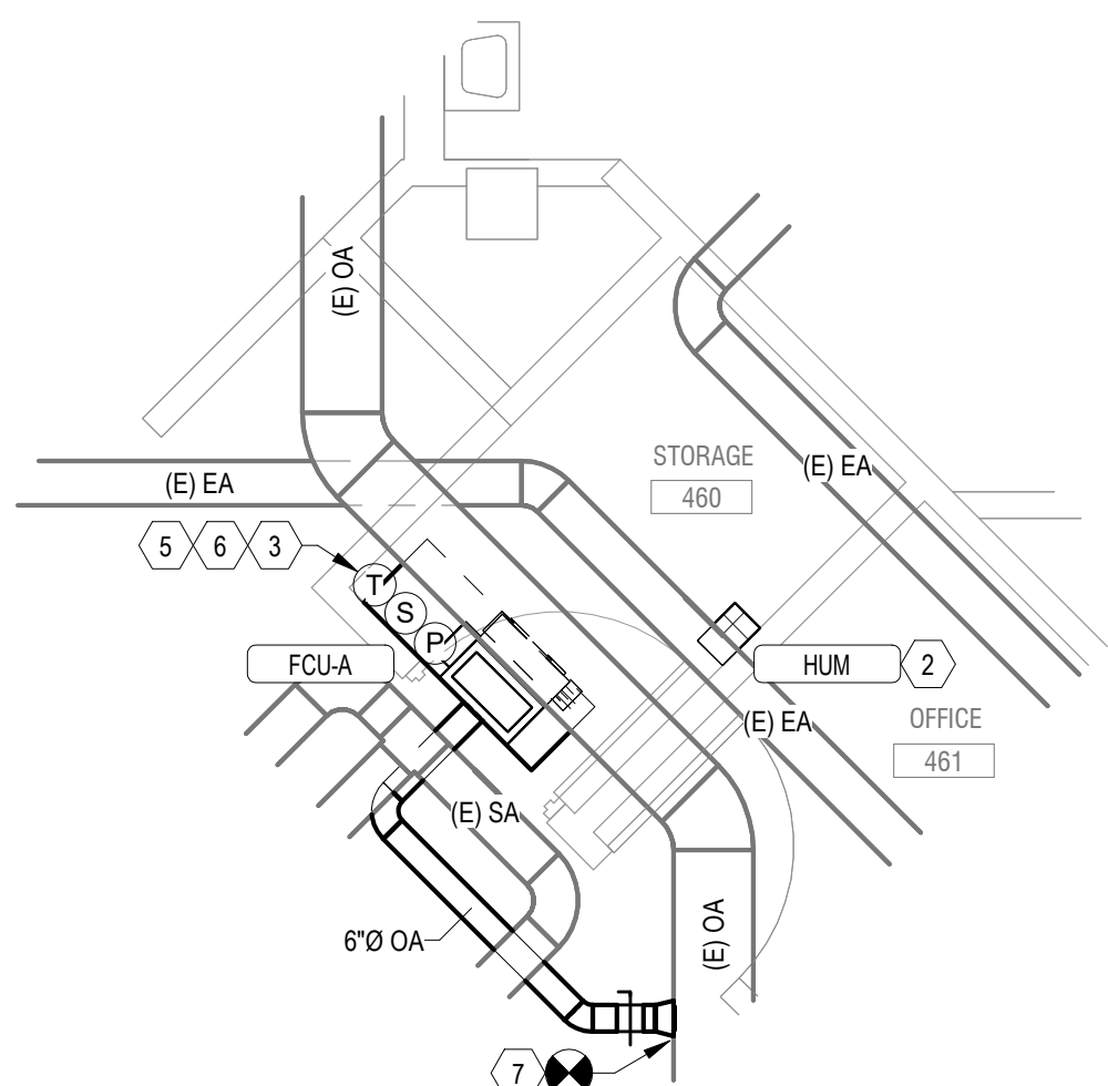
BID DEDUCT 1 - Bldg 17-04 FOURTH FLOOR HVAC PLAN - ROOM 460 1/4" = 1'-0"
