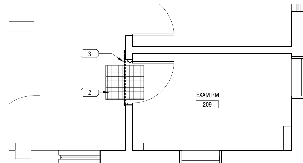
BID DEDUCT 1- Bldg 17-02-SECOND FLOOR - 209 - ICRA 1/4" = 1'-0"
