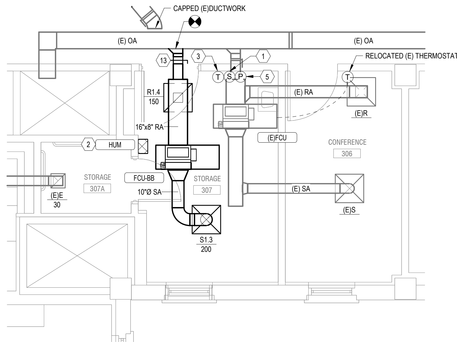
2 Bldg 01-03 THIRD FLOOR HVAC PLAN - ROOM 307 1/4" = 1'-0"
