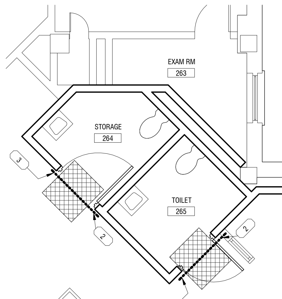
BID DEDUCT 1- Bldg 17-02-SECOND FLOOR - 264 - ICRA 1/4" = 1'-0"
