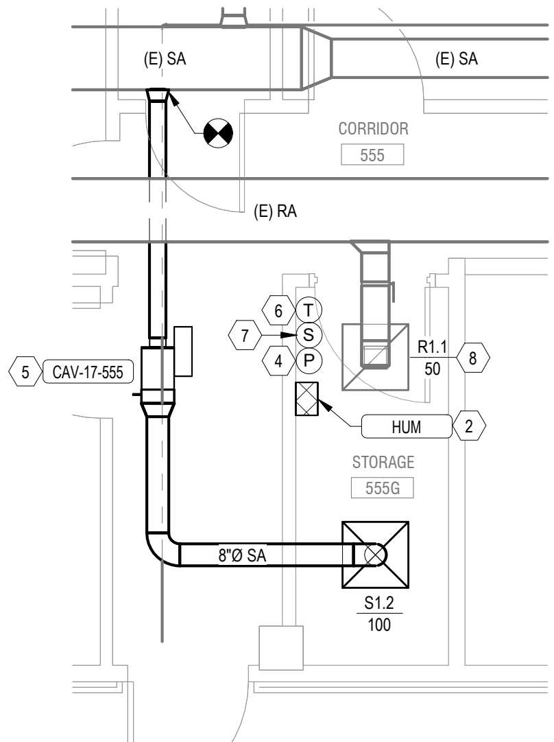
BID DEDUCT 1 - Bldg 17-05 FIFTH FLOOR HVAC PLAN - ROOM 555G 1/4" = 1'-0"
