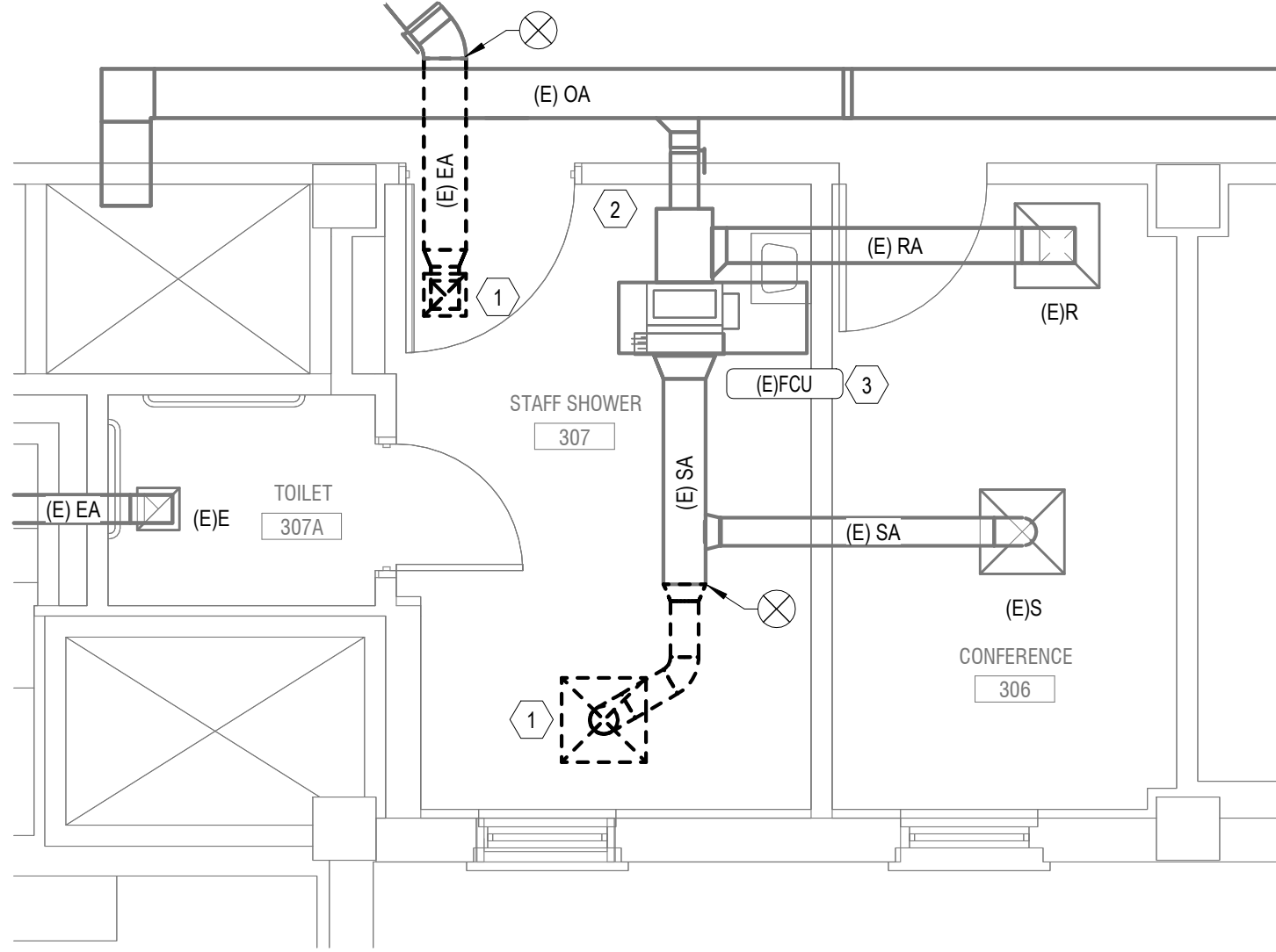
2 Bldg 01-03 THIRD FLOOR HVAC DEMOLITION PLAN - ROOM 307 1/4" = 1'-0"
