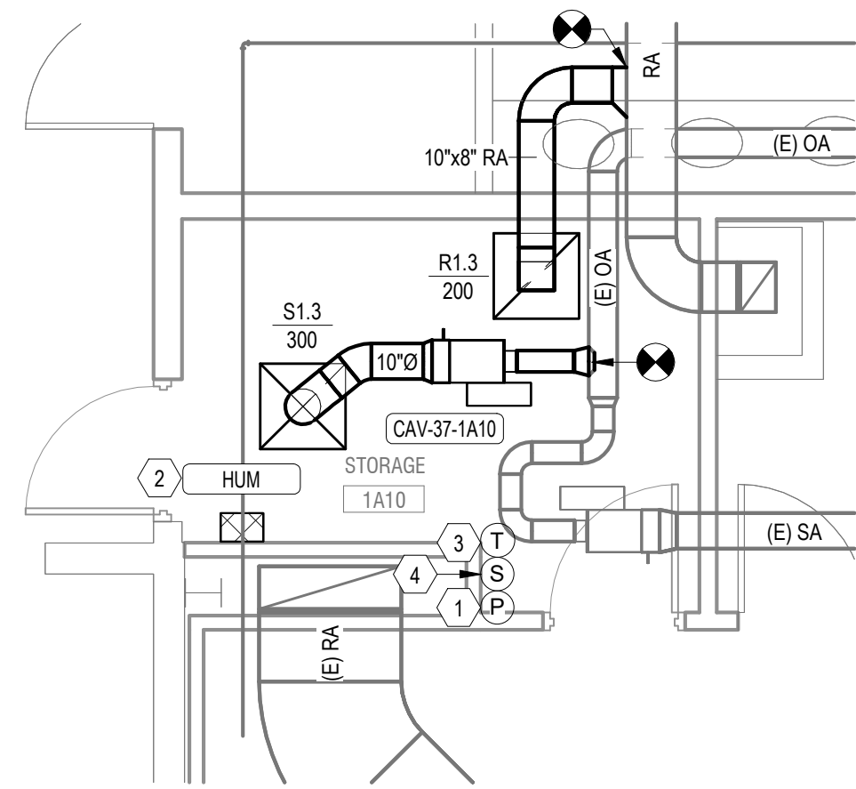
Bldg 37-01-FIRST FLOOR HVAC PLAN - ROOM 1A10
