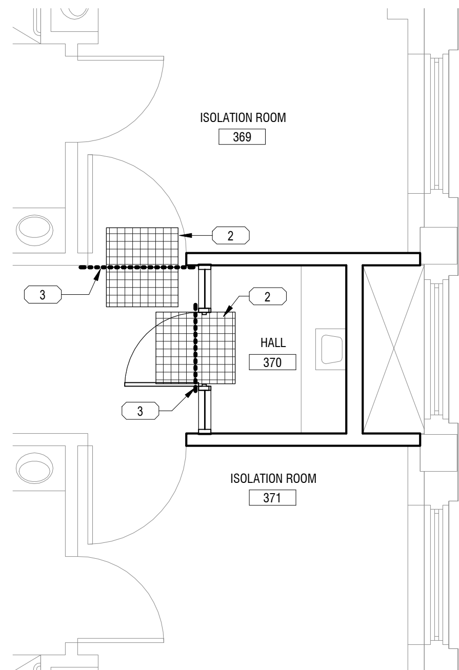
3 Bldg 01-03 THIRD FLOOR - 370 - ICRA 1/4" = 1'-0"
