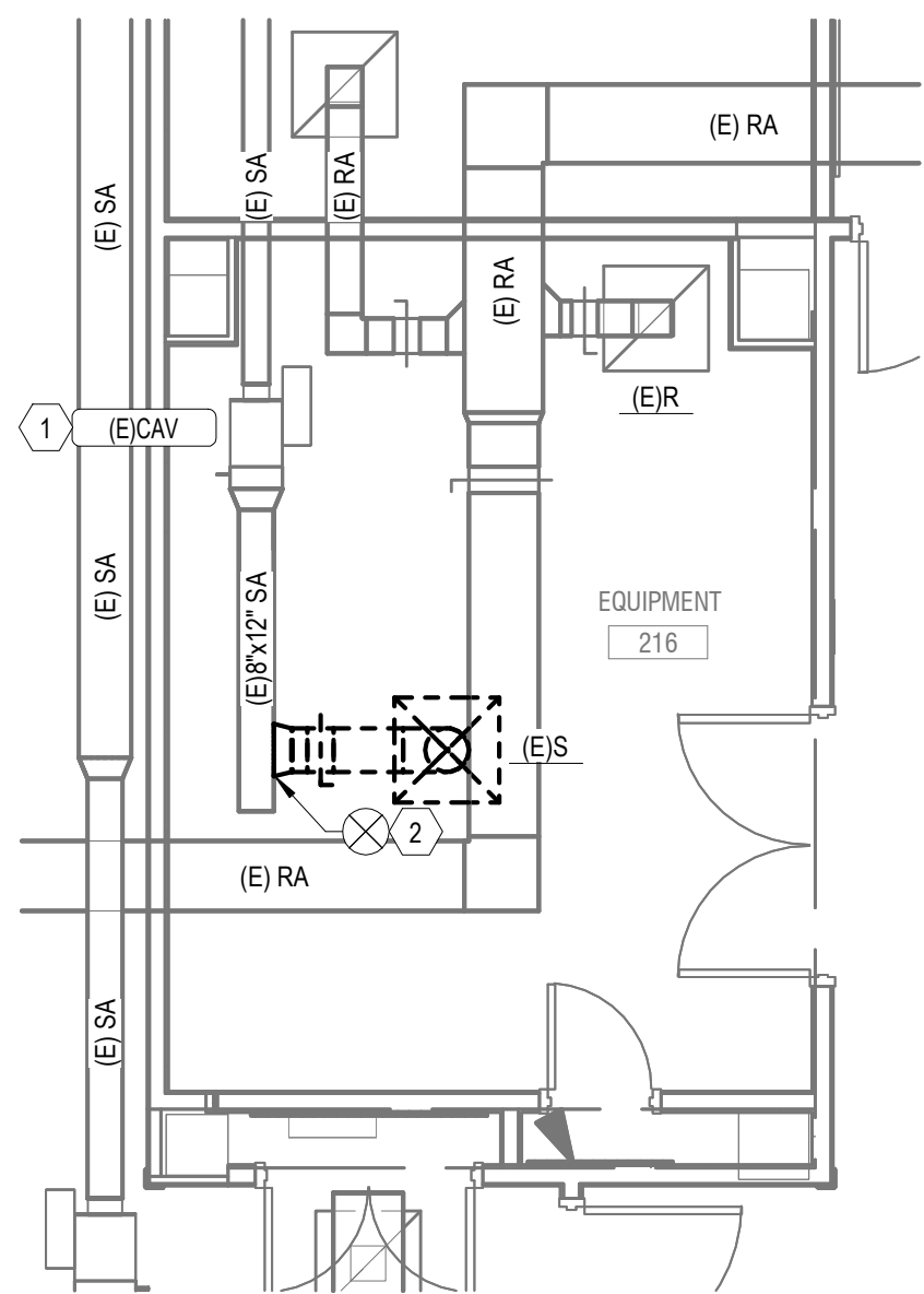
Bldg 22-02-SECOND FLOOR HVAC DEMOLITION PLAN - ROOM 216
