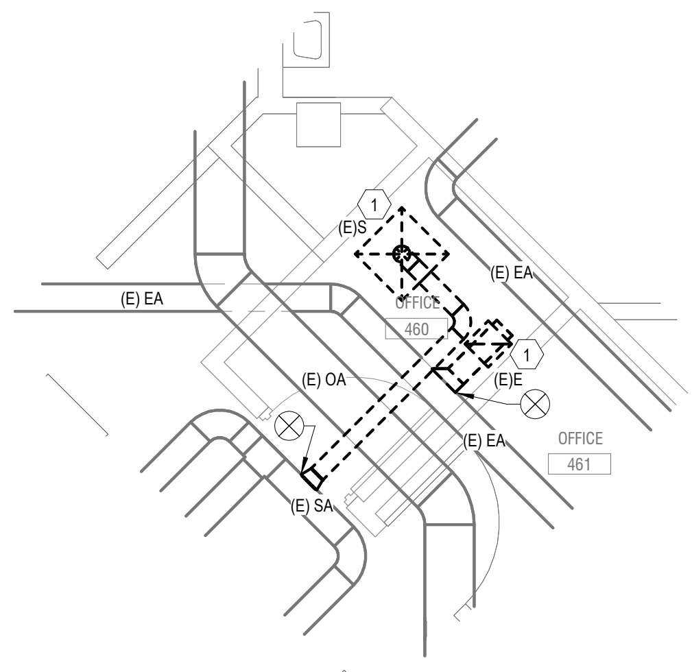
BID DEDUCT 1 - Bldg 17-04 FOURTH FLOOR HVAC DEMOLITION PLAN - ROOM 460
