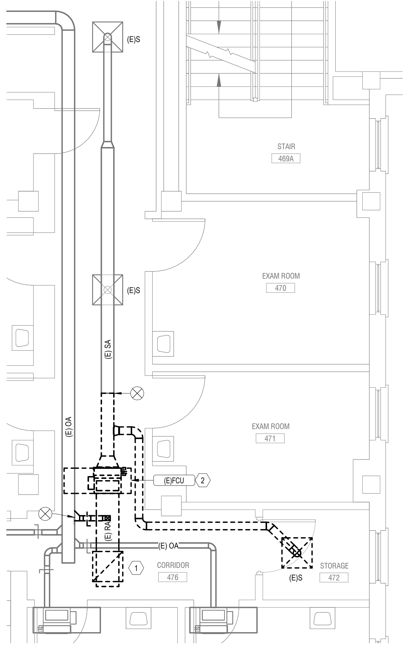
BID DEDUCT 1 - Bldg 17-04 FOURTH FLOOR HVAC DEMOLITION PLAN - ROOM 472
