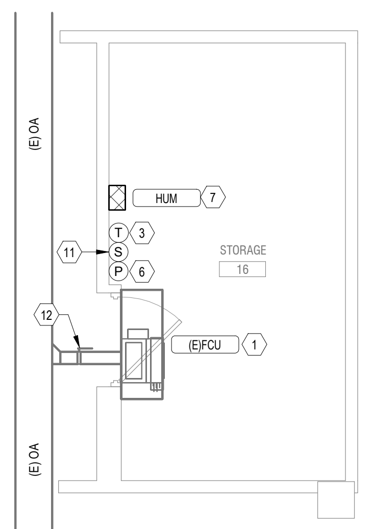
Bldg 01-00 BASEMENT FLOOR HVAC PLAN - ROOM 16
