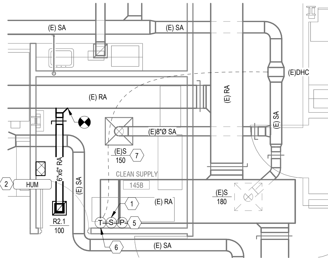
Bldg 101-01-FIRST FLOOR HVAC PLAN - ROOM 145B
