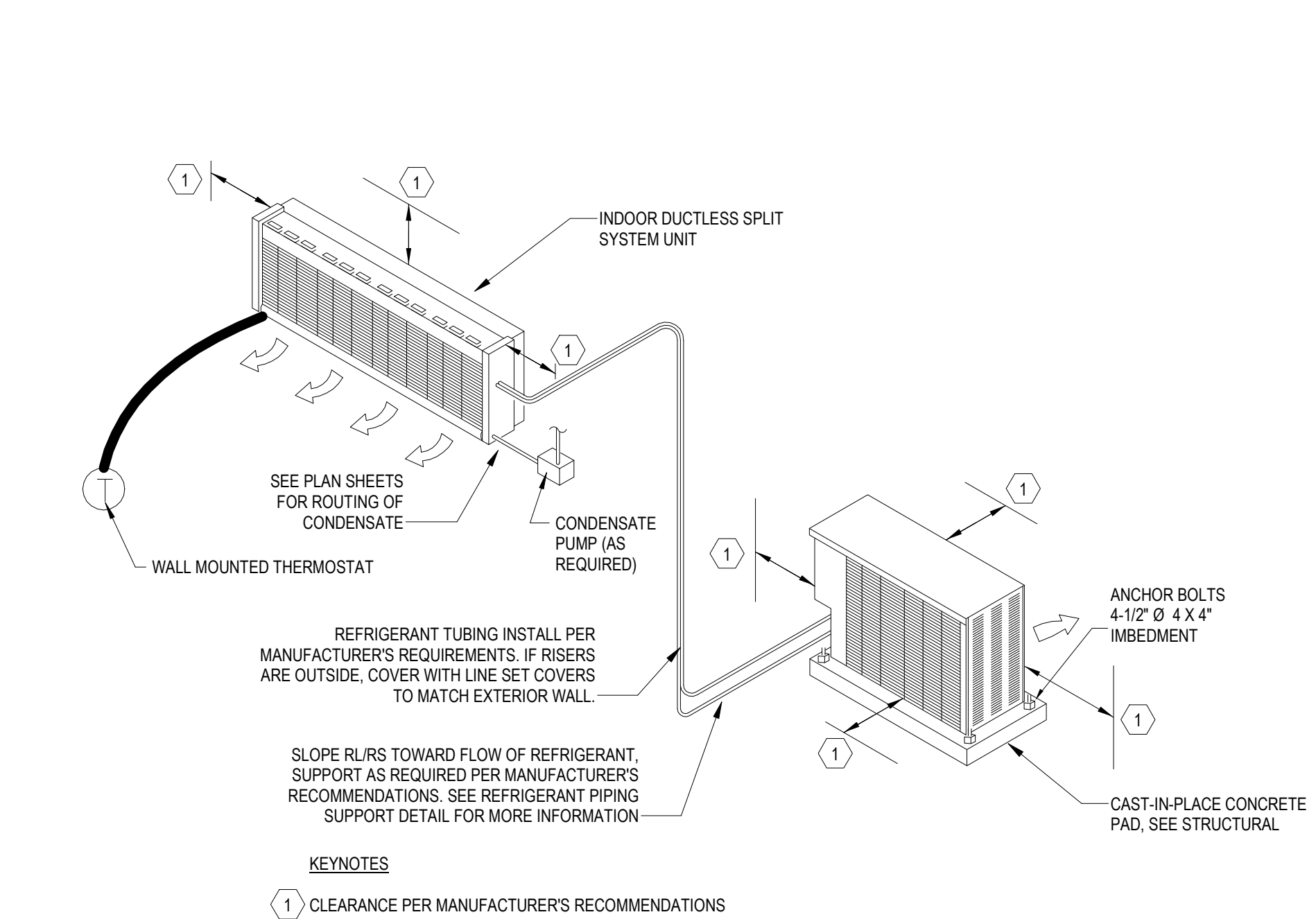
1 GROUND MOUNTED DUCTLESS SPLIT SYSTEM
