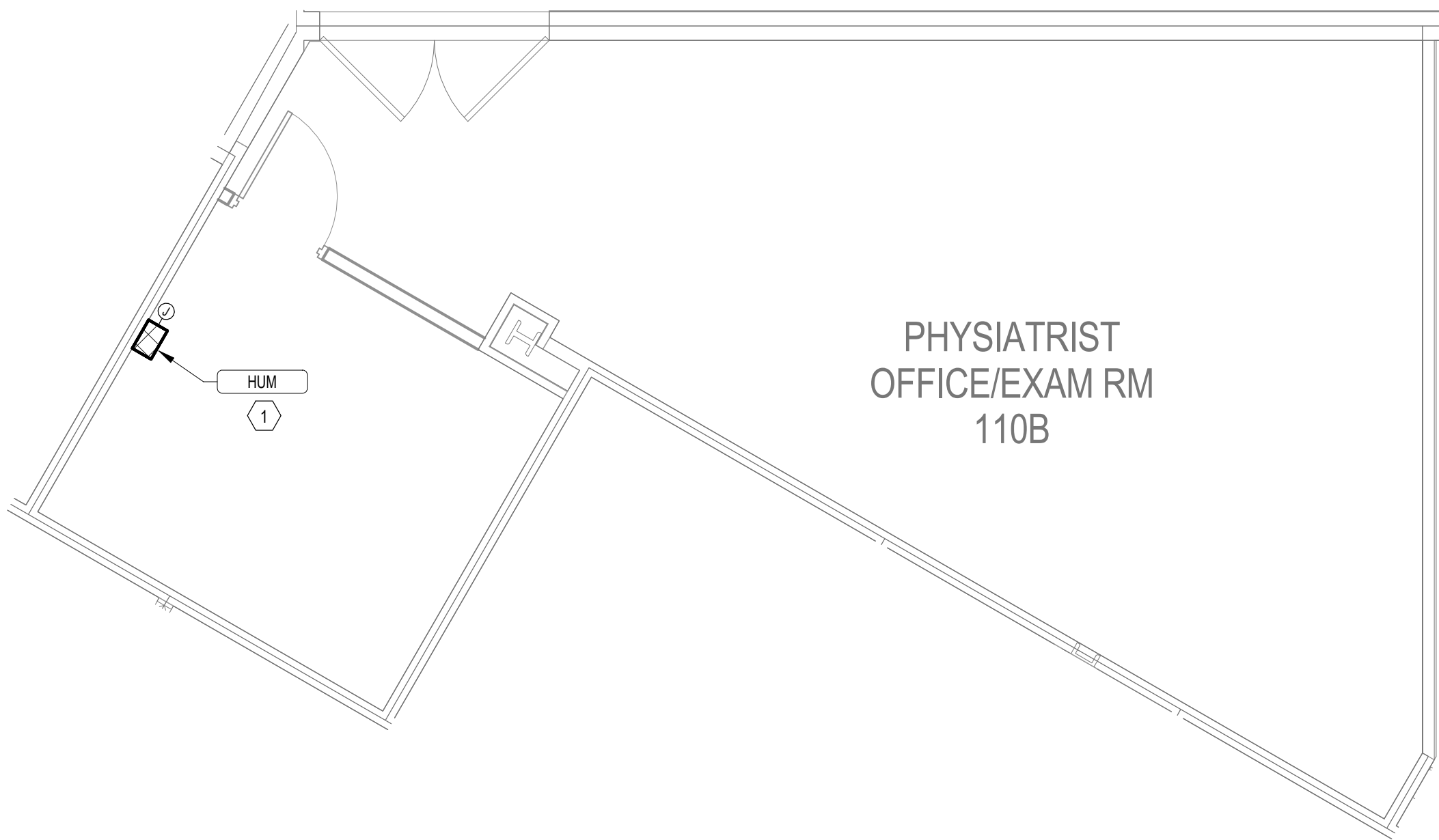
2 BLDG 102-01 FIRST FLOOR ELECTRICAL PLAN - ROOM 110 1/4" = 1'-0"
