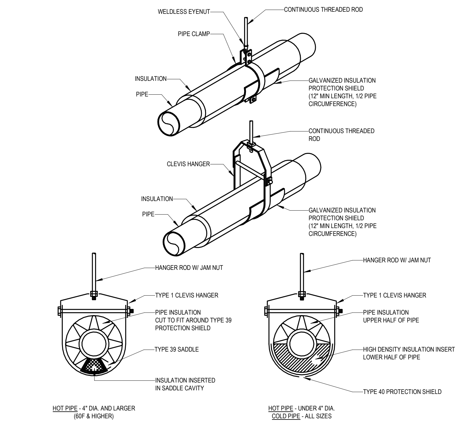
5 PIPE CLEVIS HANGER
