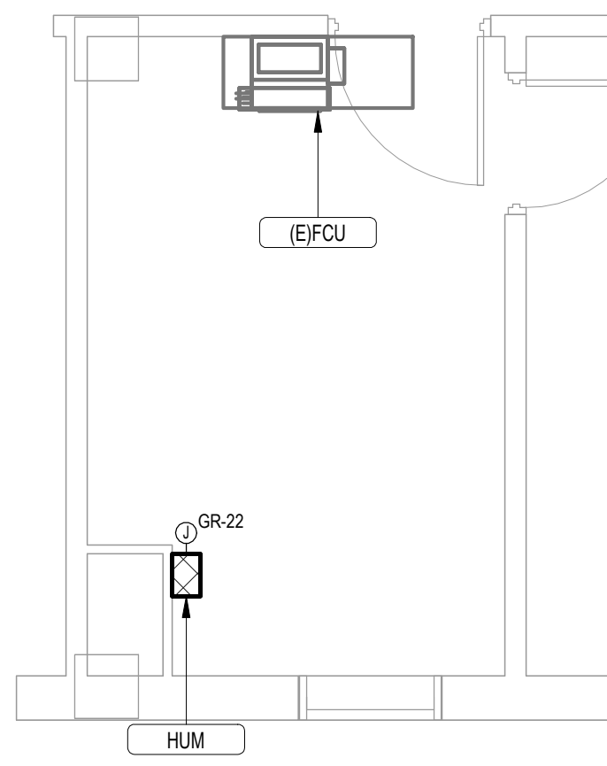
2 BLDG 01-01 FIRST FLOOR ELECTRICAL PLAN - ROOM 111 1/4" = 1'-0"
