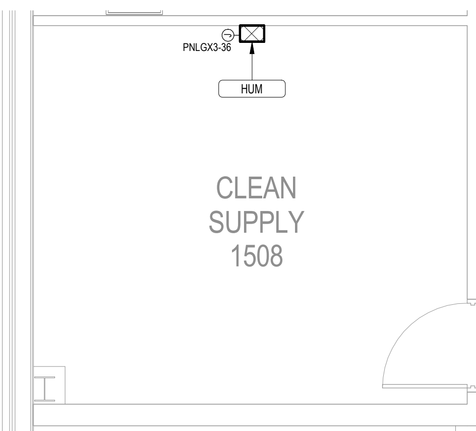
BLDG 104-01 FIRST FLOOR ELECTRICAL PLAN - ROOM 1508
