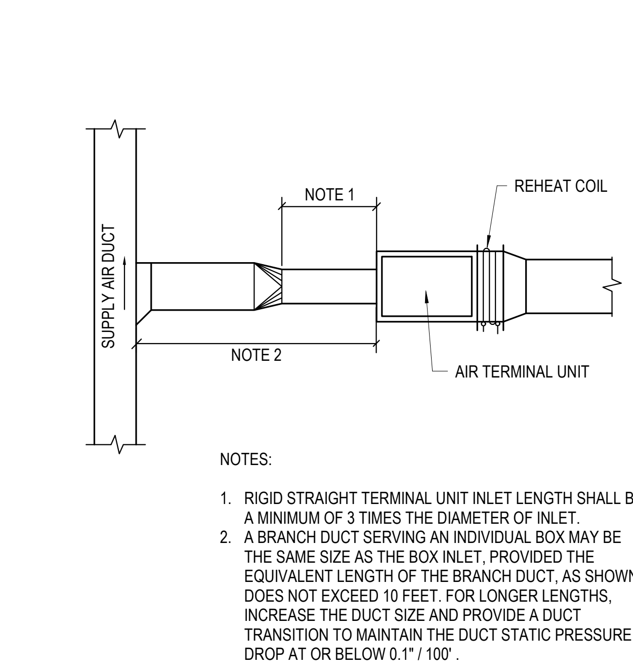
3 VAV/CAV AIR TERMINAL UNITS
