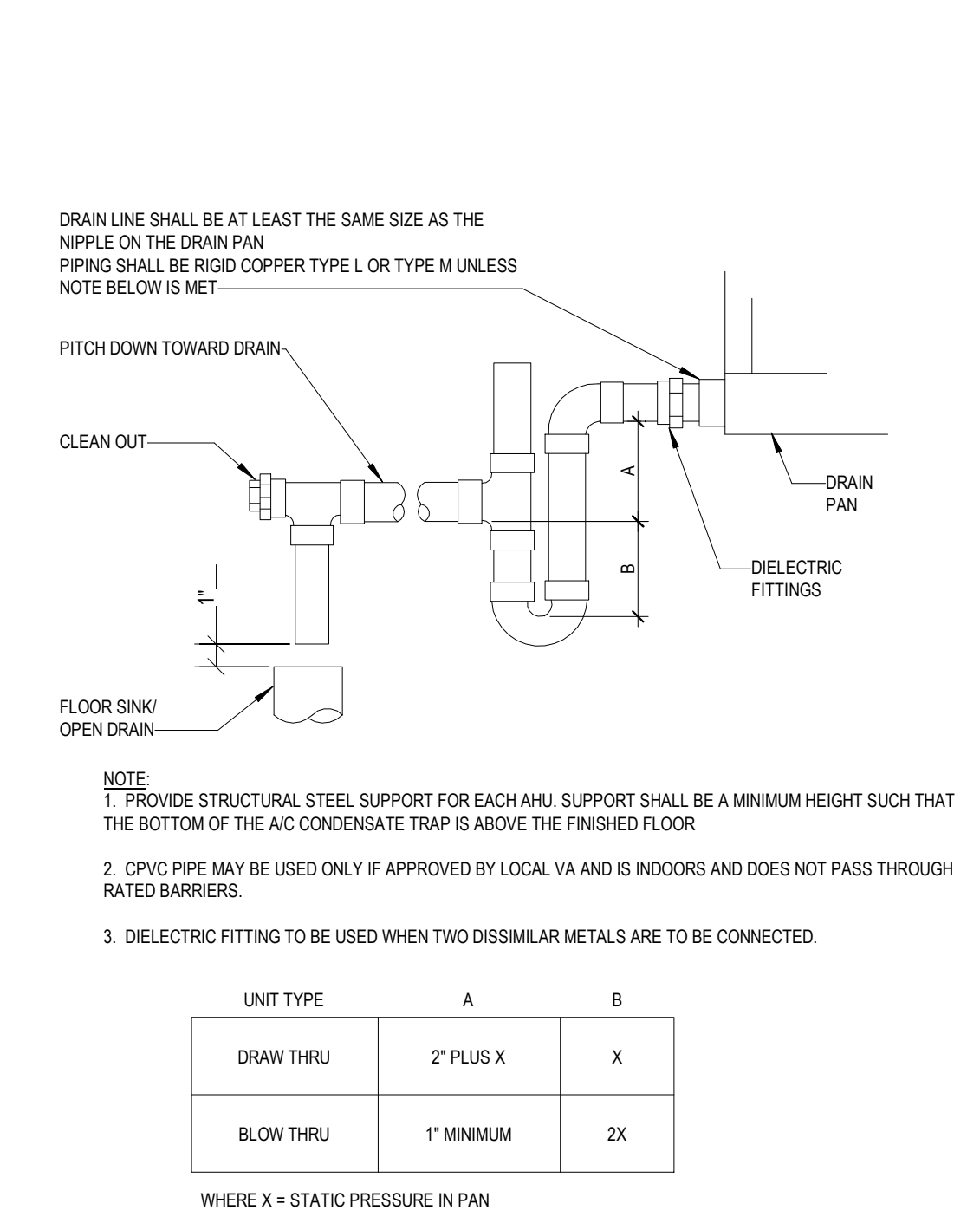
6 CONDENSATE DRAIN TRAP DETAIL
