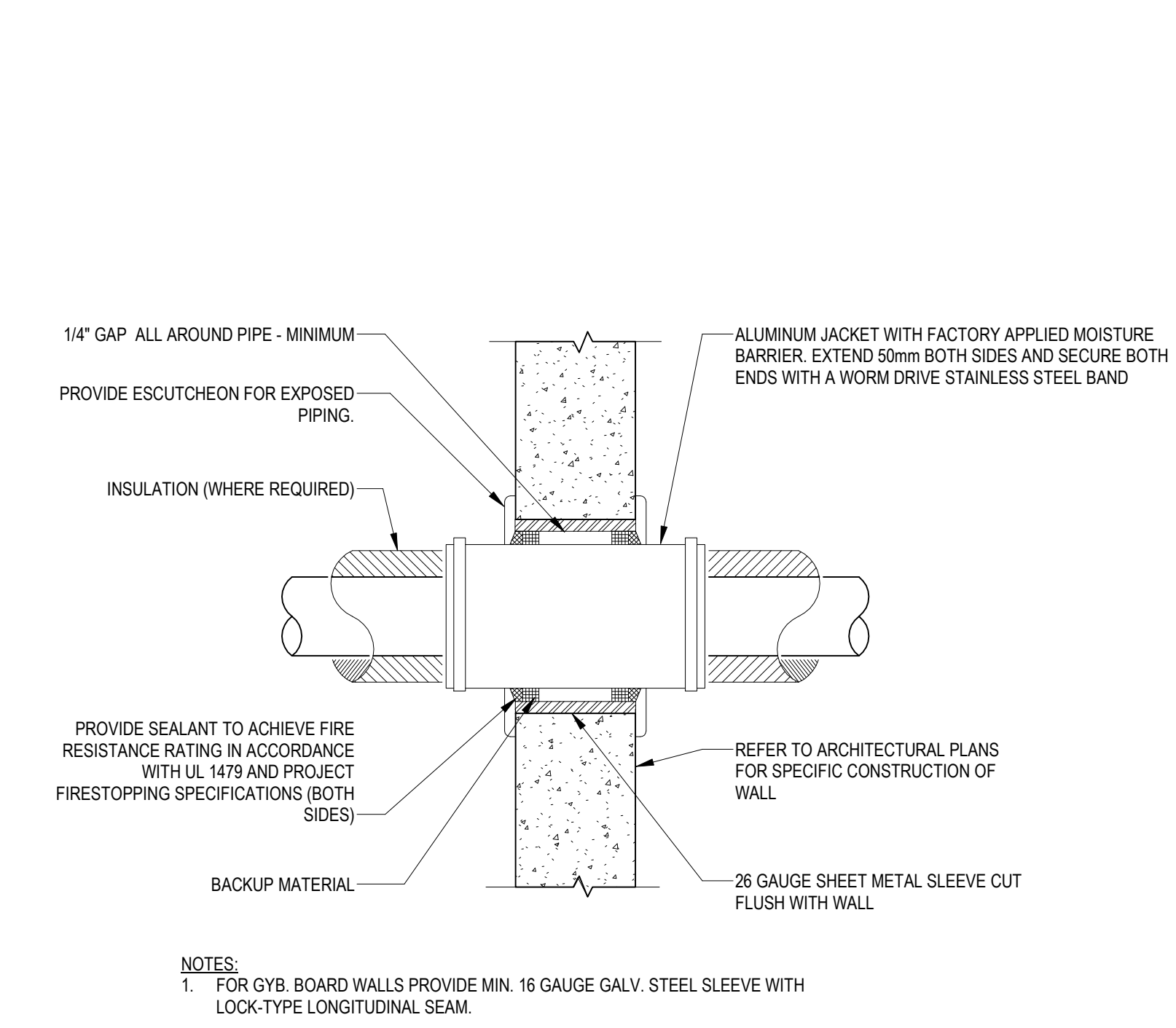
7 EXTERIOR PIPE WALL PENETRATION DETAIL
