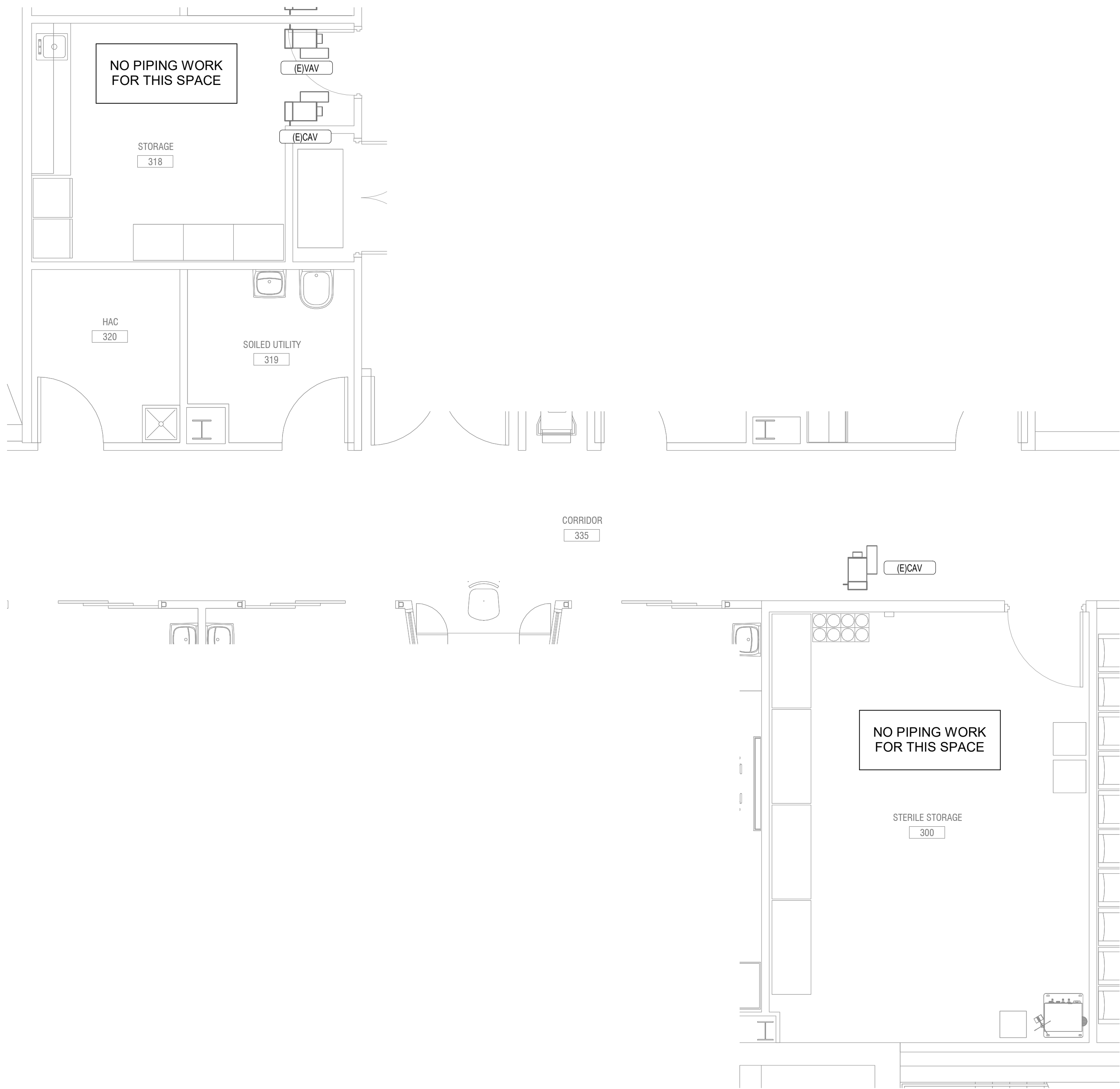
2 Bldg 104-03 THIRD FLOOR PIPING PLAN - ROOM 300 & 318 1/4" = 1'-0"
