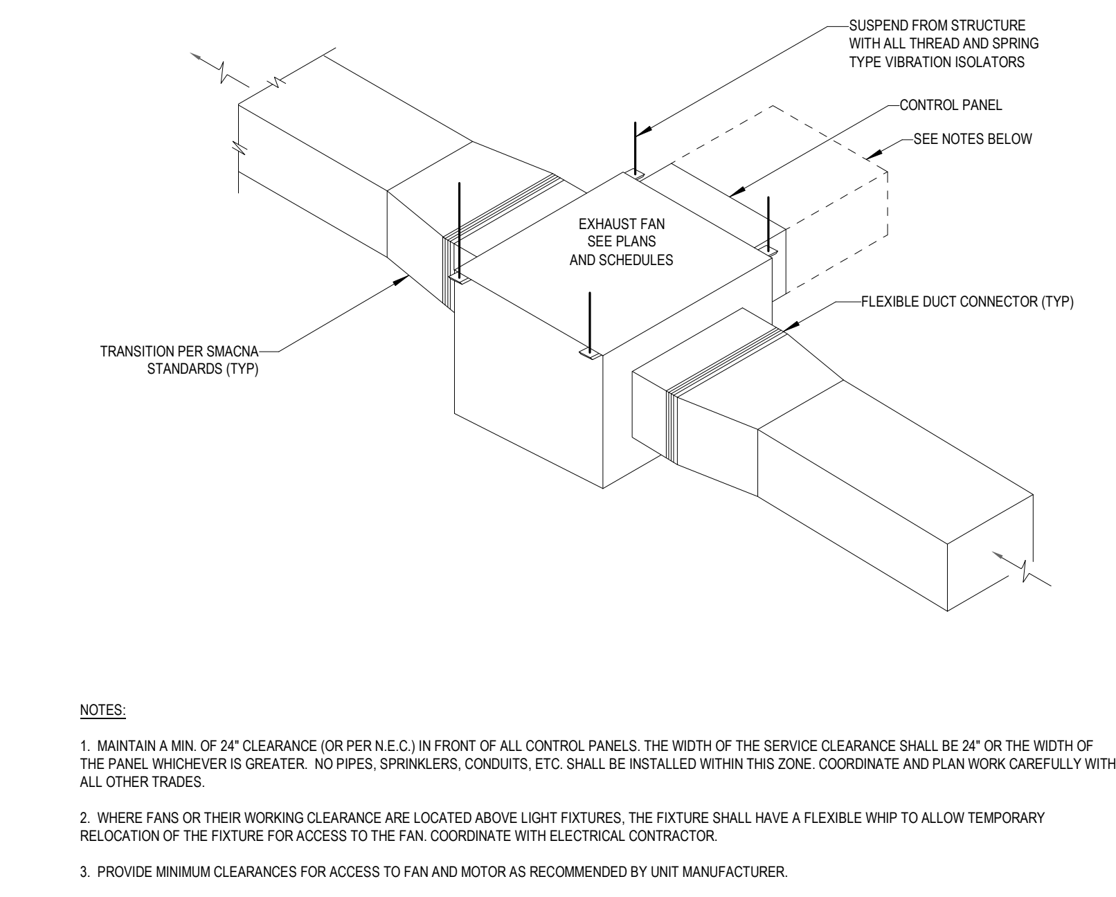
2 IN-LINE FAN HANGING DETAIL
