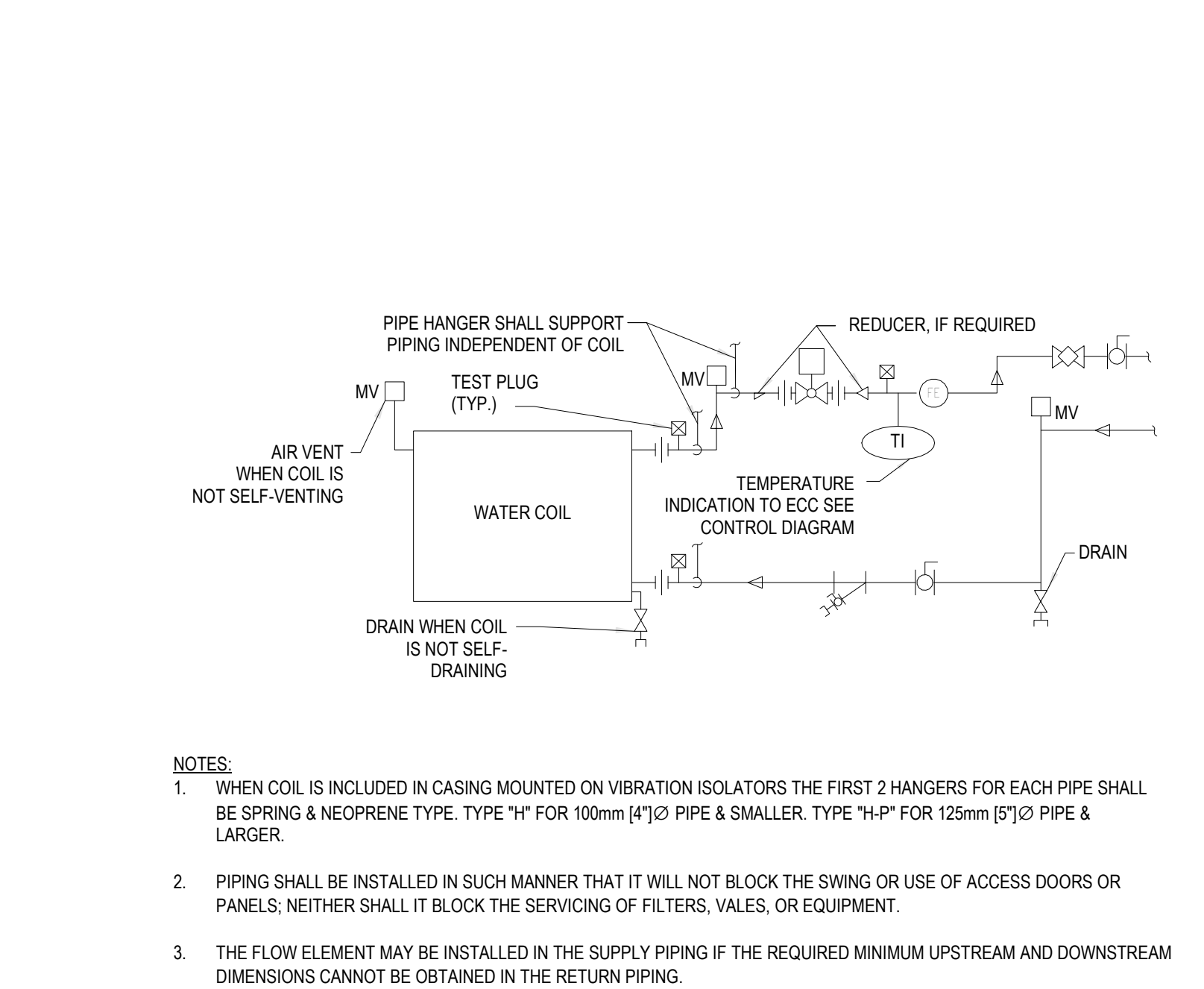
4 CHILLED WATER COIL - PIPING CONNECTIONS
