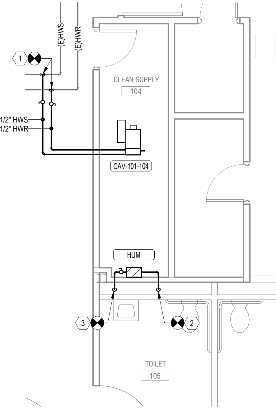
2 Bldg 101-01-FIRST FLOOR PIPING PLAN - ROOM 104 1/4" = 1'-0"
