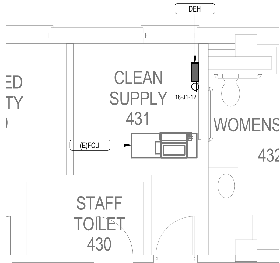
BLDG 18-04 FOURTH FLOOR ELECTRICAL PLAN - ROOM 431
