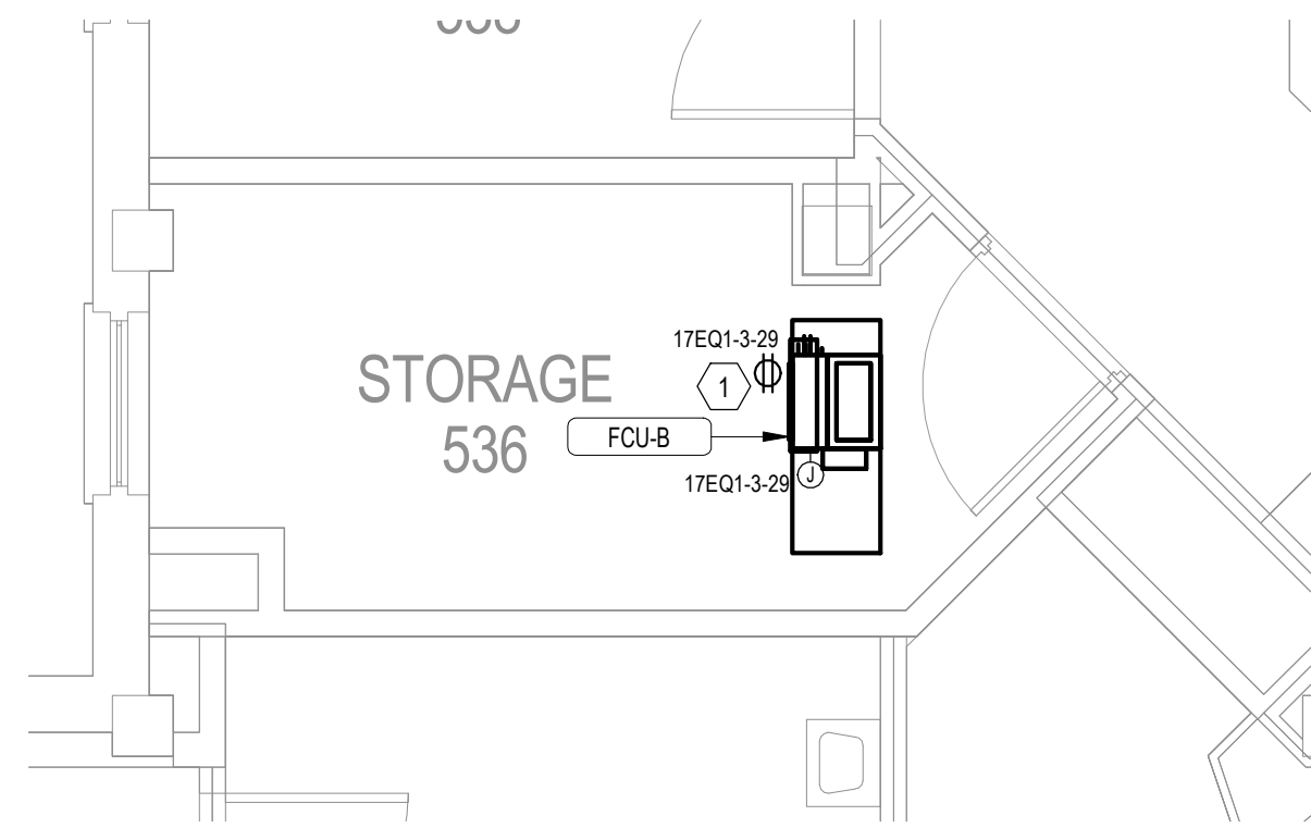
BID DEDUCT 1 - BLDG 17-05 FIFTH FLOOR ELECTRICAL PLAN - ROOM
