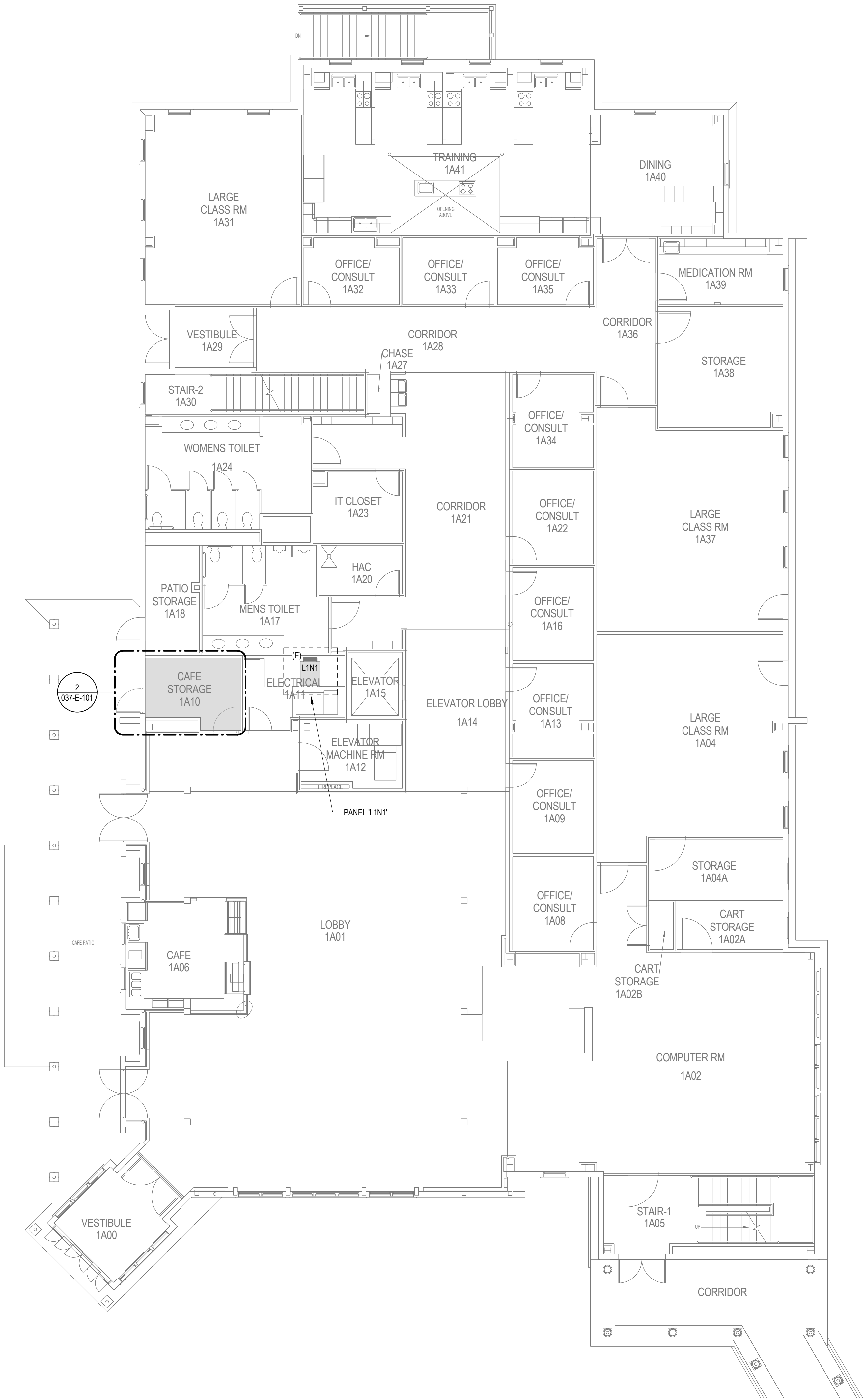
1 1/8" = 1'-0" BLDG 37-01 FIRST FLOOR ELECTRICAL PLAN
