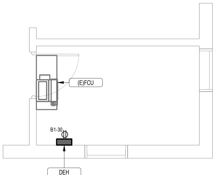
2 BID DEDUCT 1 - BLDG 17-02 SECOND FLOOR ELECTRICAL PLAN - ROOM 208 1/4" = 1'-0"
