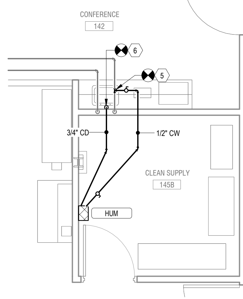
4 Bldg 101-01-FIRST FLOOR PIPING PLAN - ROOM 145B 1/4" = 1'-0"
