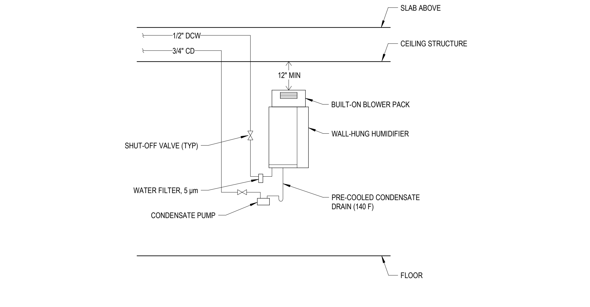
12 ELECTRODE STEAM HUMIDIFIER DETAIL
