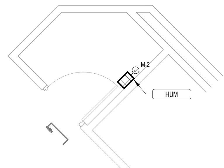
3 BID DEDUCT 1 - BLDG 17-02 SECOND FLOOR ELECTRICAL PLAN - ROOM 264 1/4" = 1'-0"
