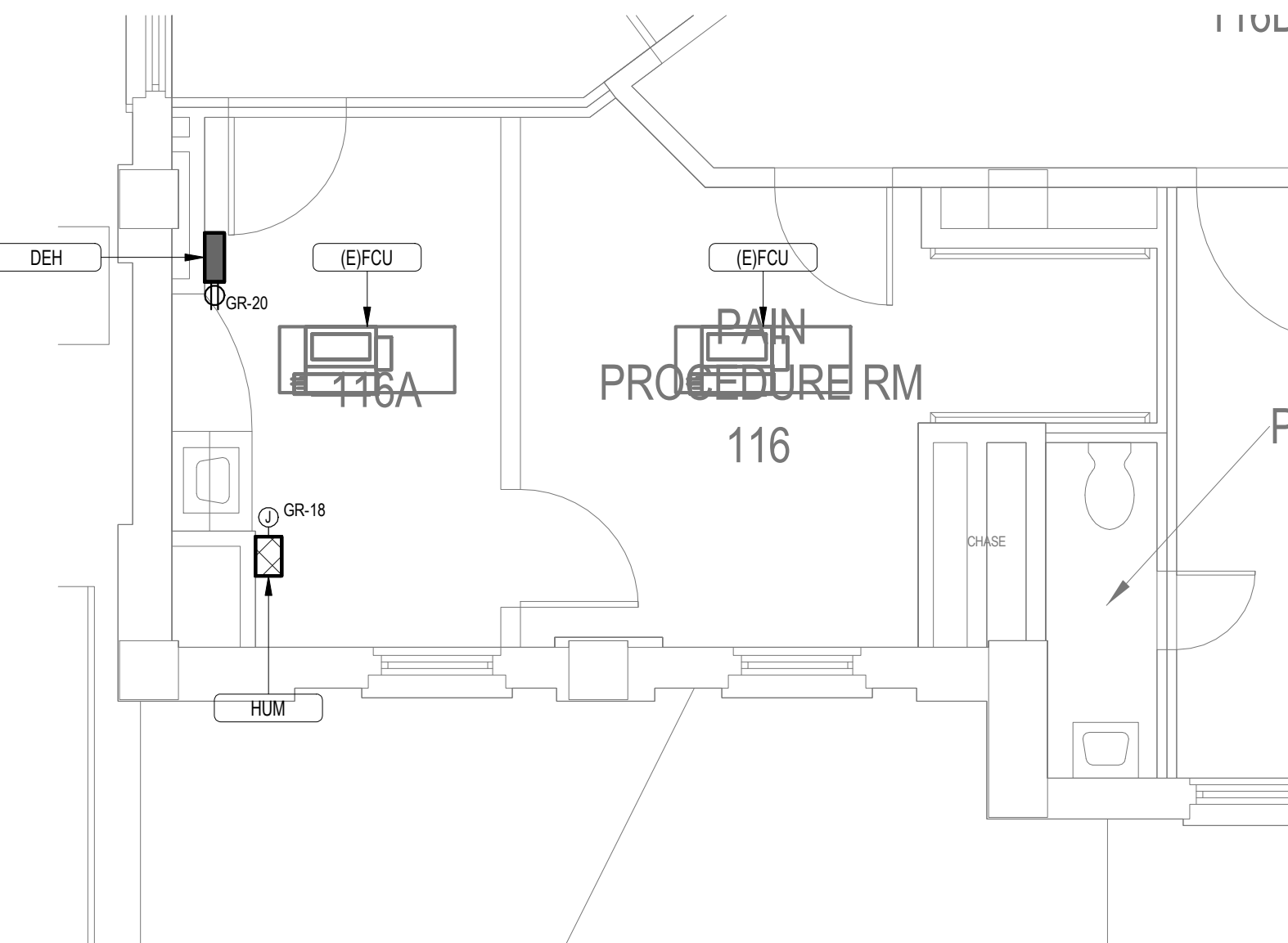
3 BLDG 01-01 FIRST FLOOR ELECTRICAL PLAN - ROOM 116A 1/4" = 1'-0"
