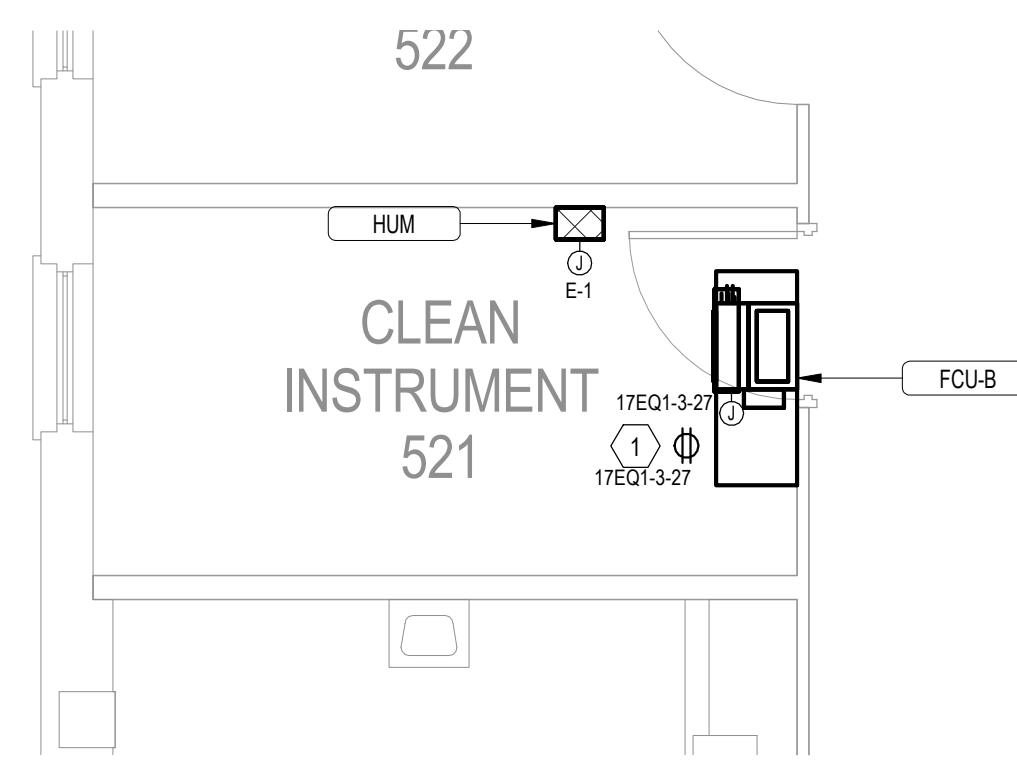
BID DEDUCT 1 - BLDG 17-05 FIFTH FLOOR ELECTRICAL PLAN - ROOM
