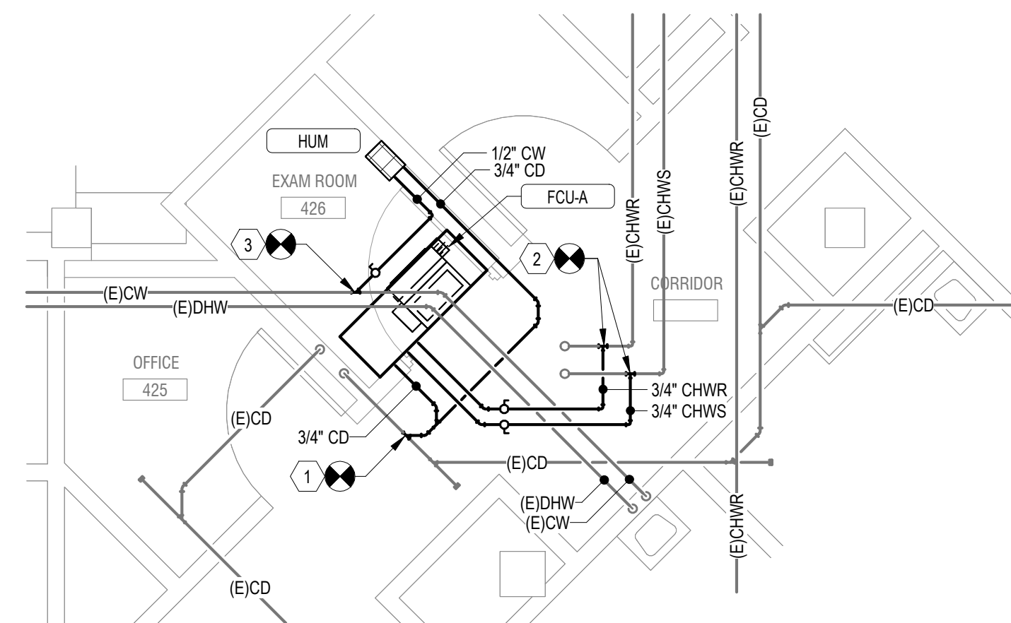
BID DEDUCT 1 - Bldg 17-04 FOURTH FLOOR PIPING PLAN - ROOM 426
