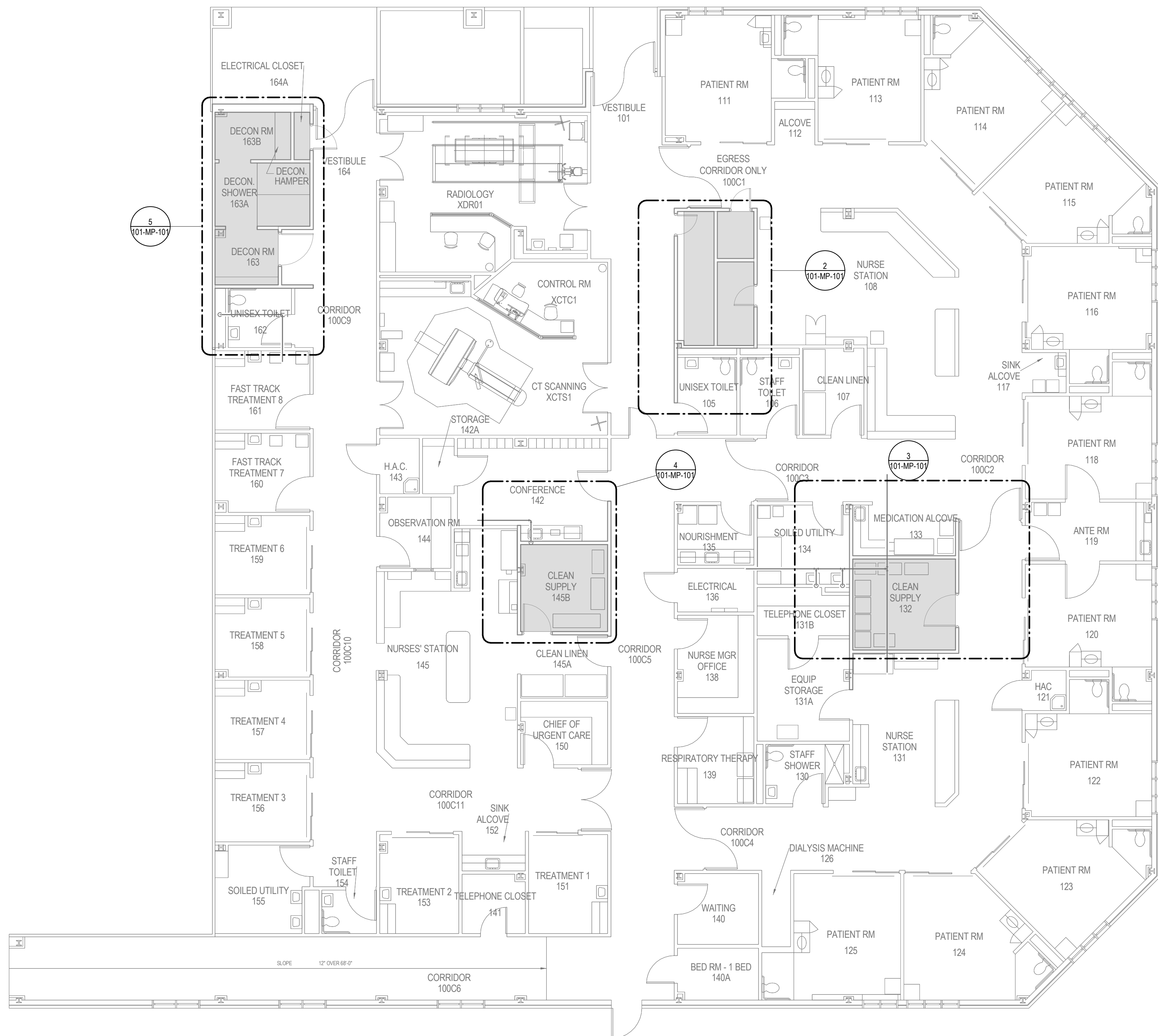
1 Bldg 101-01-FIRST FLOOR PIPING PLAN 1/8" = 1'-0"
