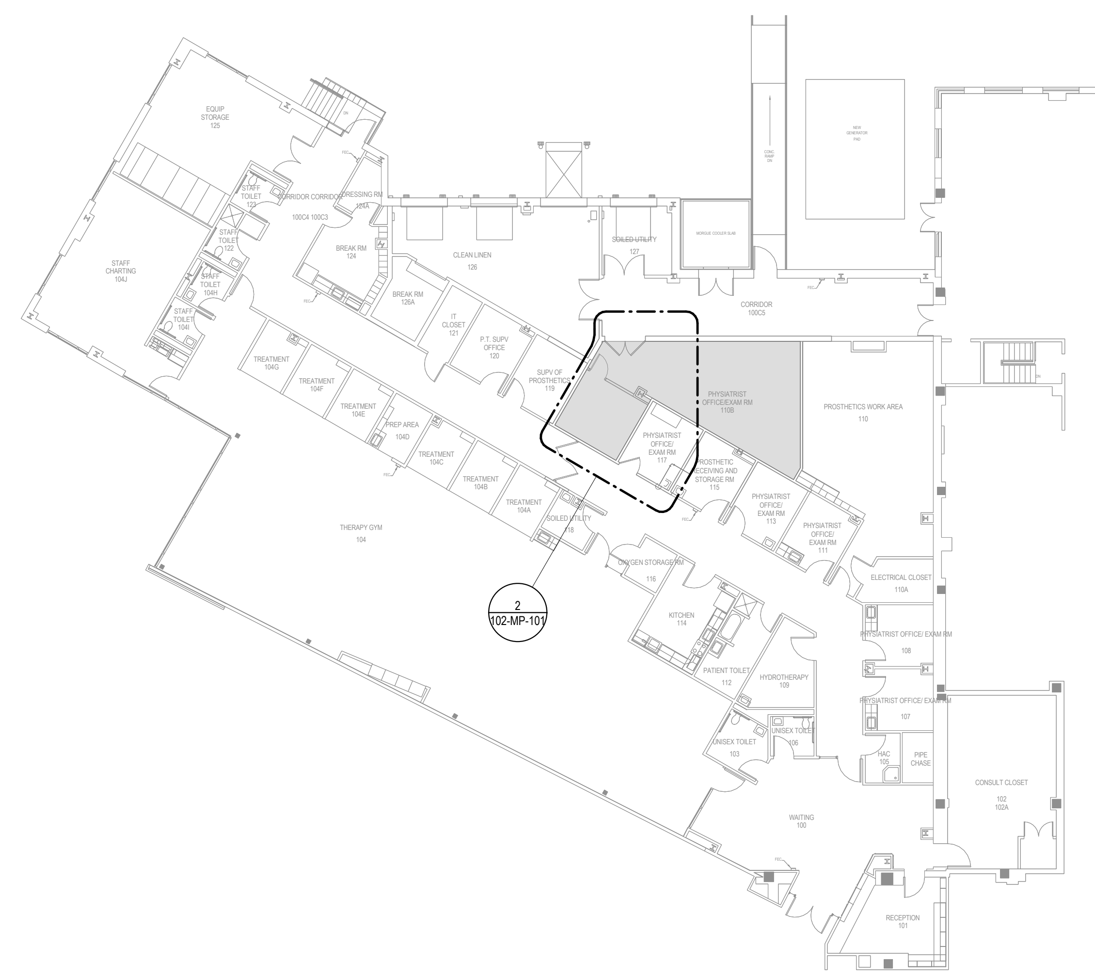
1 Bldg 102-01-FIRST FLOOR PIPING PLAN 1/16" = 1'-0"
