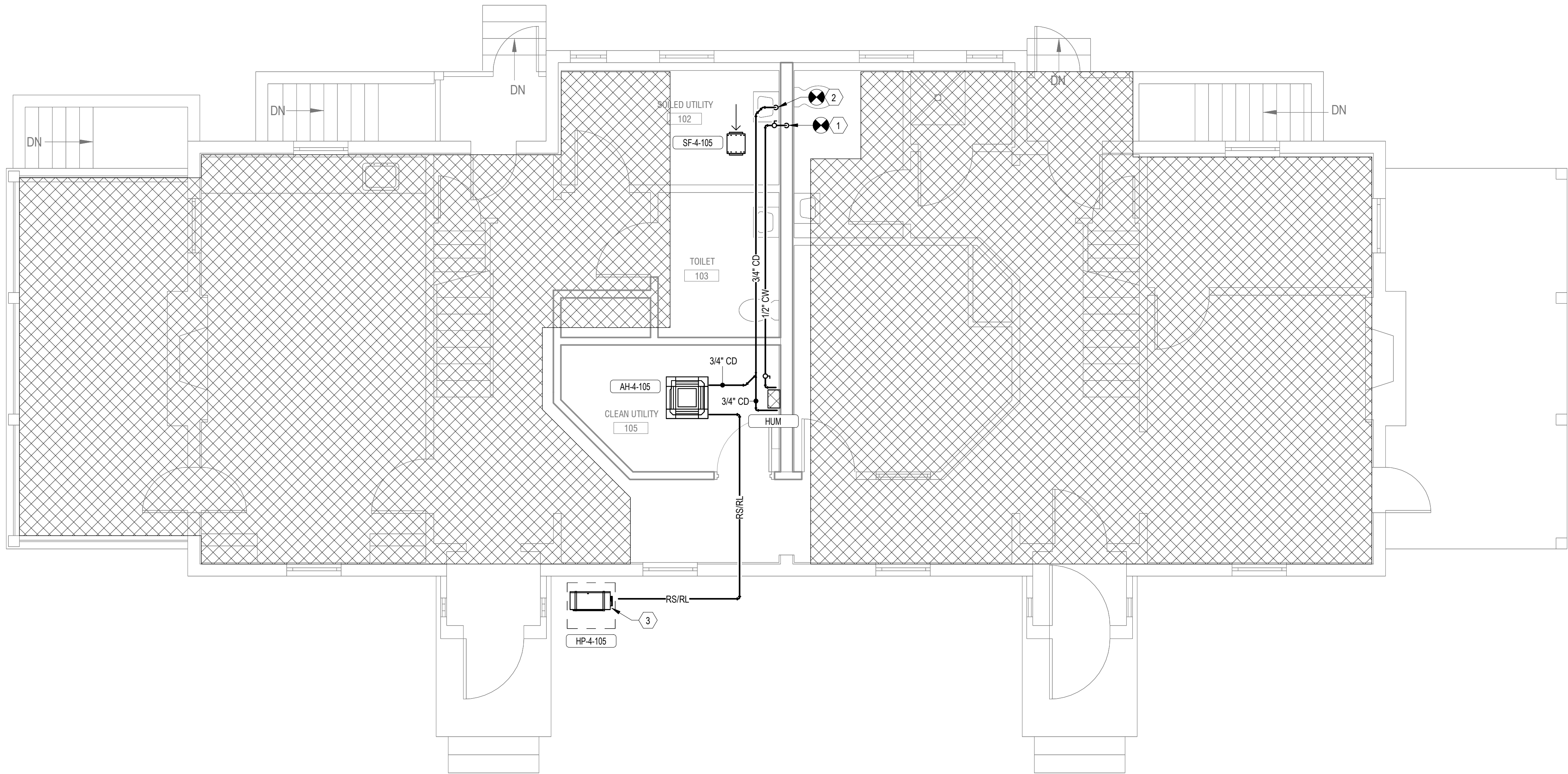
1 Bldg 04-01 FIRST FLOOR PIPING PLAN - ROOM 105 1/4" = 1'-0"
