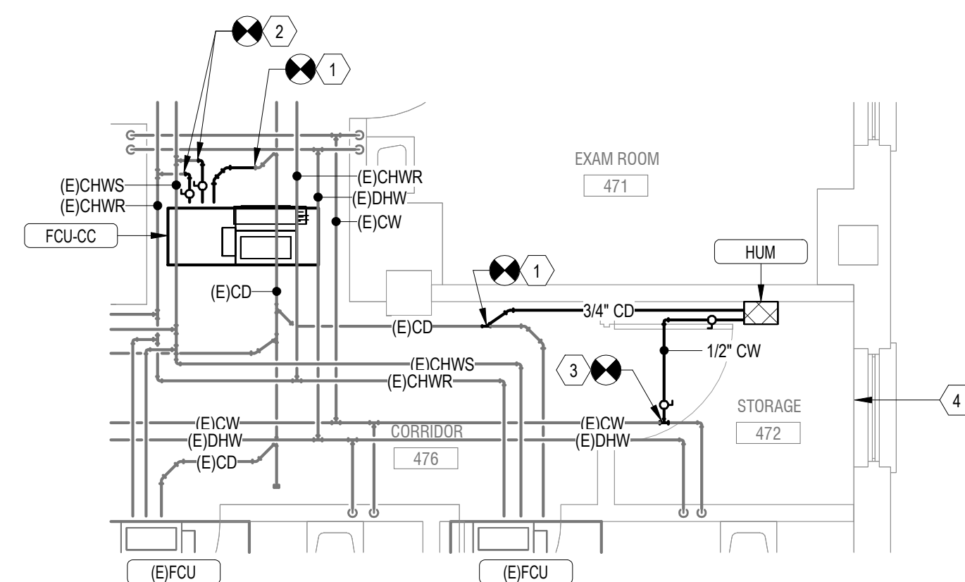
BID DEDUCT 1 - Bldg 17-04 FOURTH FLOOR PIPING PLAN - ROOM 472
