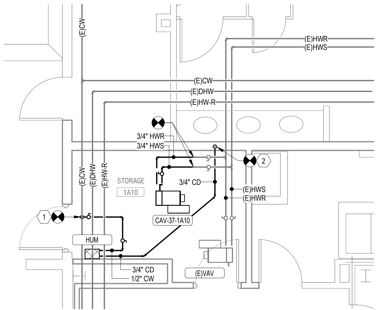
Bldg 37-01-FIRST FLOOR PIPING PLAN - ROOM 1A10
