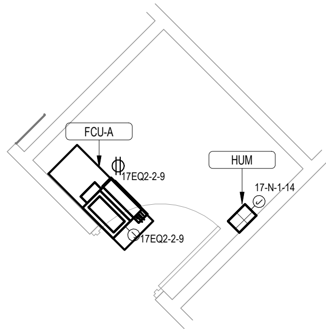
3 BID DEDUCT 1 - BLDG 17-03 THIRD FLOOR ELECTRICAL PLAN - ROOM 369 1/4" = 1'-0"
