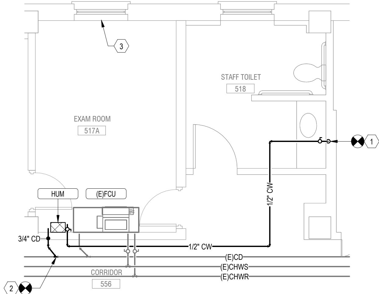
Bldg 18-05 FIFTH FLOOR PIPING PLAN - ROOM 517A
