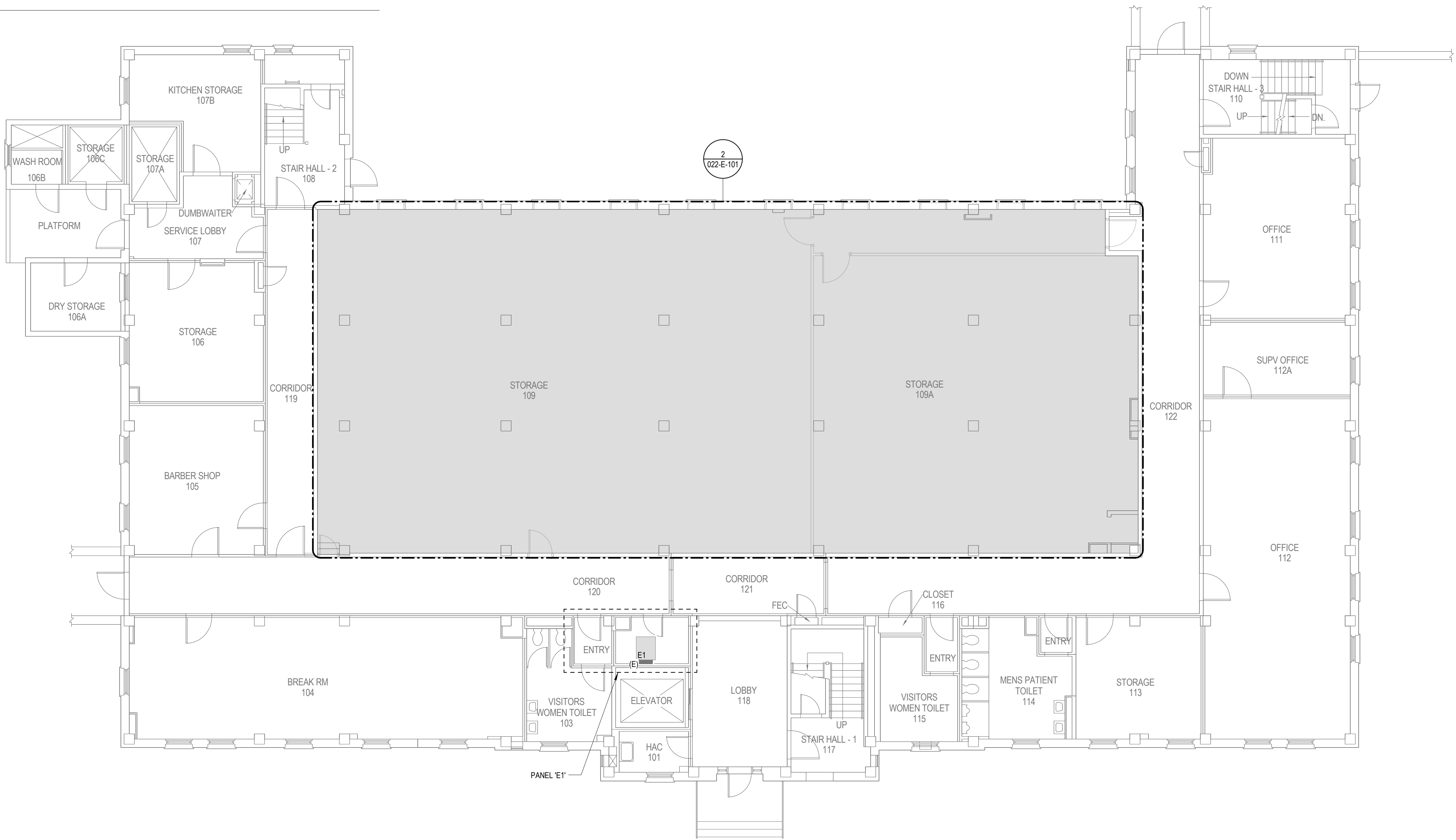
1 BLDG 22-01 FIRST FLOOR ELECTRICAL PLAN 1/8" = 1'-0"
