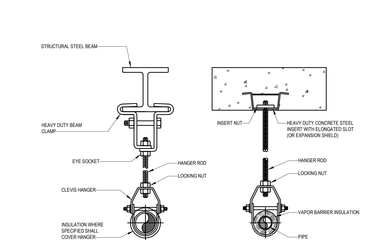
10 PIPE HANGER SUPPORTS
