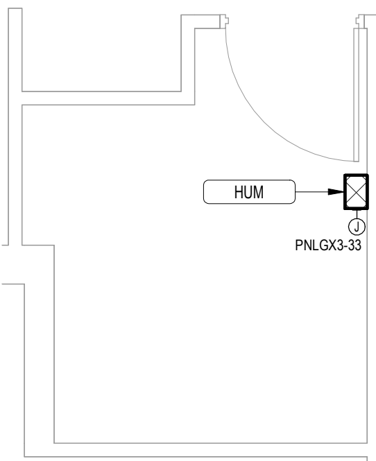
BLDG 104-01 FIRST FLOOR ELECTRICAL PLAN - ROOM 1121
