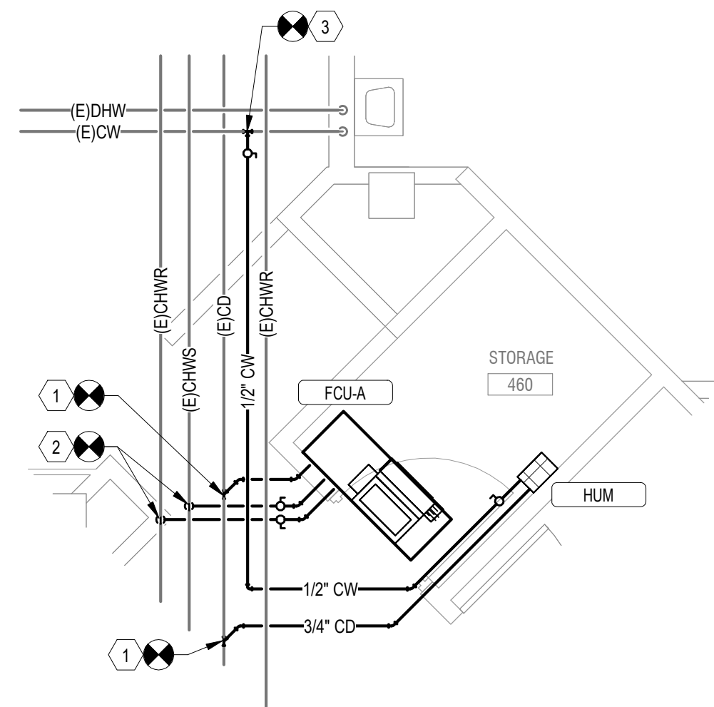
BID DEDUCT 1 - Bldg 17-04 FOURTH FLOOR PIPING PLAN - ROOM 460
