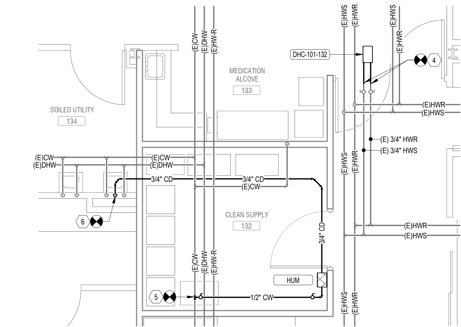
3 Bldg 101-01-FIRST FLOOR PIPING PLAN - ROOM 132 1/4" = 1'-0"
