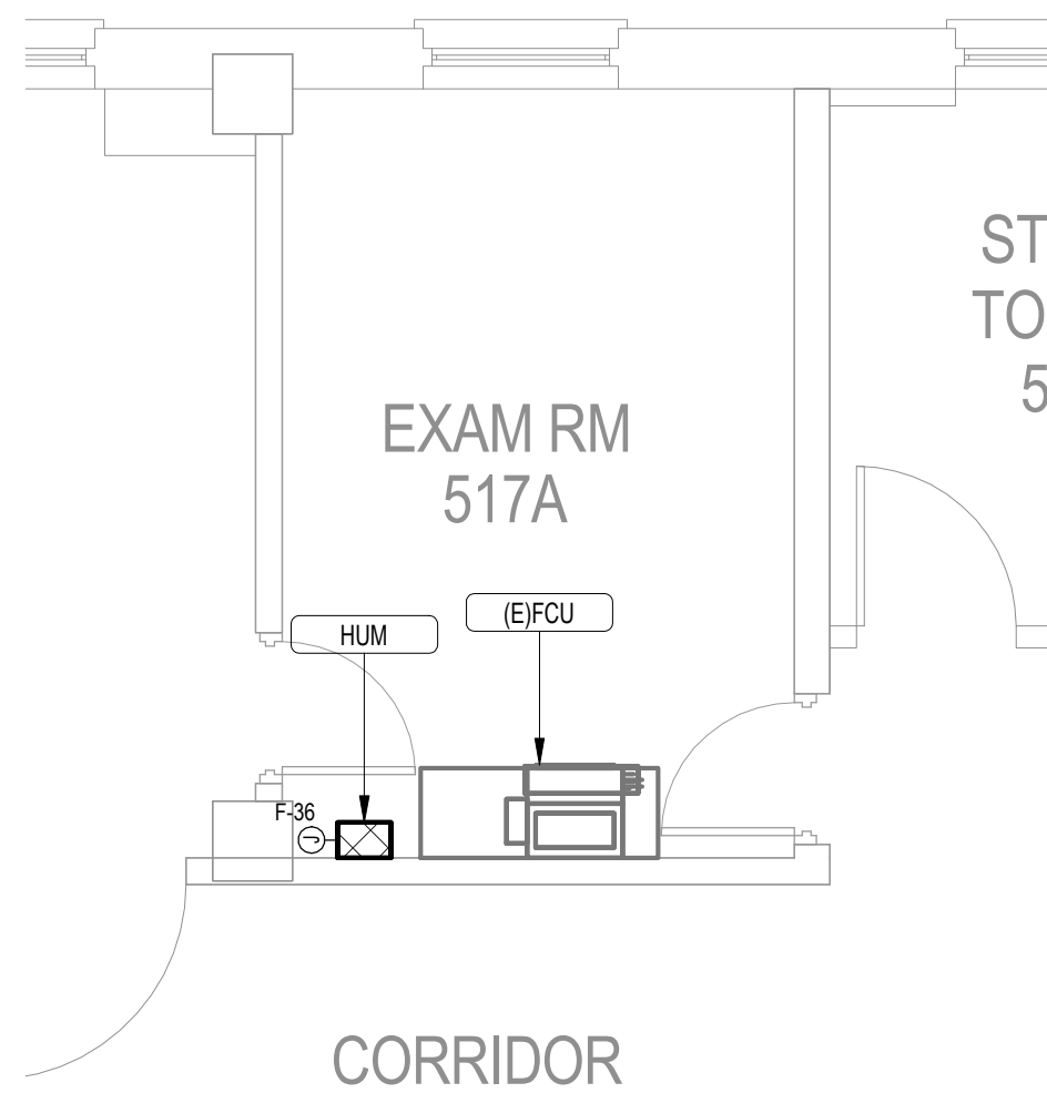
BLDG 18-05 FIFTH FLOOR ELECTRICAL PLAN - ROOM 517A
