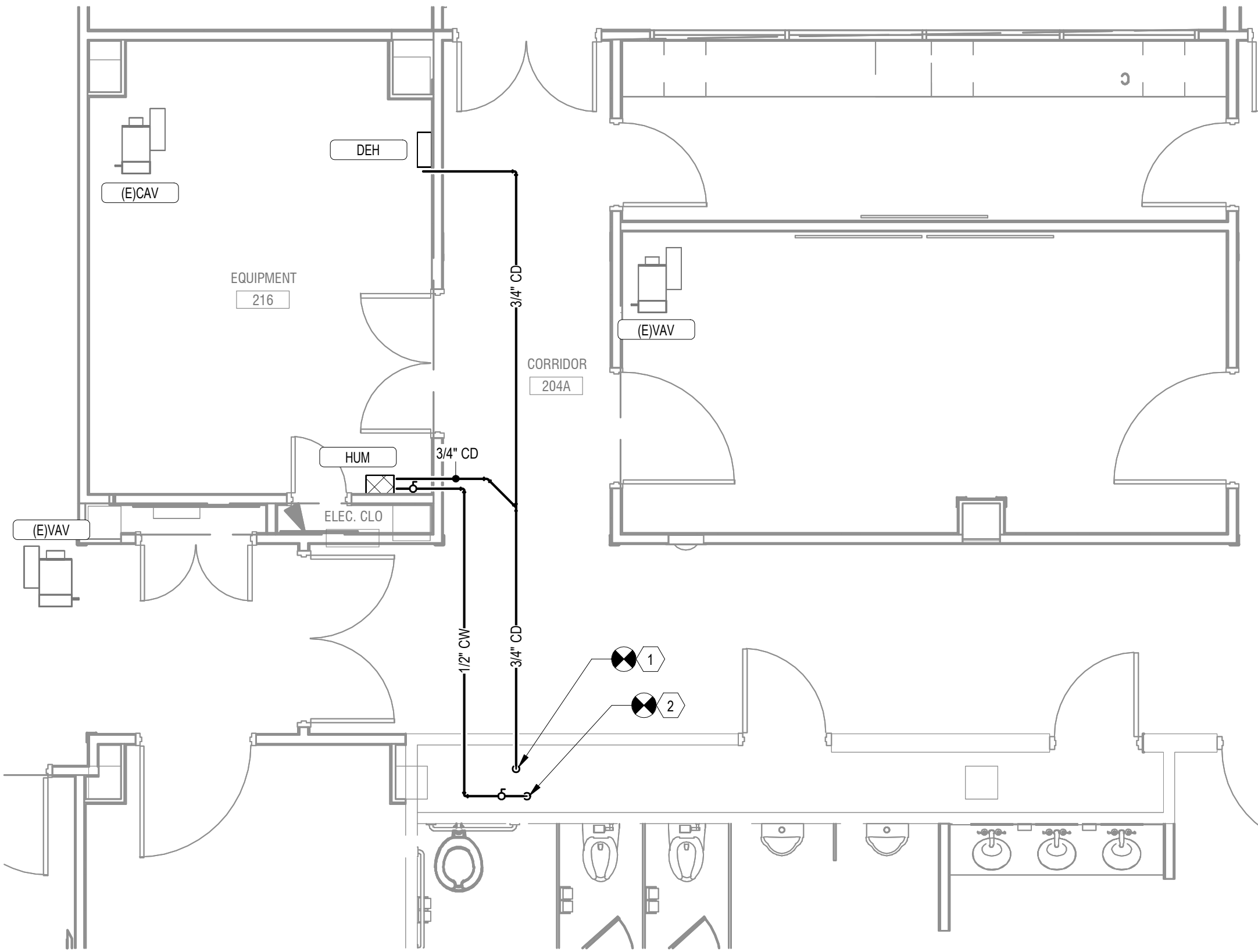
2 Bldg 22-02-SECOND FLOOR PIPING PLAN - ROOM 216 1/4\"/>
