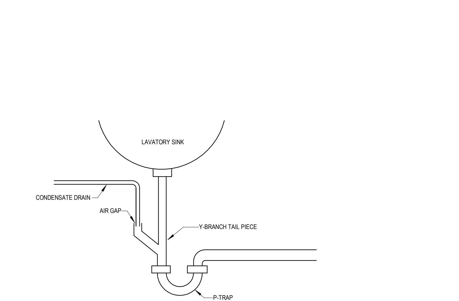
9 CONDENSATE DRAIN TO LAVATORY SINK
