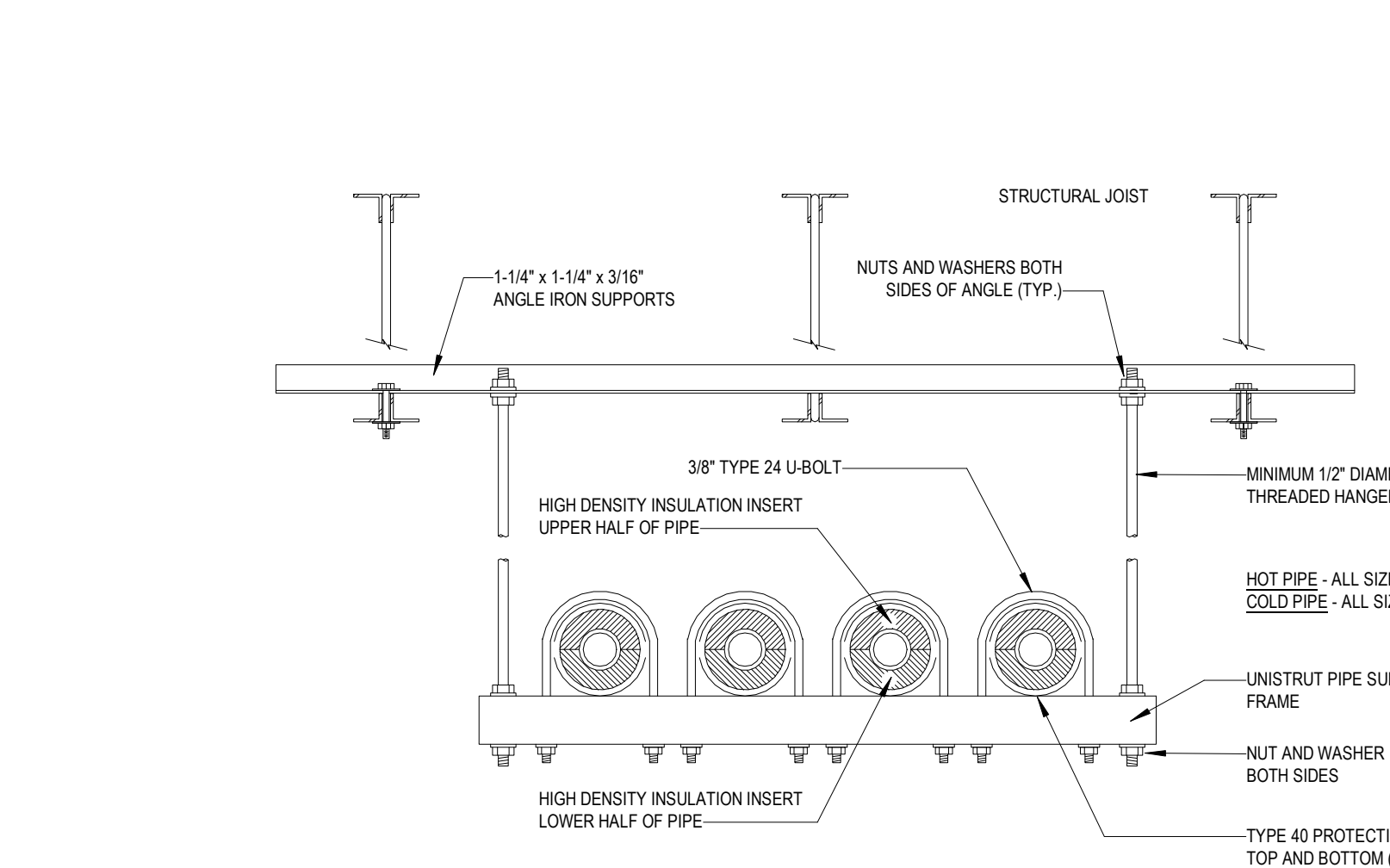
11 HORIZONTAL PIPE SUPPORT
