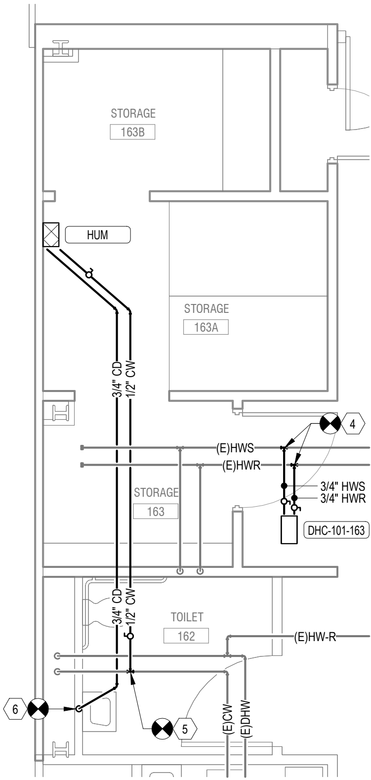
5 Bldg 101-01-FIRST FLOOR PIPING PLAN - ROOM 163, 163A, 163B 1/4" = 1'-0"
