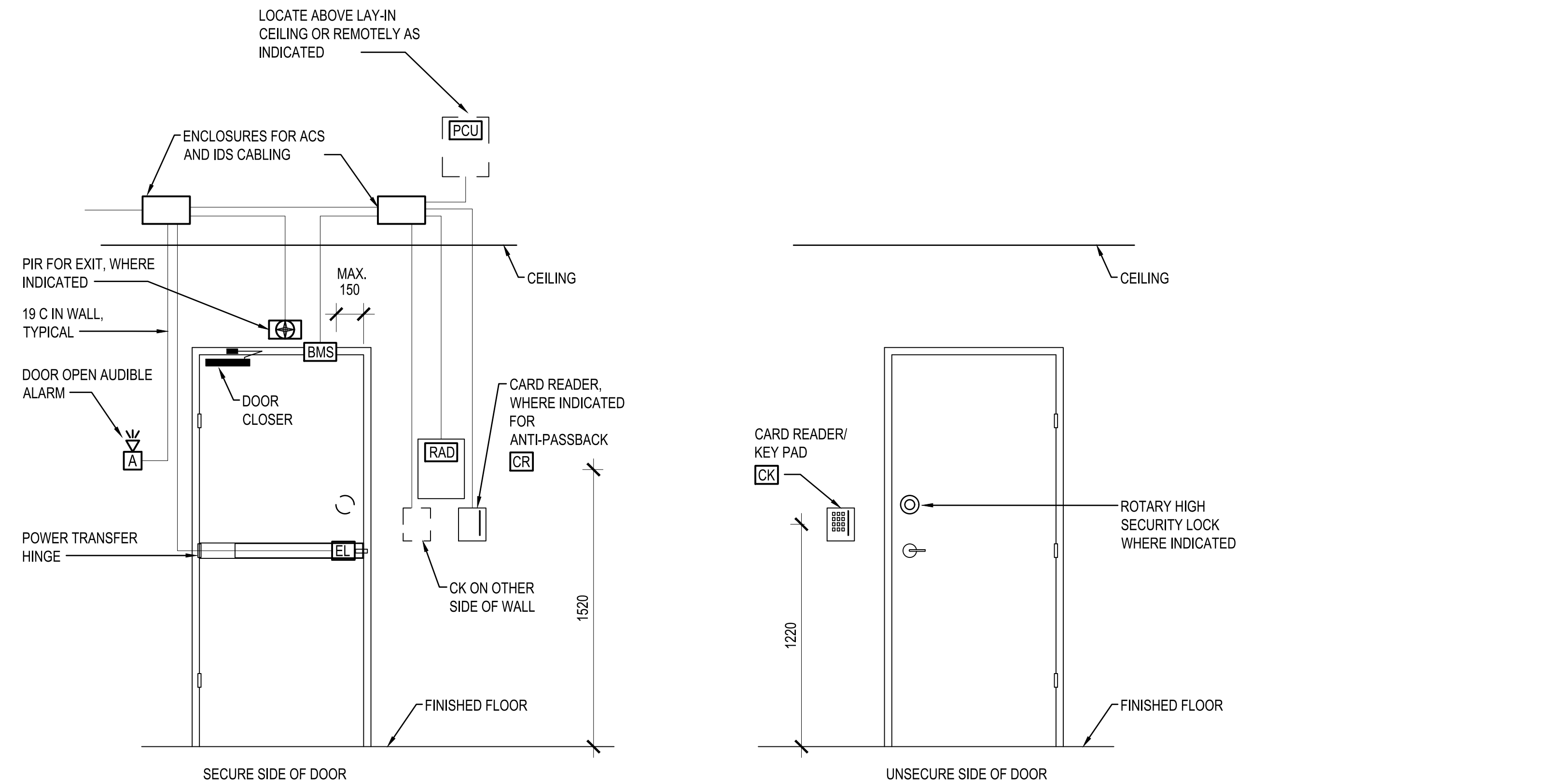
A1 SINGLE DOOR ELEVATION FOR ESS ROUGH-IN SCALE: NOT TO SCALE
