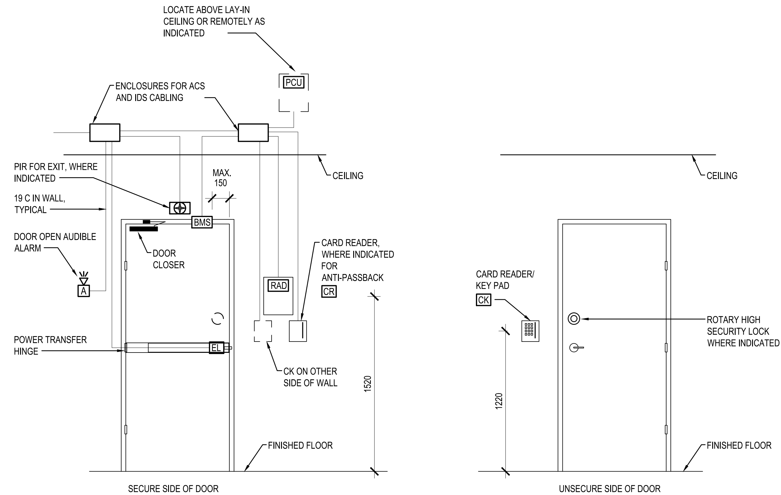
A1 SINGLE DOOR ELEVATION FOR ESS ROUGH-IN SCALE: NOT TO SCALE
