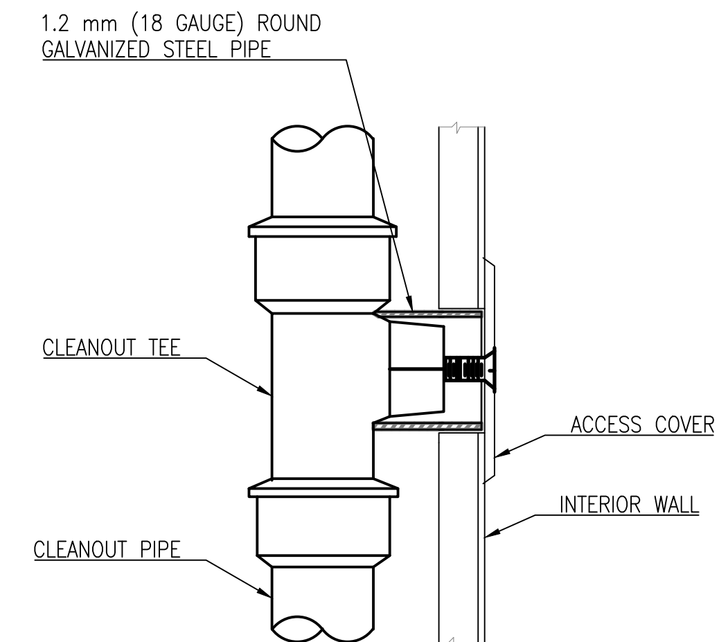
B4 WALL CLEANOUT DETAIL SCALE: NOT TO SCALE
