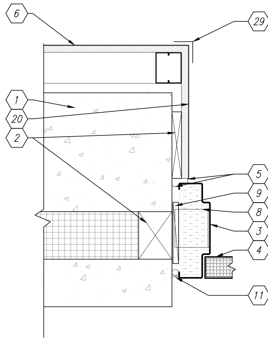
A1 EXTERIOR DOOR DETAIL - JAMB SCALE: 1:5
