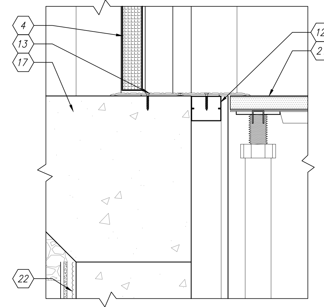
B4 INTERIOR DOOR DETAIL - SILL SCALE: 1:5
