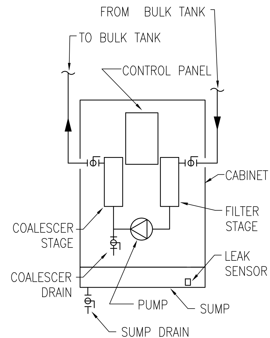
C3 AUTOMATIC FUEL POLISHING UNIT DETAIL N.T.S.
