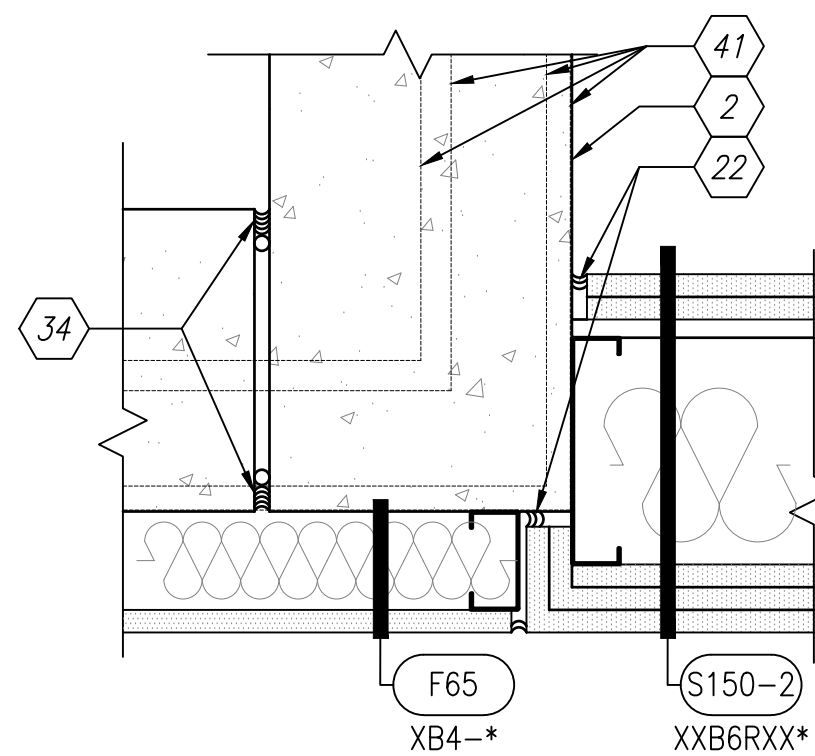
A2 3-HOUR WALL TO 1-HR WALL INTERSECTION SCALE: 1:5 A-105
