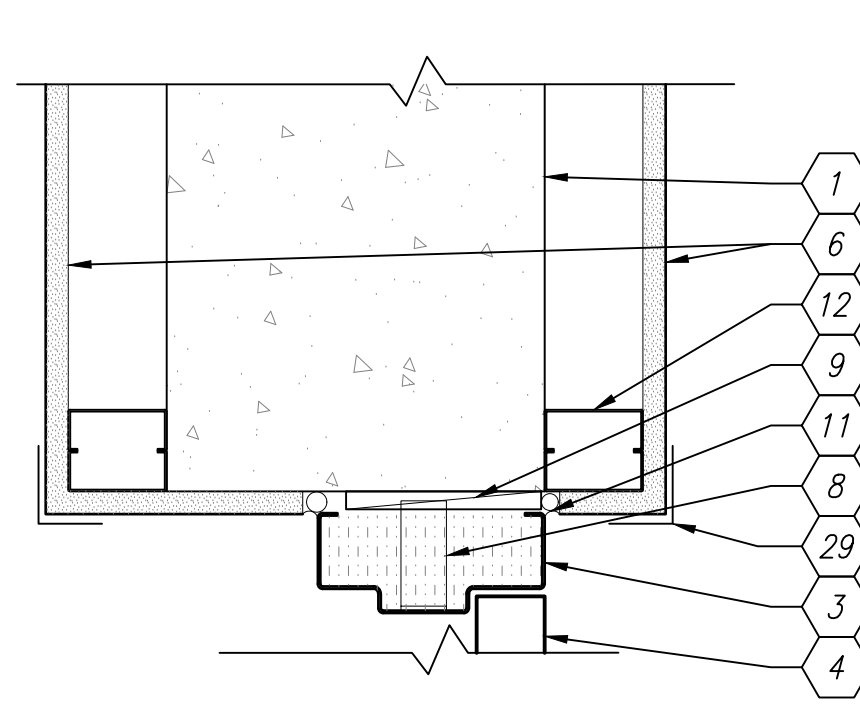
D3 INTERIOR DOOR DETAIL - HEAD/JAMB SCALE: 1:5
