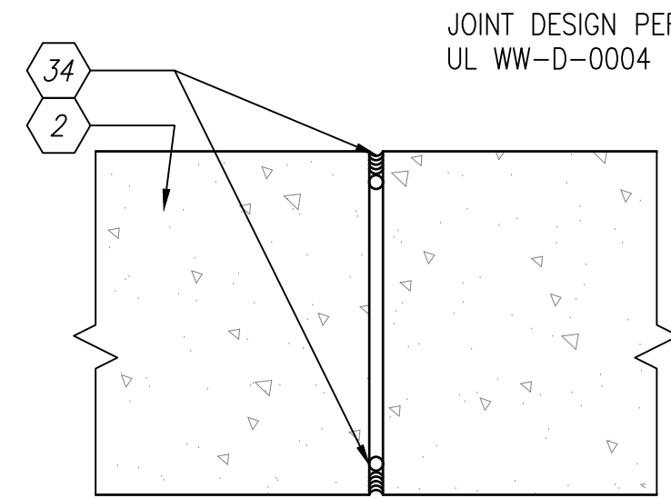
C4 FIRE RATED WALL INTERSECTION JOINT SCALE: 1:5
