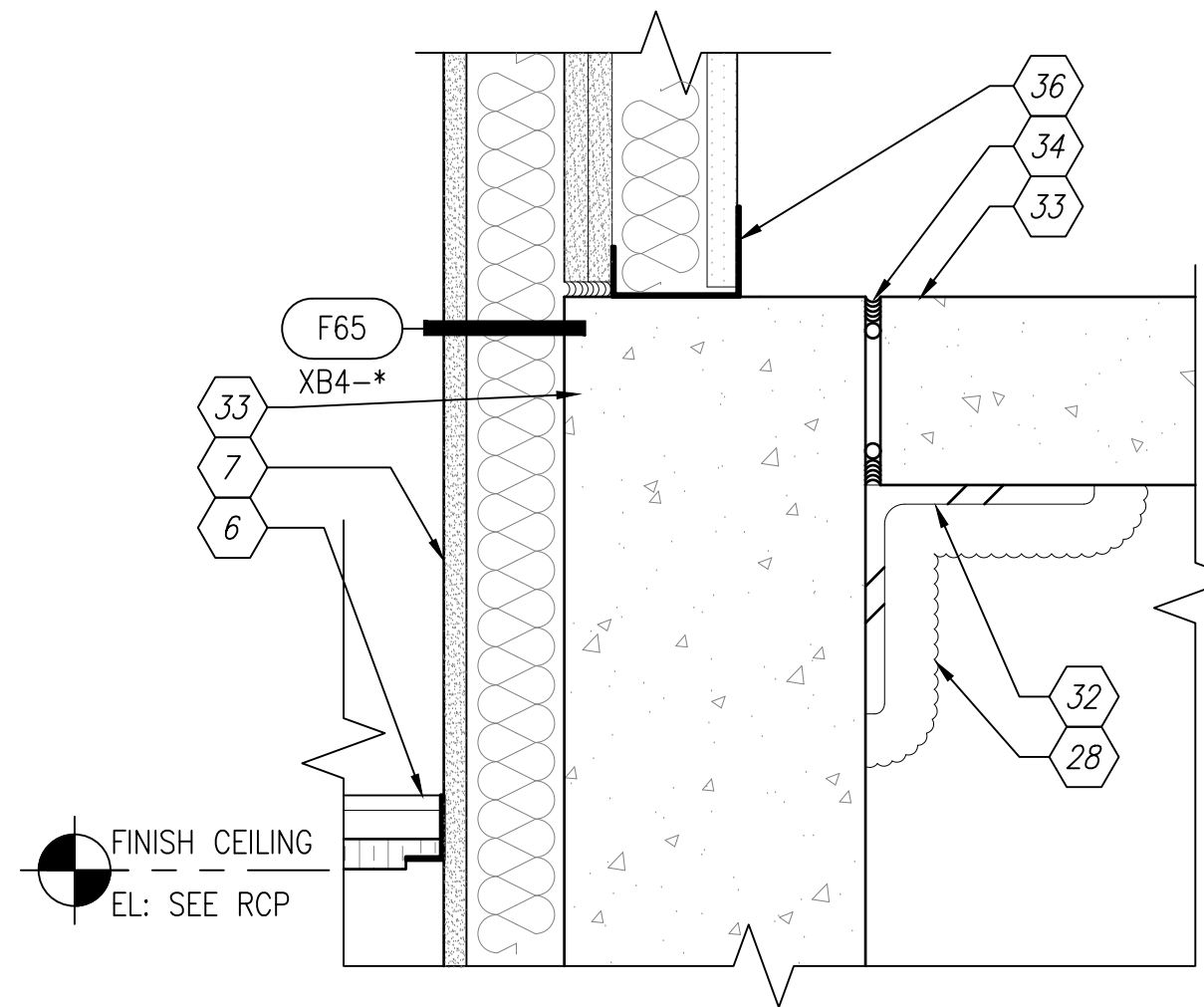
B2 3-HR CONCRETE CAP TO TO 1-HR SHAFTWALL SCALE: 1:5 A-506
