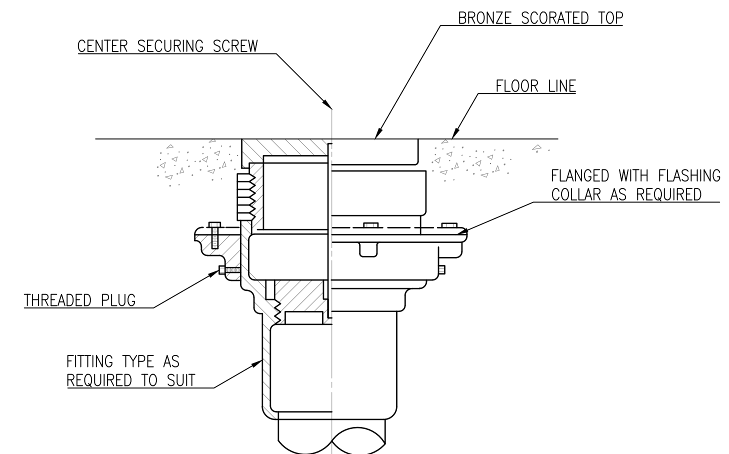
A4 FLOOR CLEANOUT DETAIL SCALE: NOT TO SCALE
