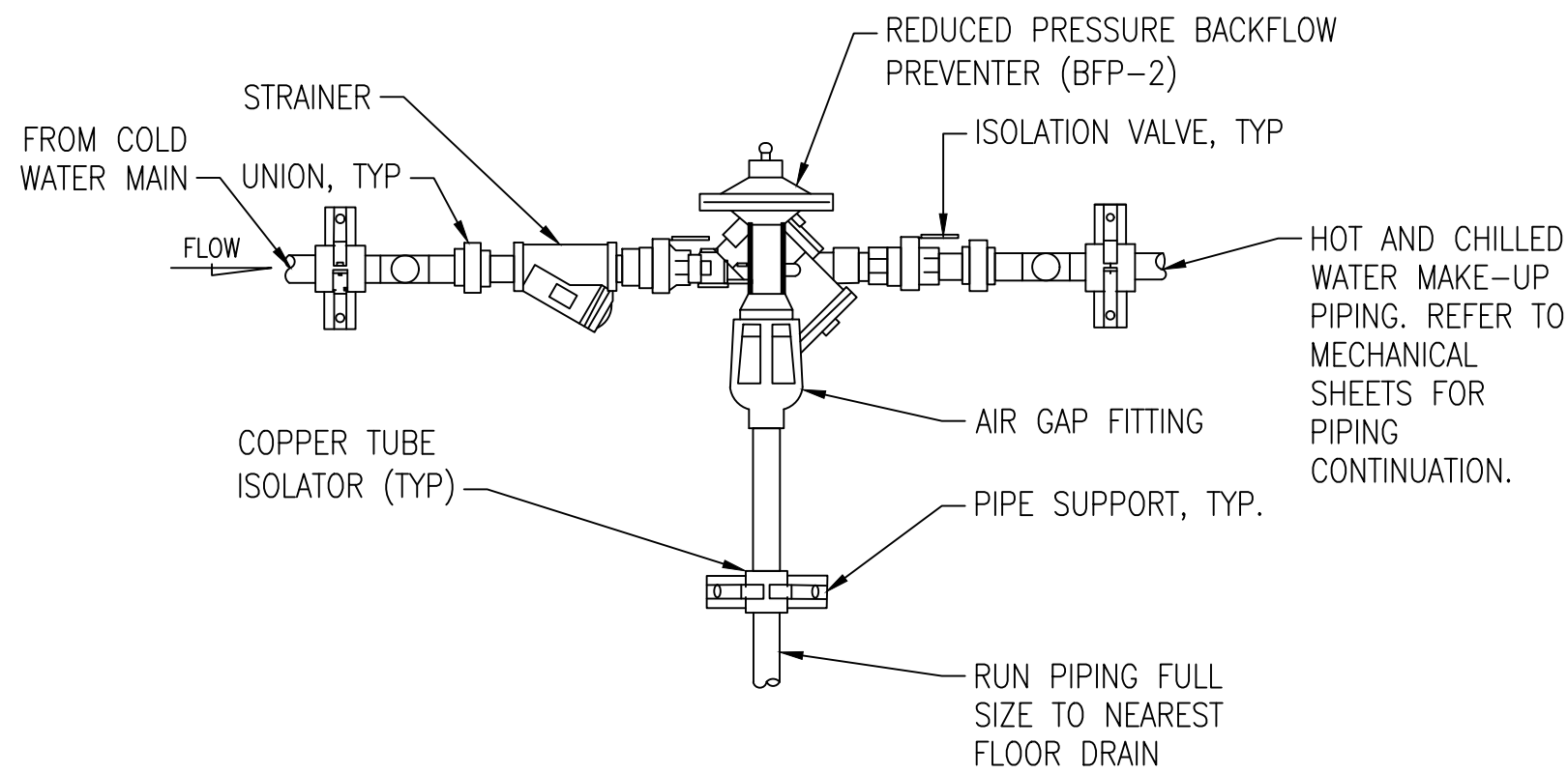
C1 REDUCED PRESSURE BACKFLOW PREVENTER, WALL-MOUNT SCALE: NOT TO SCALE
