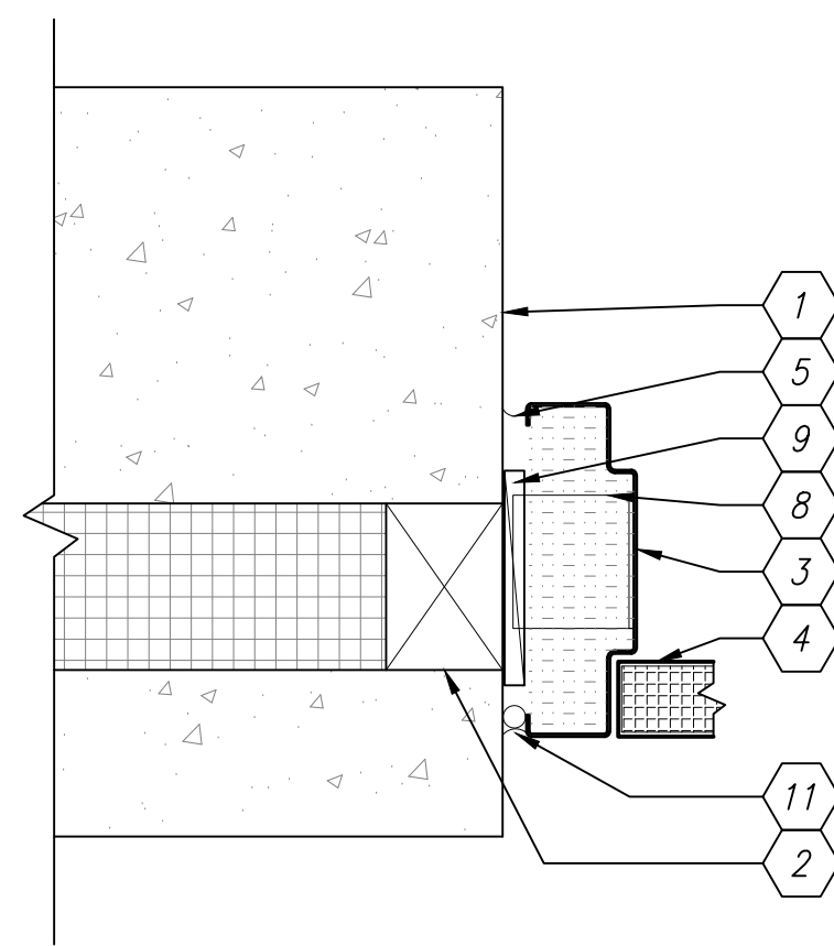
A2 EXTERIOR DOOR DETAIL - JAMB SCALE: 1:5
