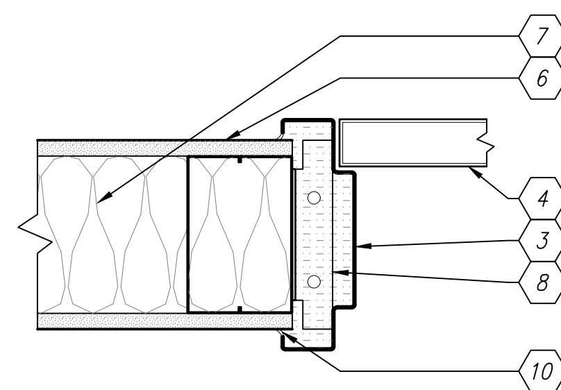
B3 INTERIOR DOOR DETAIL - SILL SCALE: 1:5
