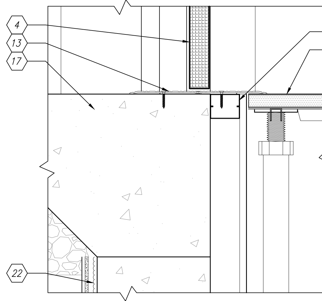
B3 INTERIOR DOOR DETAIL - SILL SCALE: 1:5
