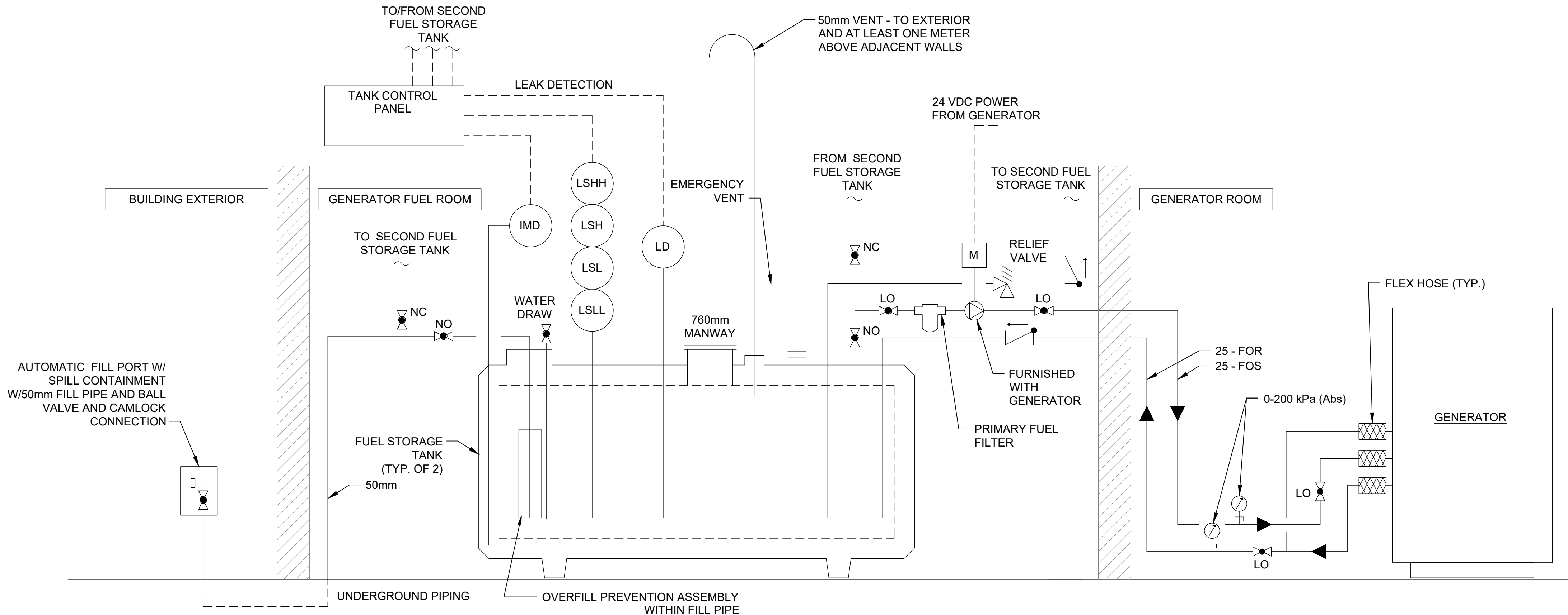
C1 FUEL PIPING SCHEMATIC FLOW DIAGRAM SCALE: NOT TO SCALE
