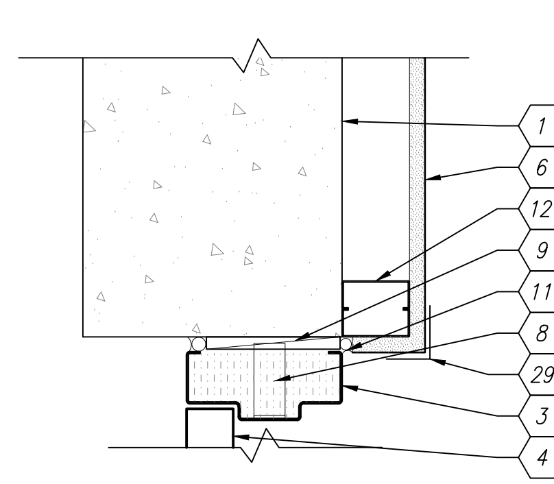
D4 INTERIOR DOOR DETAIL - HEAD/JAMB SCALE: 1:5
