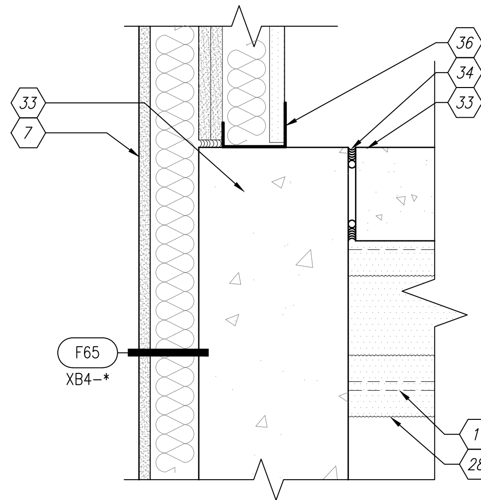
B1 3-HR CONCRETE CAP TO TO 1-HR SHAFTWALL SCALE: 1:5 A-307
