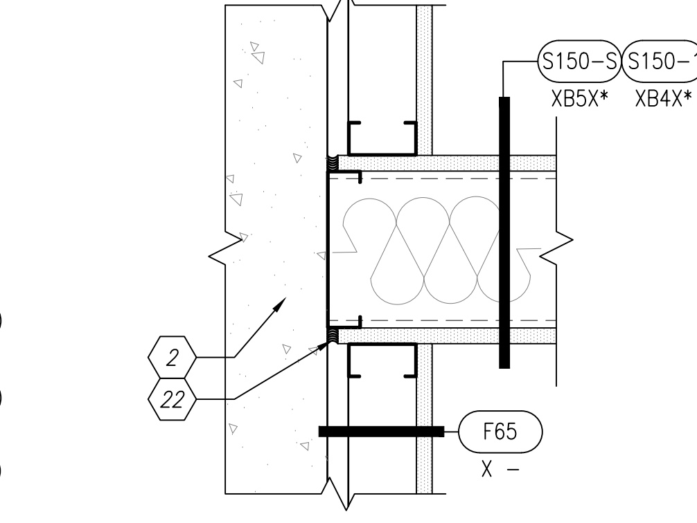
A4 1HR/SMOKE PARTITION TO EXTERIOR WALL INTERSECTION SCALE: 1:5 A-405
