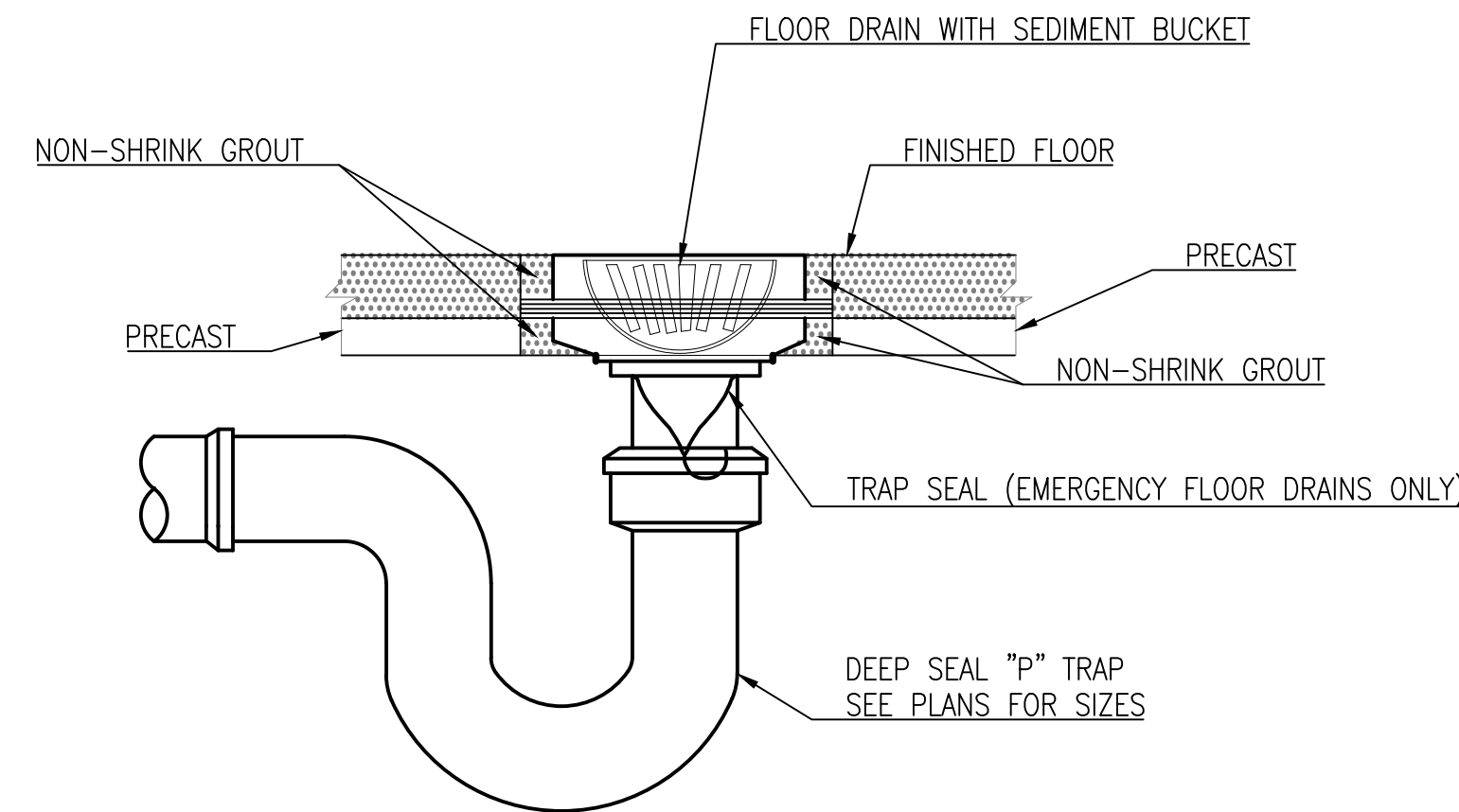
B3 FLOOR DRAIN DETAIL SCALE: NOT TO SCALE
