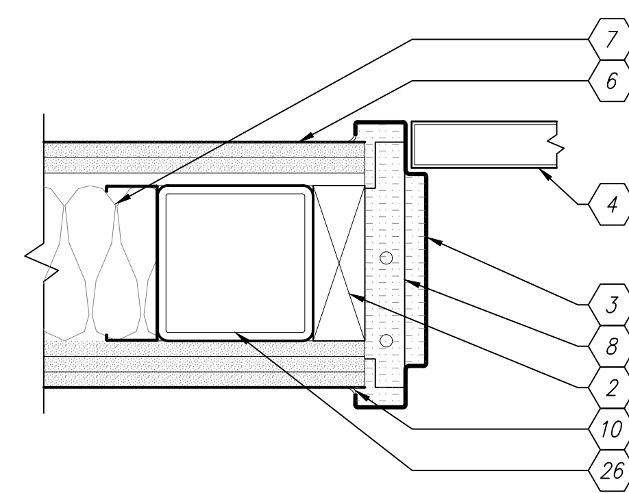
B5 180 MIN INTERIOR DOOR DETAIL - HEAD/JAMB SCALE: 1:5
