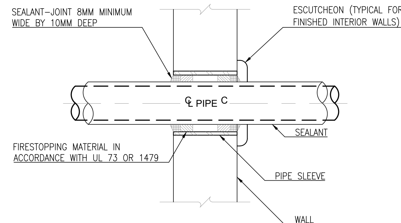
A3 PIPE INTERIOR WALL PENETRATION DETAIL SCALE: NOT TO SCALE
