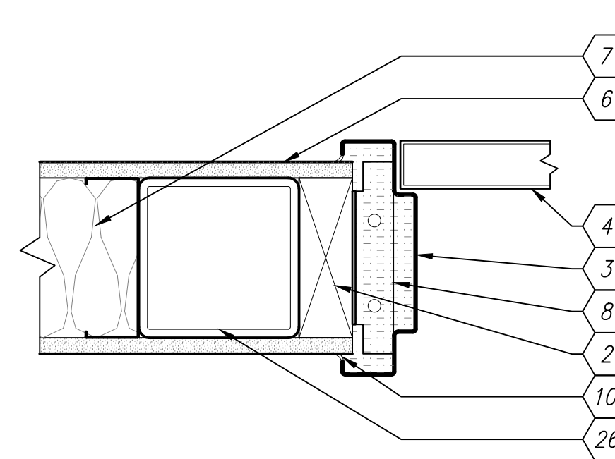
B4 INTERIOR DOOR DETAIL - SILL SCALE: 1:5
