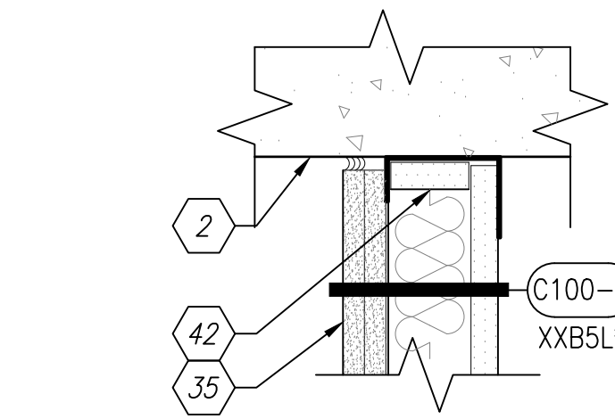
B5 1-HR SHAFTWALL TO EXTERIOR WALL SCALE: 1:5 A-405
