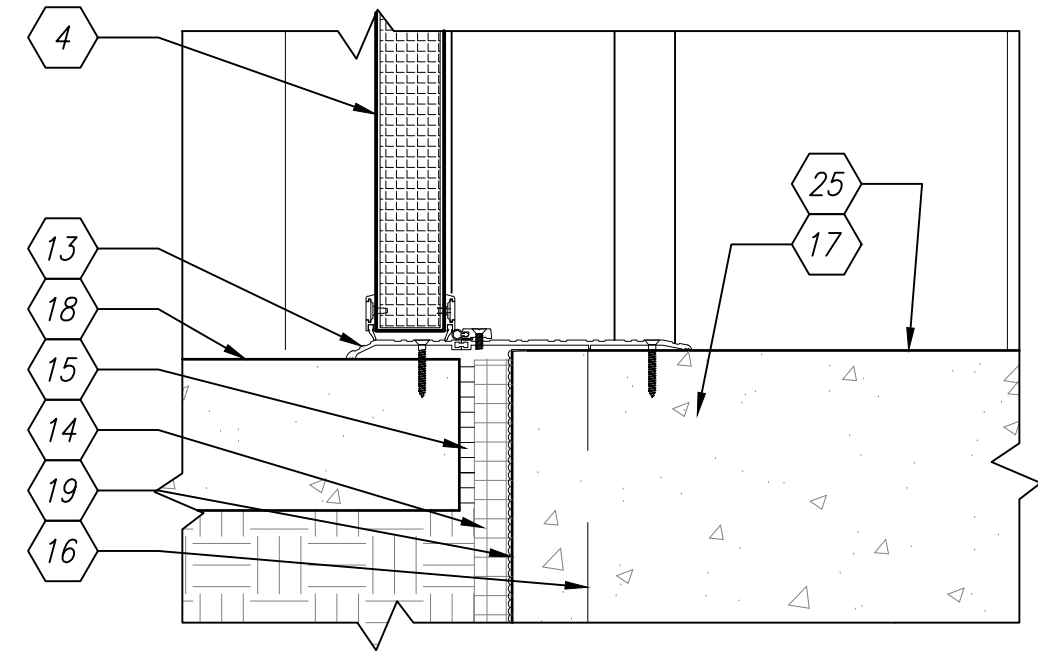
C1 EXTERIOR DOOR DETAIL - SILL SCALE: 1:5
