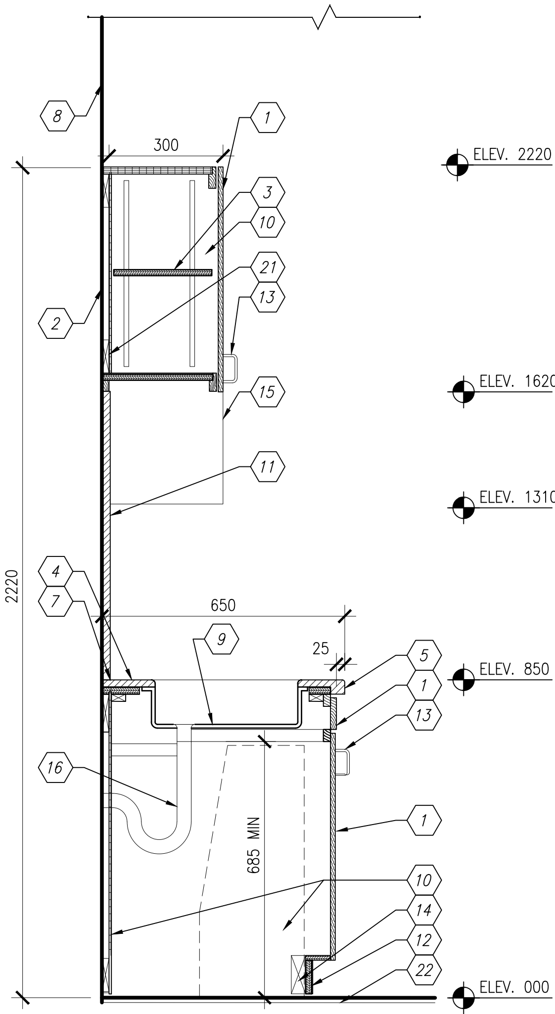
A1 SECTION AT CASEWORK - ROOM 105 SCALE: 1:10 A-406
