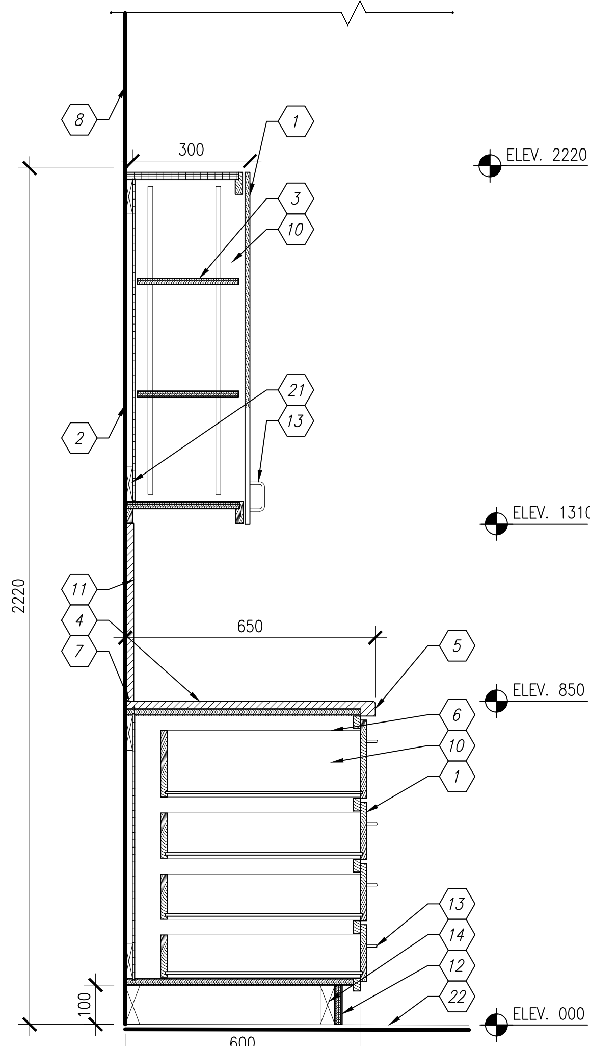
A2 SECTION AT CASEWORK - ROOM 105 SCALE: 1:10 A-406
