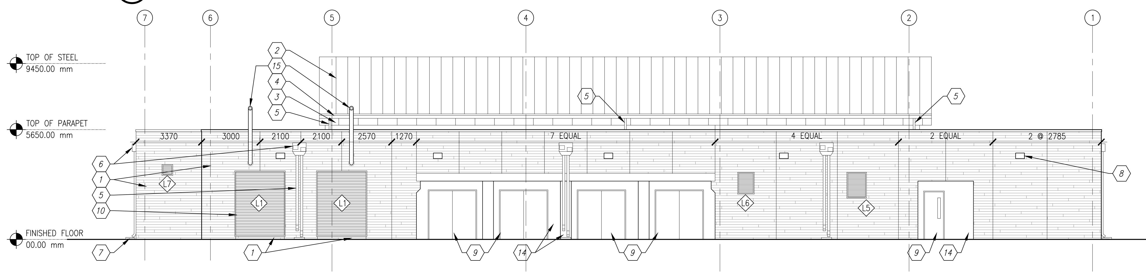
B1 SOUTH ELEVATION SCALE: 1:100
