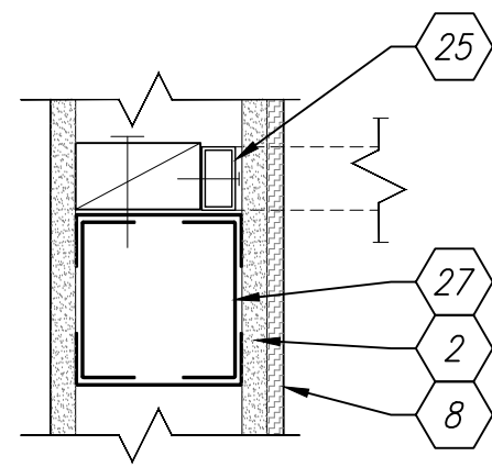
D1 PLANNED SECTION AT CONCEALED COUNTERTOP BRACKET SCALE: 1:5 A-407
