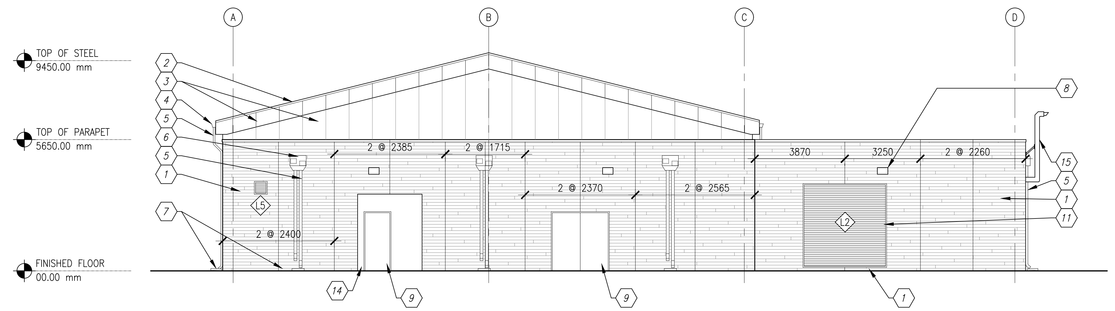
B1 SOUTH ELEVATION SCALE: 1:100
