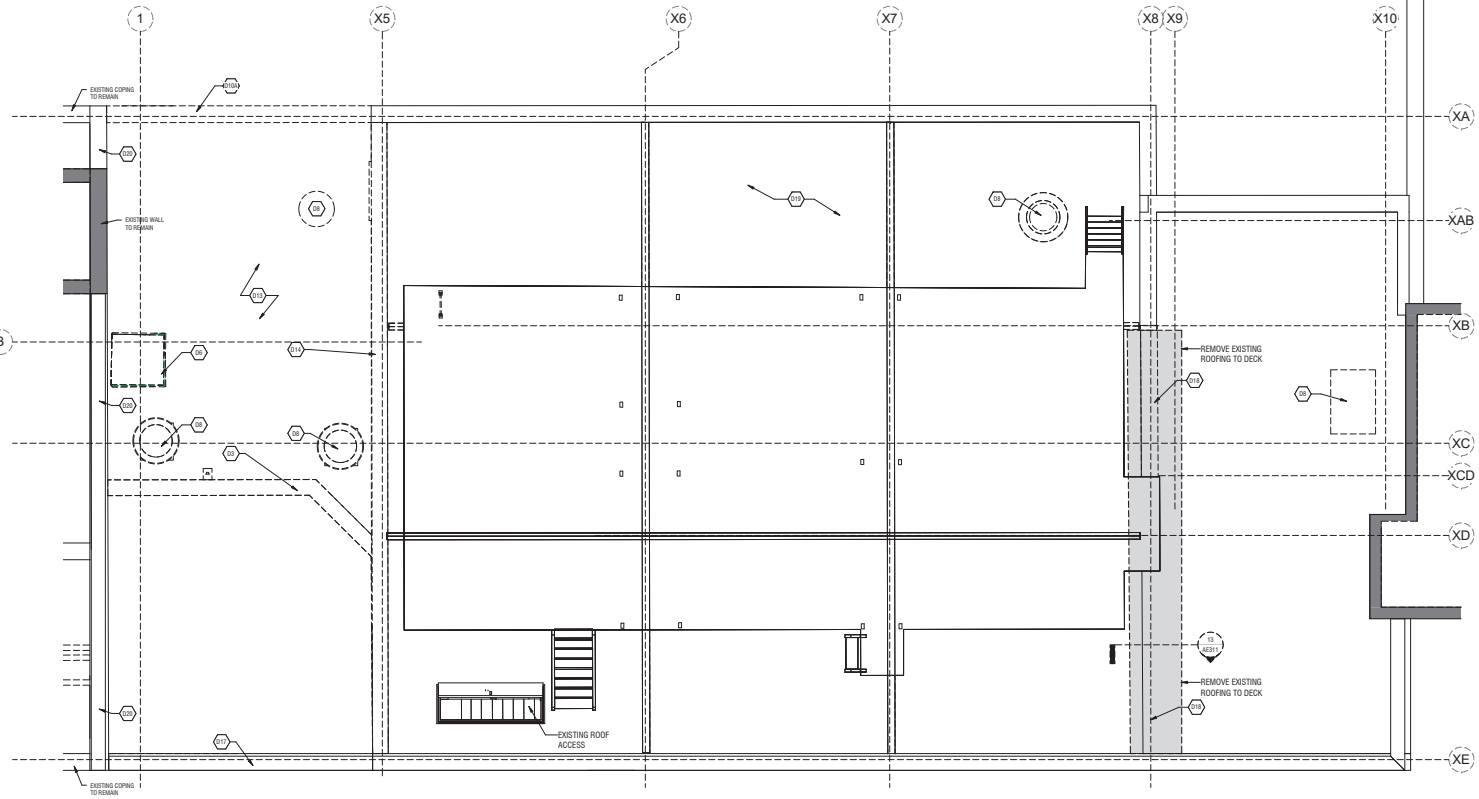
1 ROOF LEVEL DEMOLITION PLAN SCALE: 1/4" = 1'-0"
