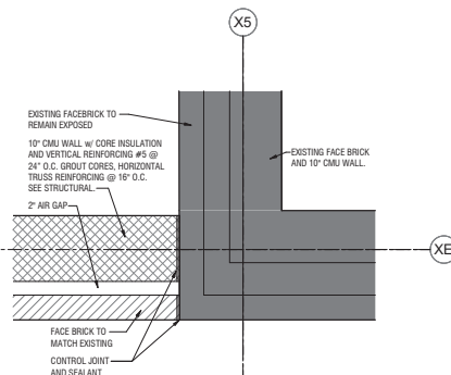
5 PLAN DETAIL AE310 SCALE: 1 1/2" = 1'-0"
