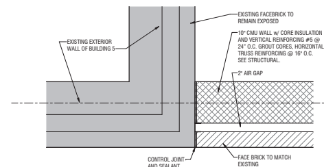
3 PLAN DETAIL AE310 SCALE: 1 1/2" = 1'-0"
