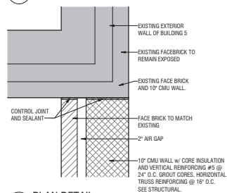
3 PLAN DETAIL AE310 SCALE: 1 1/2" = 1'-0"
