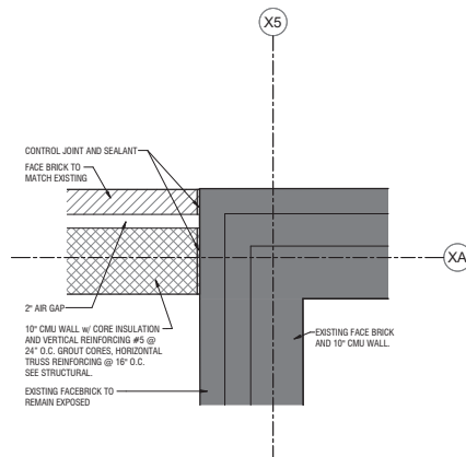
1 PLAN DETAIL AE310 SCALE: 1 1/2" = 1'-0"
