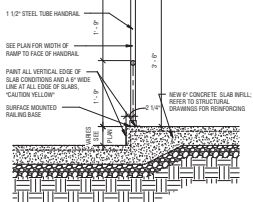
3 HANDRAIL DETAIL SCALE: 3/4\"/>
