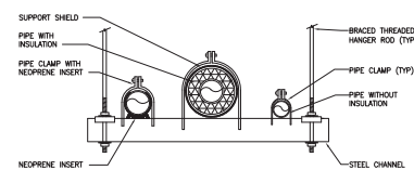
6 TYPICAL TRAPEZE PIPE SUPPORT DETAIL SCALE: NONE
