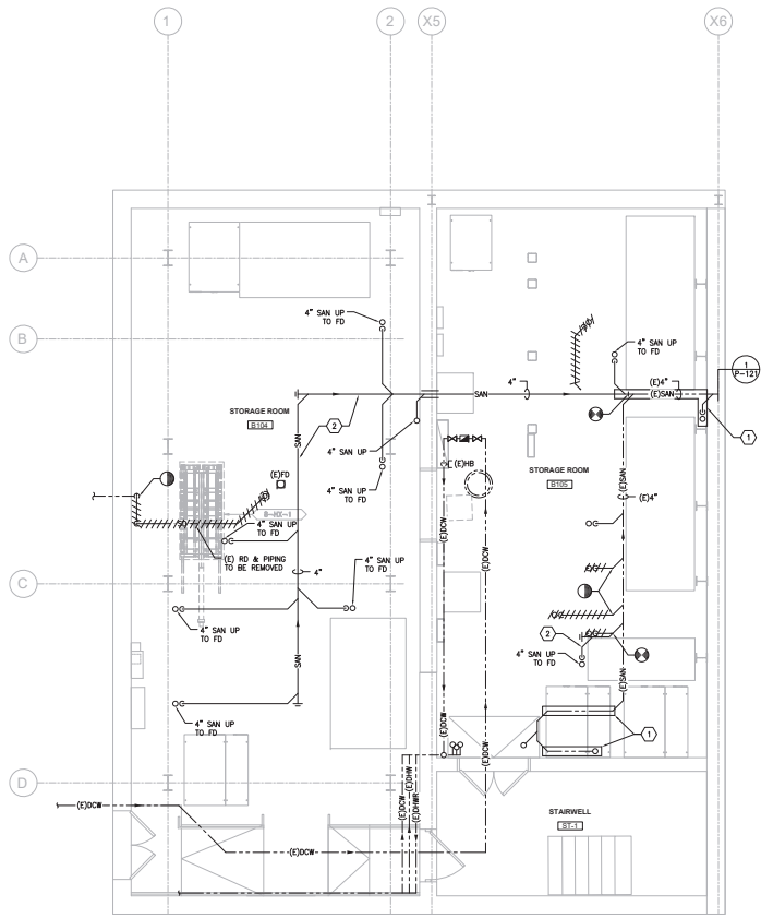
1 PLUMBING PLAN - FIRST LEVEL SCALE: 1/4" = 1'-0"
