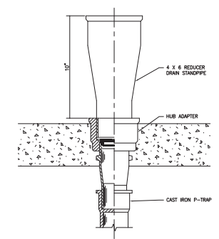
3 HUB DRAIN DETAIL SCALE: NONE
