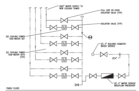
1 SUB-METER DETAIL SCALE: NONE
