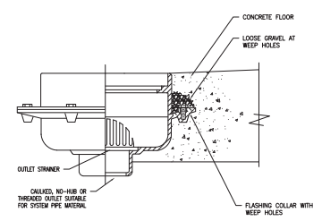
2 TYPE "E" FLOOR DRAIN DETAIL SCALE: NONE
