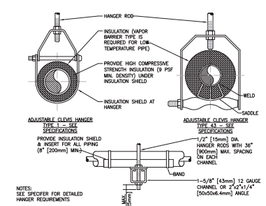
6 TYPICAL TRAPEZE PIPE SUPPORT DETAIL SCALE: NONE
