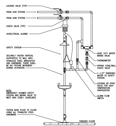
4 EMERGENCY SHOWER DETAIL SCALE: NONE
