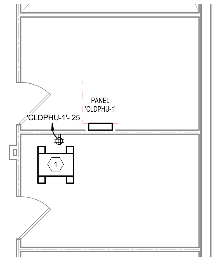
1 HEADEND EQUIPMENT LOCATION - CLC 1H-103 Scale: 1/4" = 1'-0"
