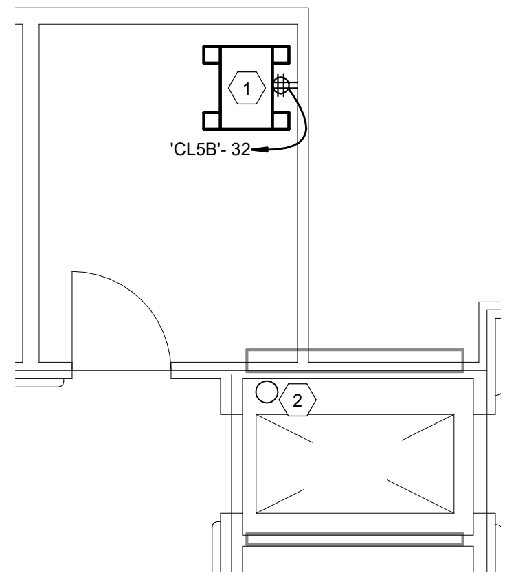
4 HEADEND EQUIPMENT LOCATION - BUILDING 1 FIFTH FLOOR 5B-302C Scale: 1/4" = 1'-0"
