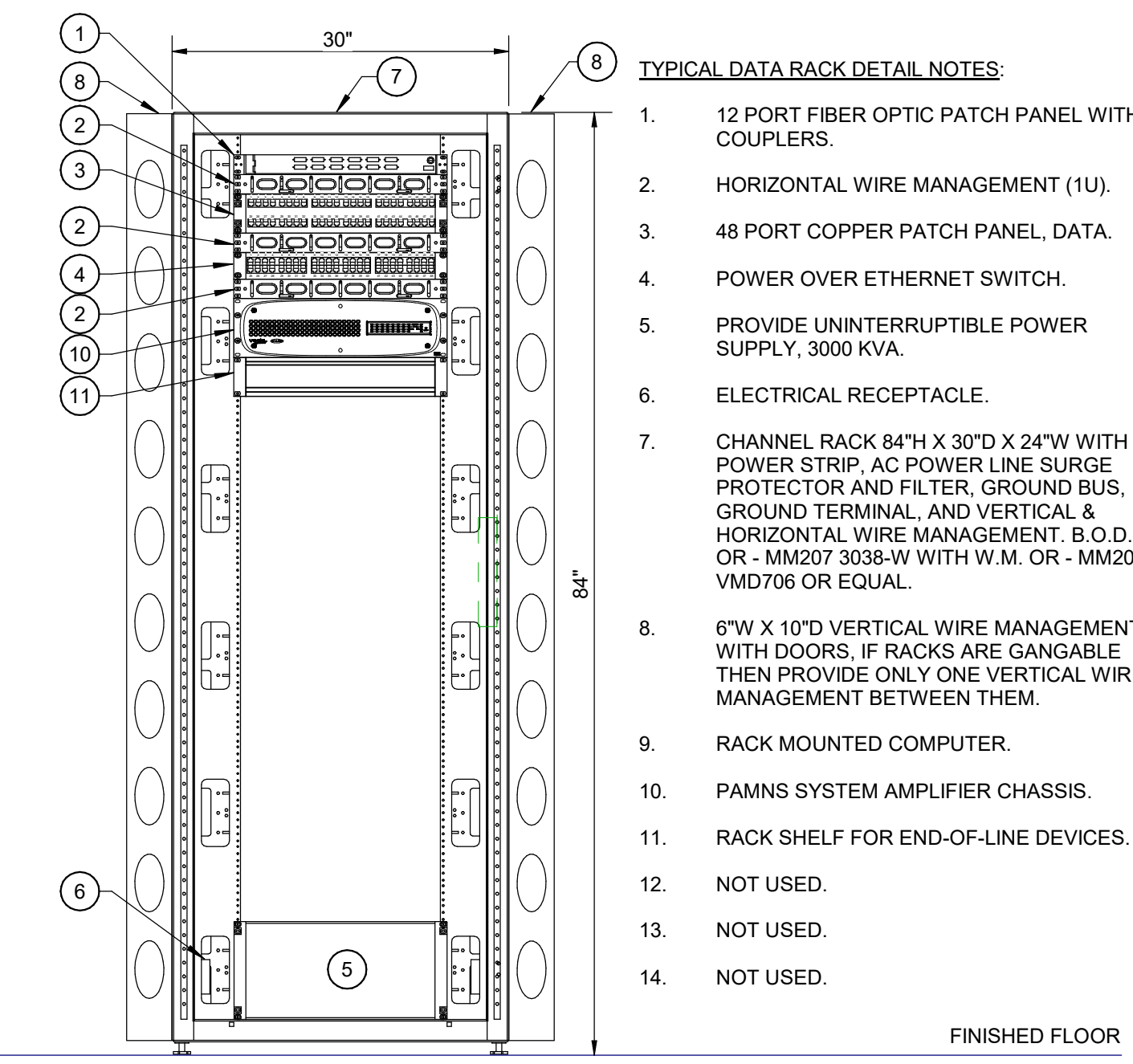
5 PAMNS HEAD END EQUIPMENT RACK TELECOM 1H-103 Scale: No Scale
