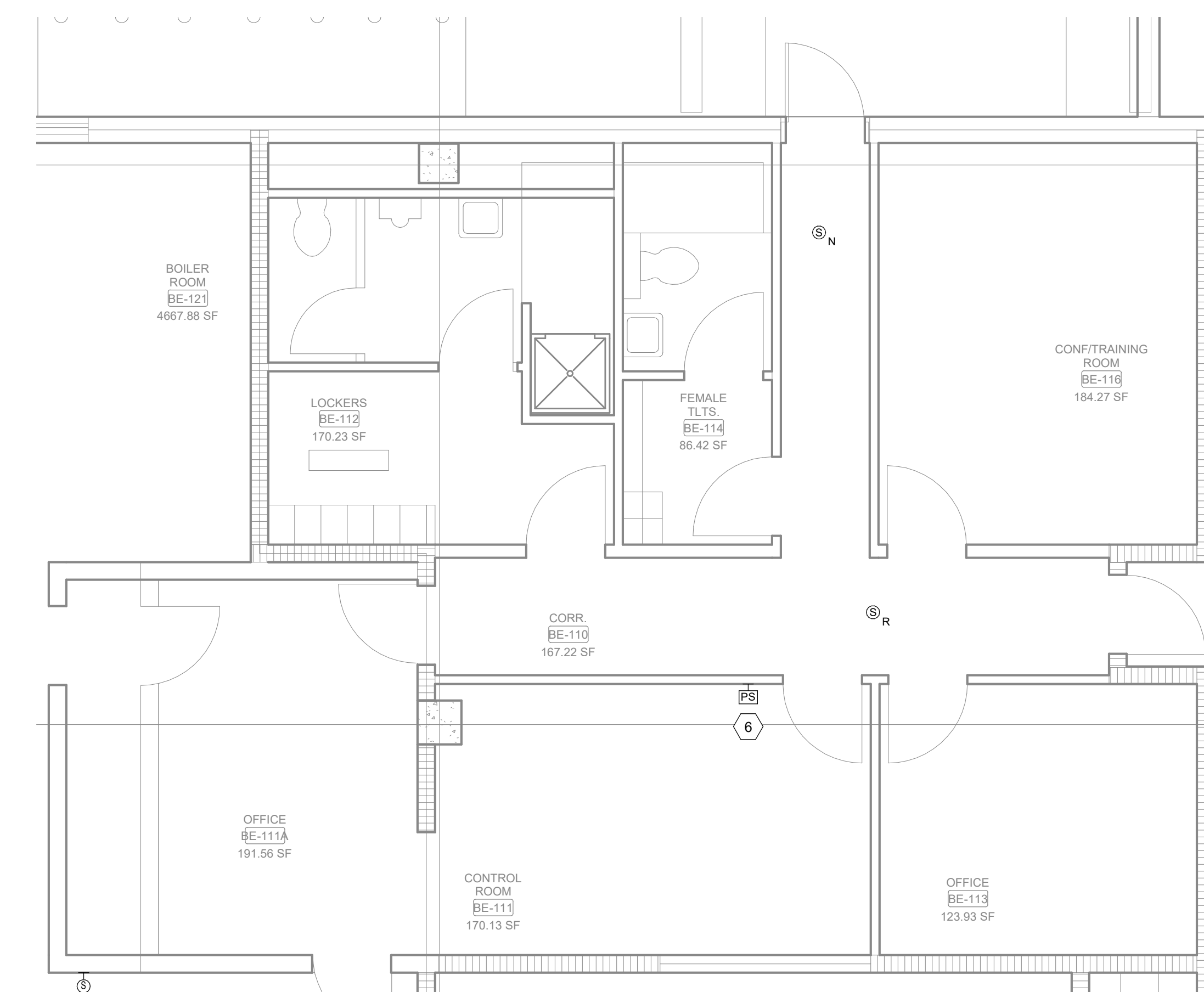
2 BASEMENT ENLARGEMENT - ENERGY CENTER Scale: 1/4" = 1'-0"
