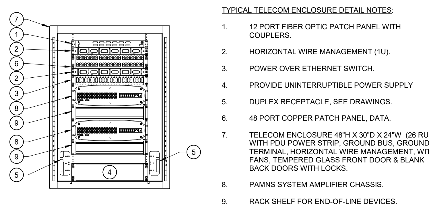
PAMNS HEAD END EQUIPMENT CABINET TELECOM 2B-302C TELECOM 5B-302C TELECOM 8A-302C Scale: No Scale
