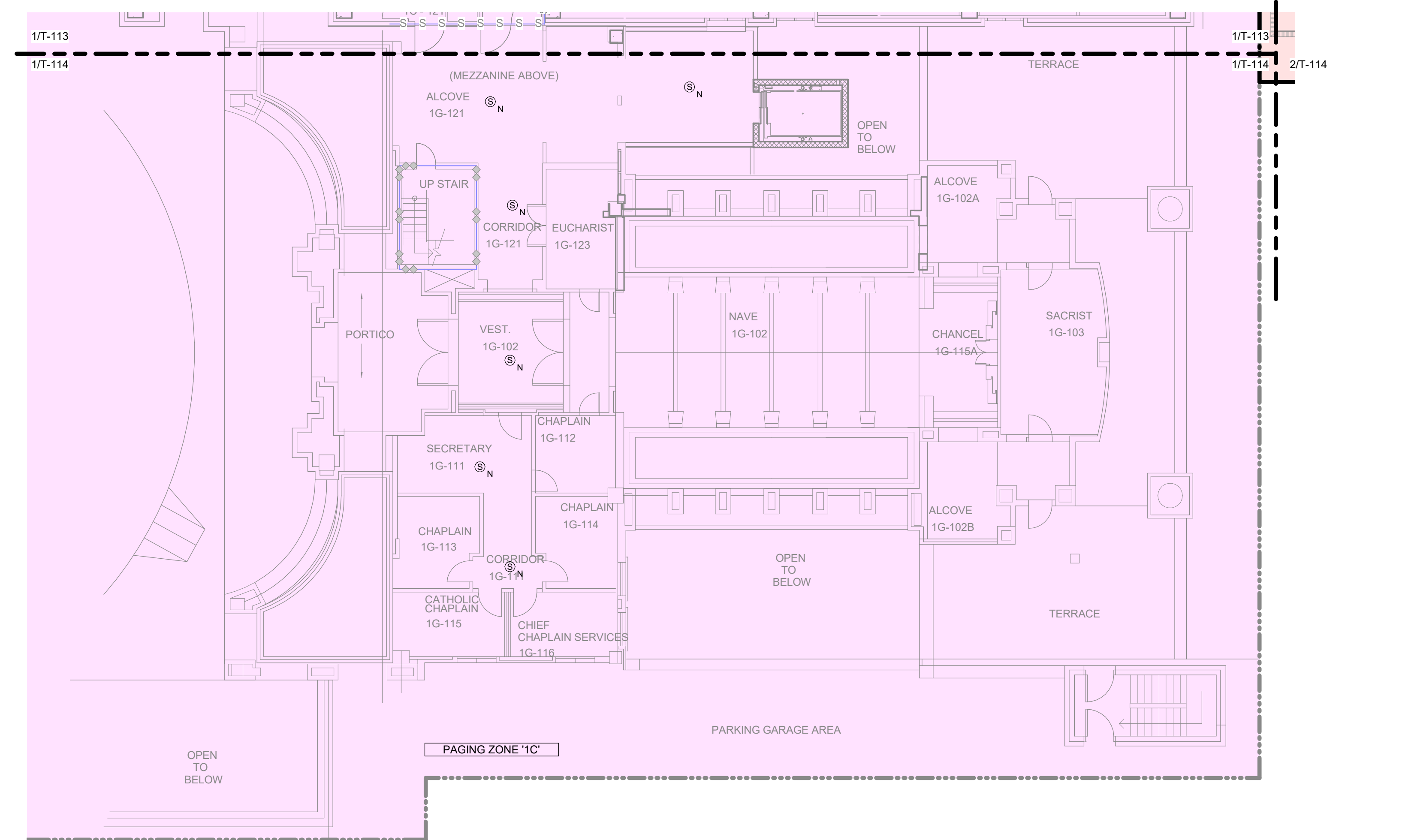
1 FIRST FLOOR E PAMNS Scale: 3/32" = 1'-0"
