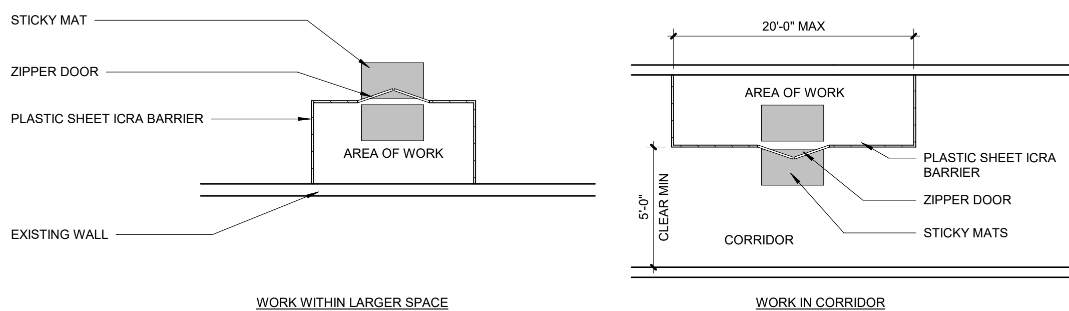
5 TYPICAL ICRA CONDITIONS Scale: 1/4" = 1'-0"
