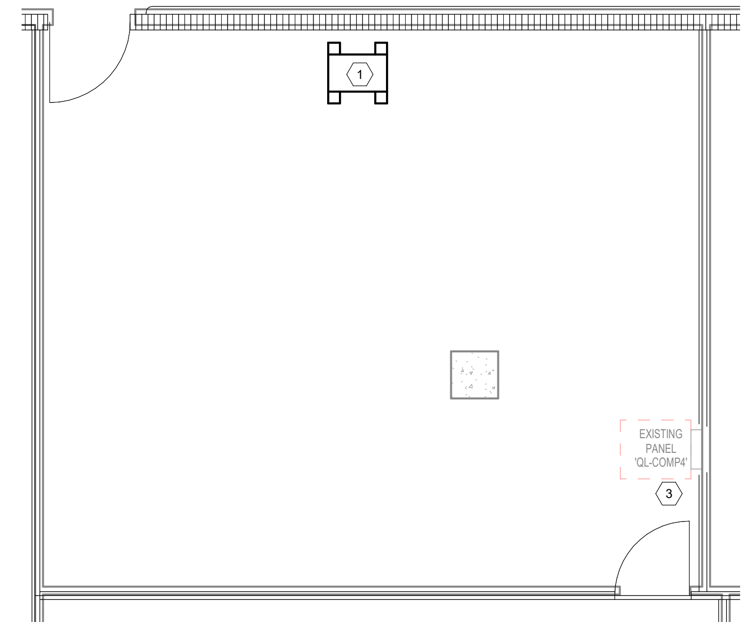
2 HEADEND EQUIPMENT LOCATION - BLDG 1 BASEMENT BC-202 Scale: 1/4" = 1'-0"
