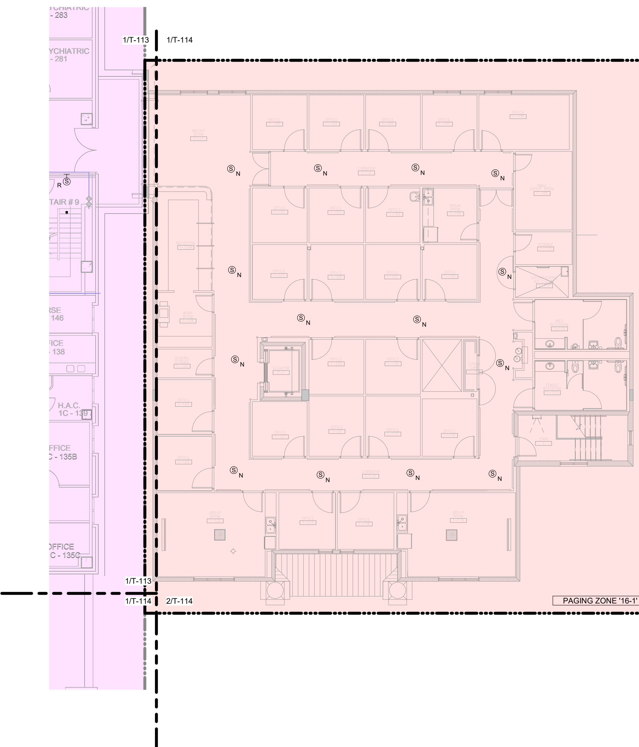
2 BUILDING 16 FIRST FLOOR SE PAMNS Scale: 3/32" = 1'-0"
