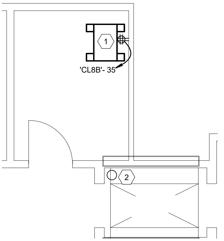
5 HEADEND EQUIPMENT LOCATION - BUILDING 1 EIGHTH FLOOR 8A-302C Scale: 1/4" = 1'-0"
