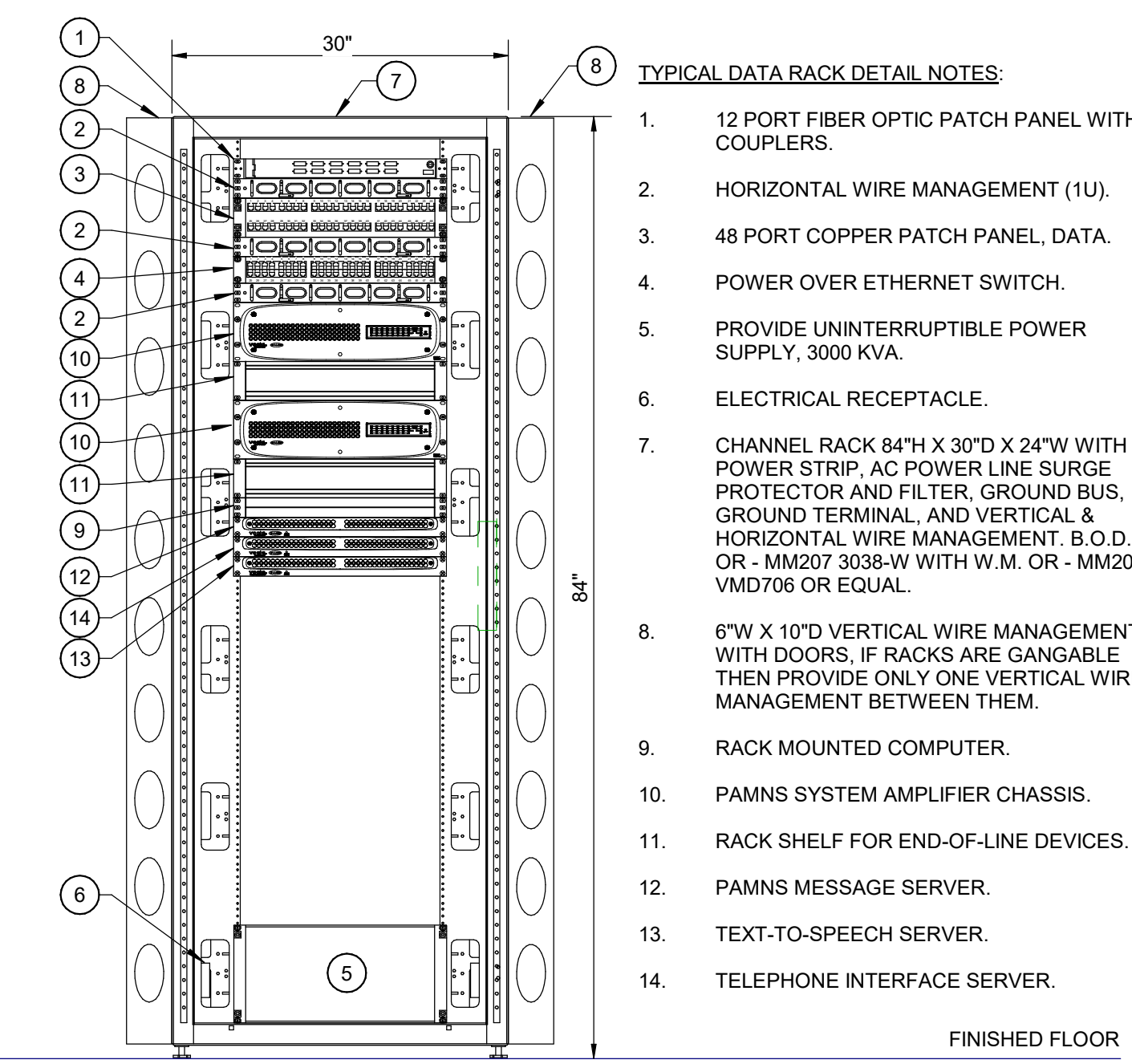
4 PAMNS HEAD END EQUIPMENT RACK EQUIP. TECH WORK ROOM BC-202 Scale: No Scale
