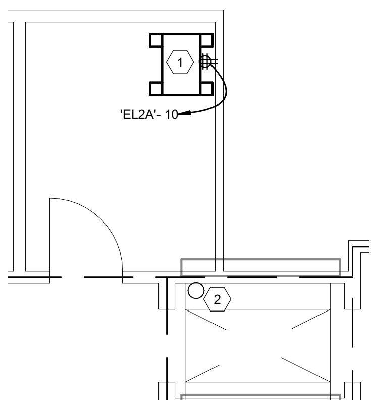
3 HEADEND EQUIPMENT LOCATION - BUILDING 1 SECOND FLOOR 2B-302C Scale: 1/4" = 1'-0"
