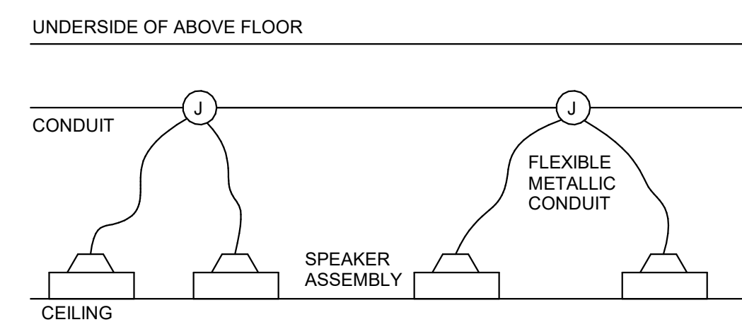
3 SPEAKER CABLING DETAIL Scale: No Scale
