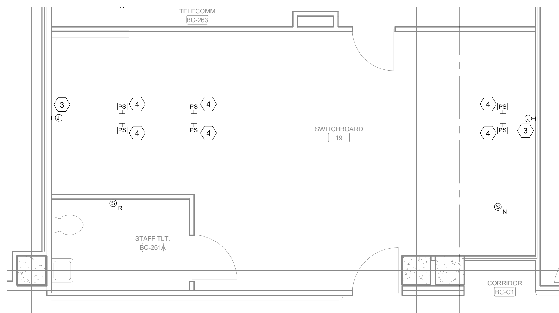
3 BASEMENT ENLARGEMENT - CALL CENTER Scale: 1/4" = 1'-0"
