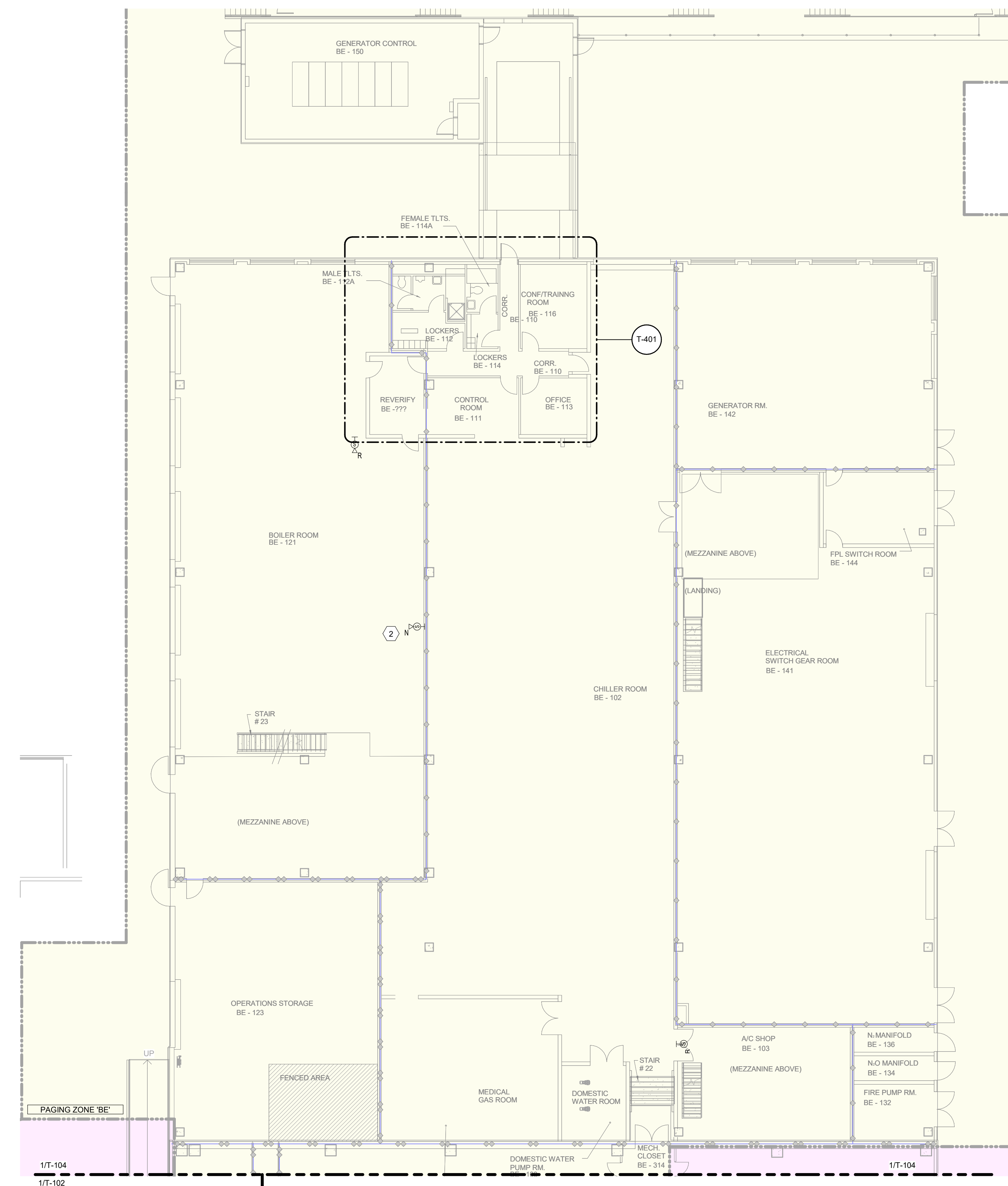
1 BASEMENT FLOOR PAMNS - ENERGY CENTER Scale: 3/32" = 1'-0"
