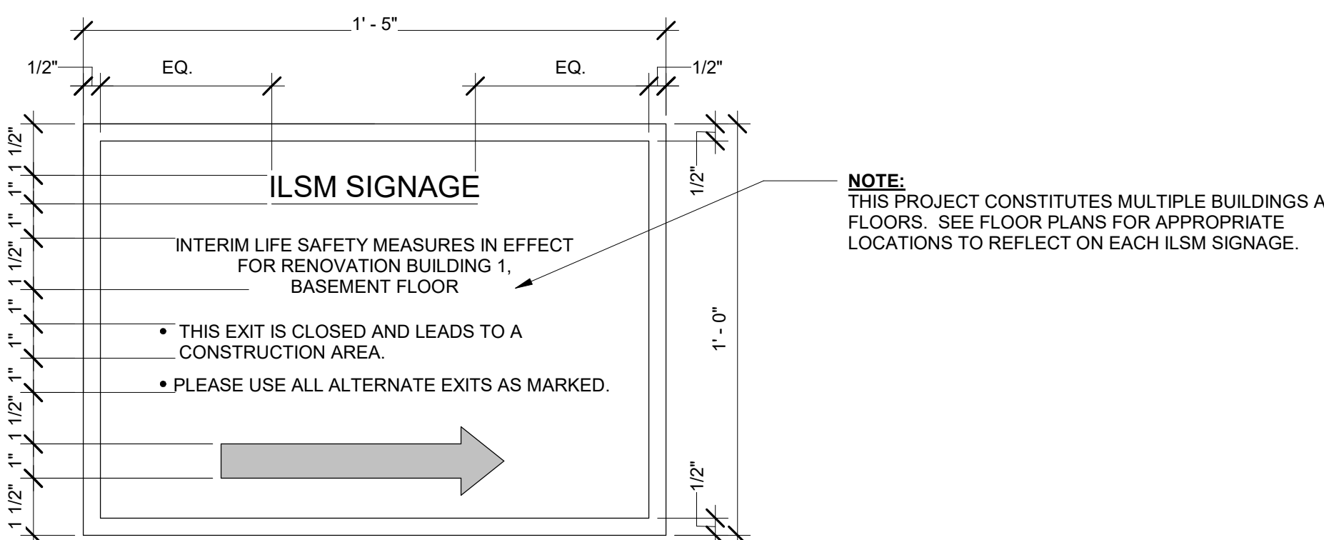
4 ILSM CONSTRUCTION EGRESS SIGNAGE Scale: 3" = 1'-0"
