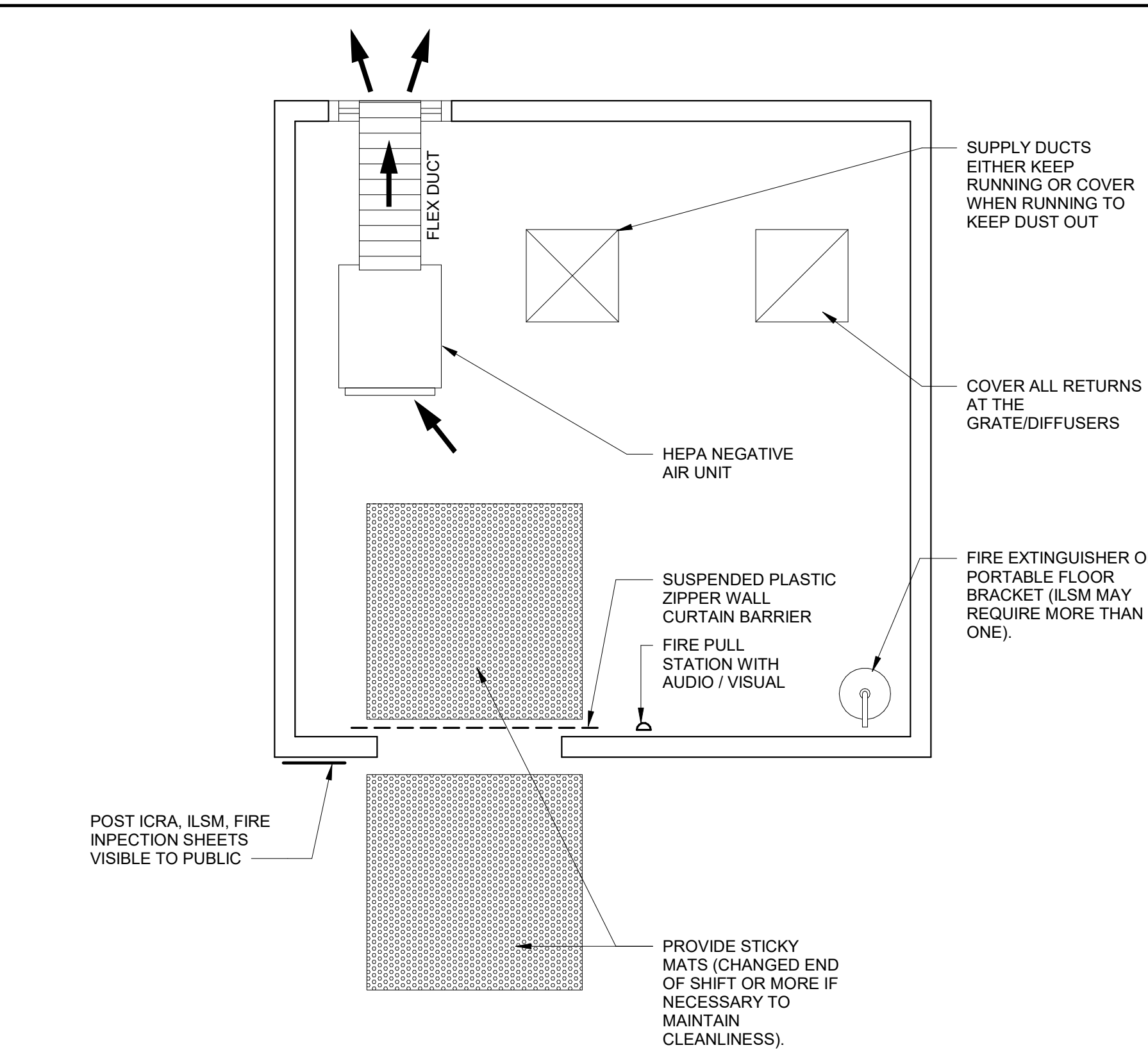
1 TYPICAL CONSTRUCTION PLAN LAYOUT Scale: 1/2" = 1'-0"
