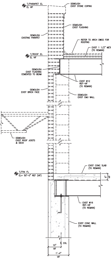
2 WALL DEMOLITION DETAIL SCALE: 1"=1'-0"
