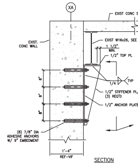
10 BEAM SUPPORT SCALE: 1" = 1'-0"
