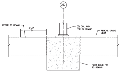
7 FOUNDATION DEMOLITION ELEVATION SCALE: 3/4"=1'-0"
