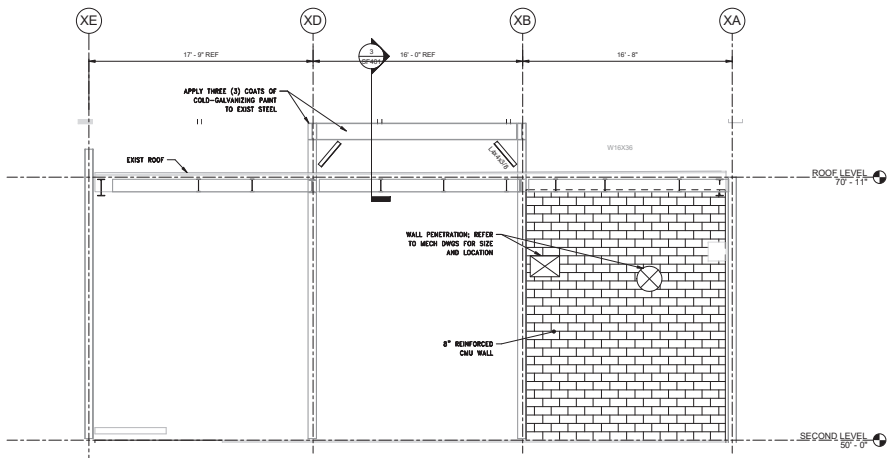
1 ELEVATION ALONG COLUMN LINE X5 SCALE: 1/4" = 1'-0"
