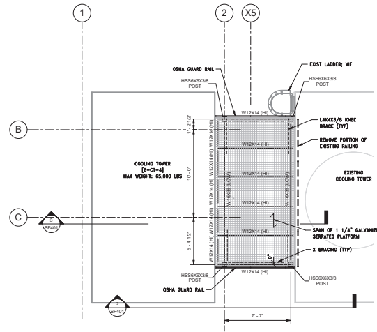
1 FRAMING PLAN - TOP OF COOLING TOWER PLATFORM SCALE: 1/4" = 1'-0"
