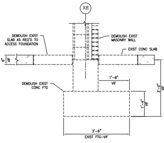
6 FOUNDATION ENLARGEMENT DETAIL SCALE: 3/4"=1'-0" REF: SFT01
