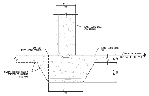
5 FOUNDATION DEMOLITION DETAIL SCALE: 1"=1'-0"
