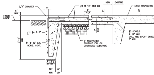
1 EXTERIOR EQUIPMENT FOUNDATION DETAIL SCALE: N.T.S.
