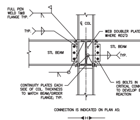
9 TYPICAL MOMENT CONNECTION AT COLUMN DETAIL SCALE: 3/4" = 1'-0"
