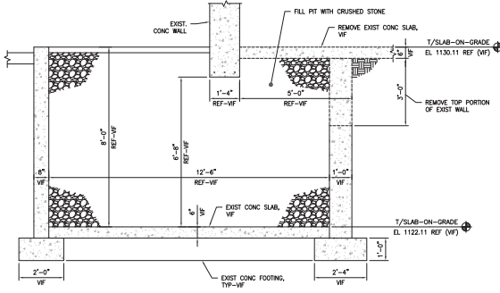
4 FOUNDATION DEMOLITION SECTION SCALE: 1/2"=1'-0"
