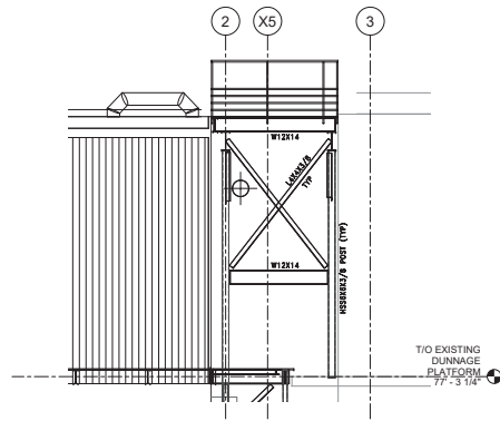
2 COOLING TOWER PLATFORM ELEVATION SCALE: 1/4" = 1'-0"
