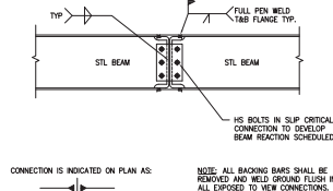
3 TYPICAL BEAM TO BEAM MOMENT CONNECTION DETAIL SCALE: 3/4" = 1'-0" REF: DWG. SF131, SF132
