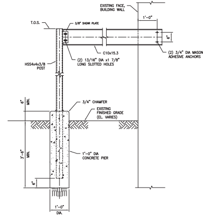
3 PIPE SUPPORT DETAIL SCALE: 3/4" = 1'-0"
