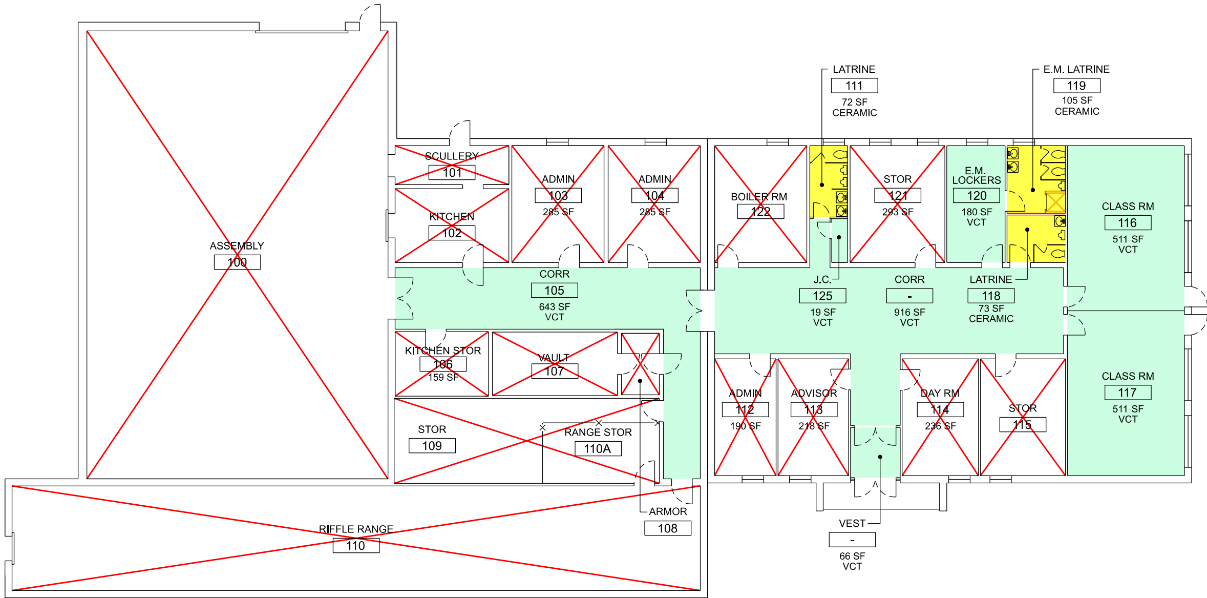
1 USARC - MAIN FLOOR CUSTODIAL SERVICE PLAN SCALE: 1/16"=1'-0"
