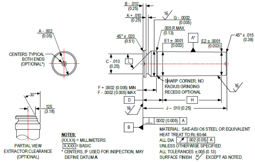
FIGURE II BELT-BREECHING CENTERFIRE RIFLE HEADSPACE GAUGES
